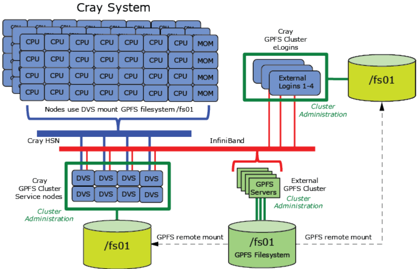
Figure 2. Cluster mount configuration diagram displaying connections between nodes and clusters.
