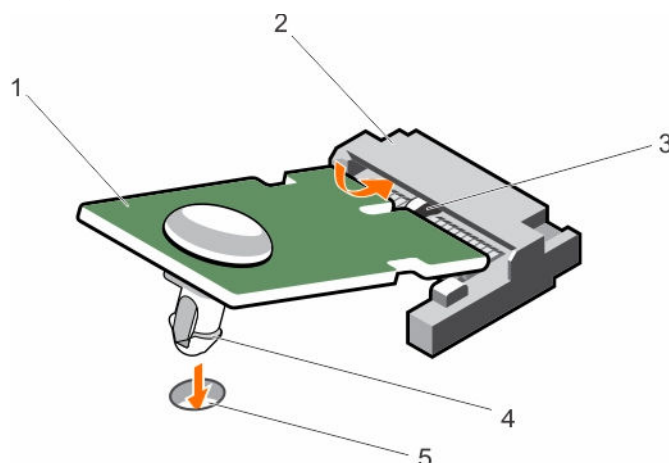
Figure 62. Installation du TPM
