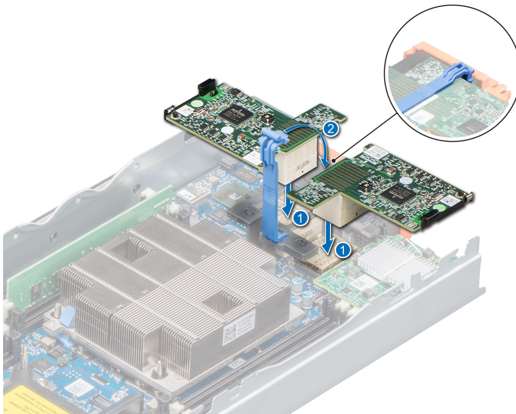
Figure 43. Installation de la carte mezzanine
