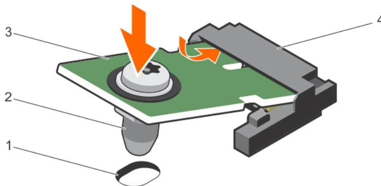
Figure 95. Installation du TPM
