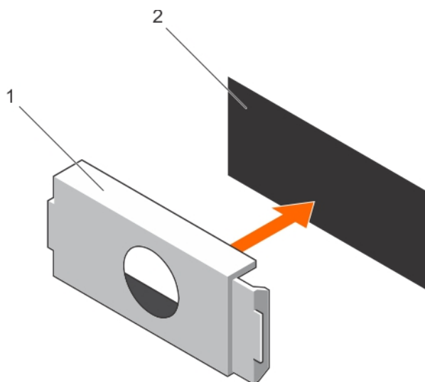
Figure 39. Installation du cache PSU
