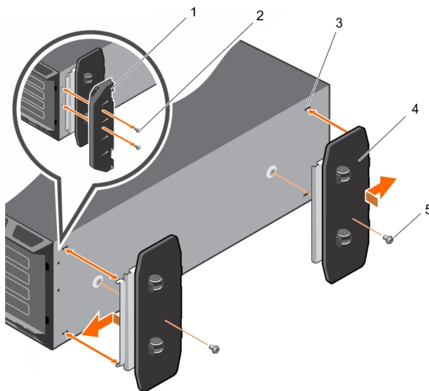
Figure 19. Installation des roulettes
