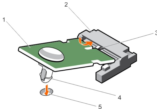
Figure 67. Installation du TPM
