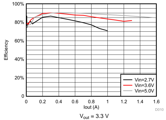
Figure 66. DCDC4 Efficiency
