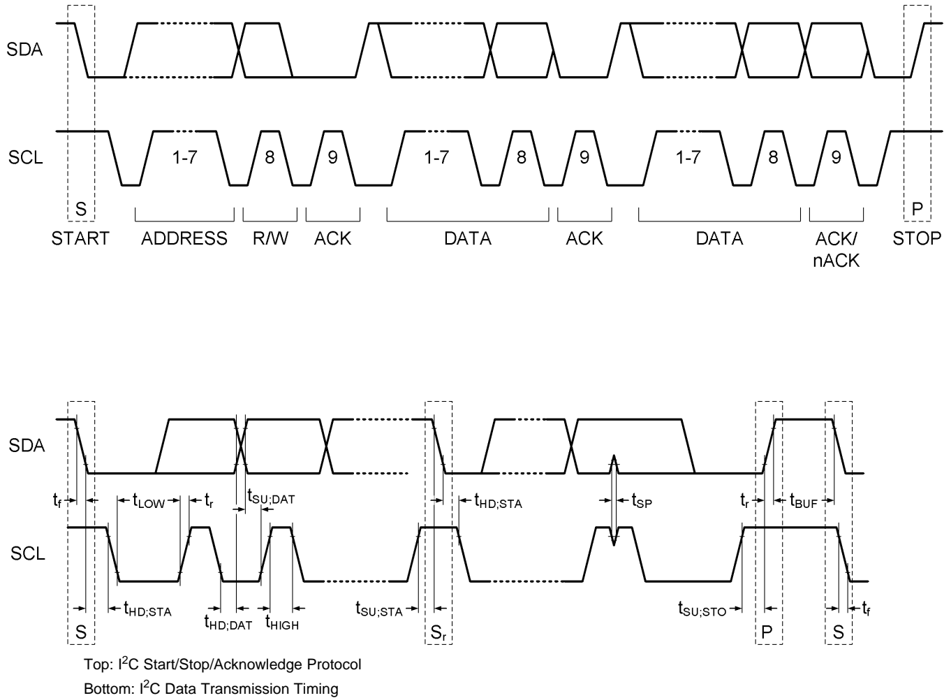
Figure 33. I 2 C Protocol and Transmission Timing
