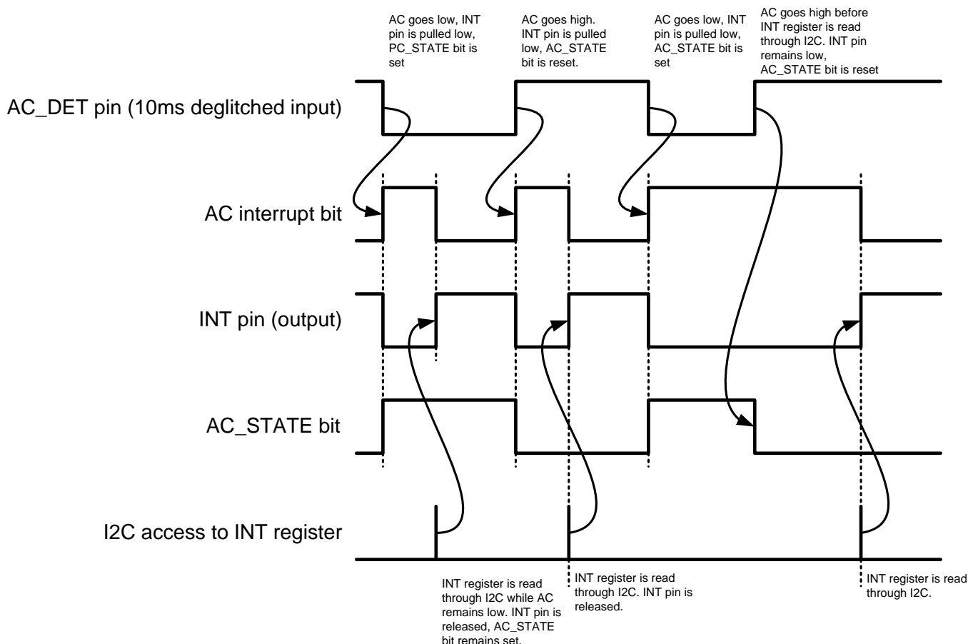
Figure 30. AC_STATE Pin
