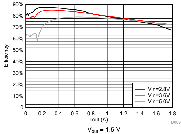
Figure 65. DCDC3 Efficiency
