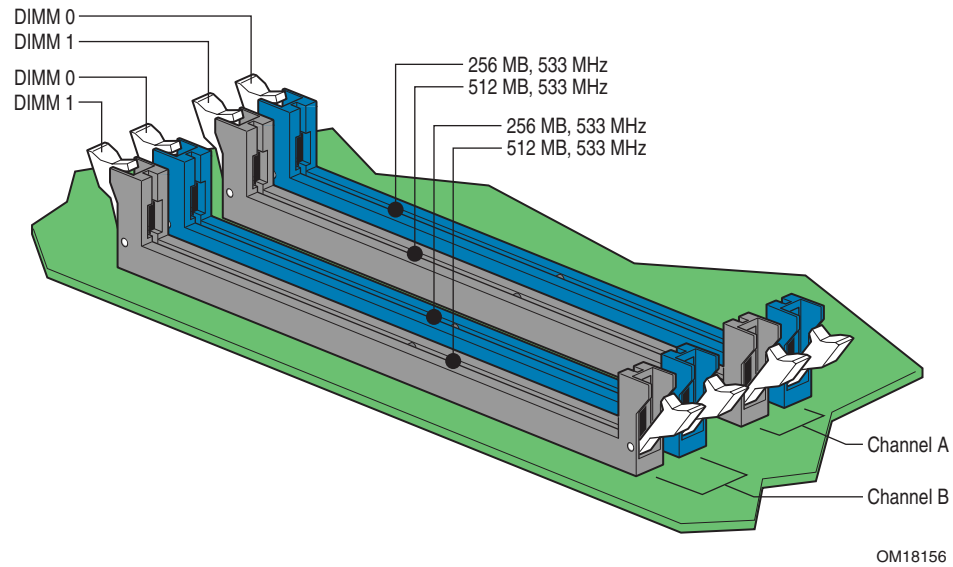
Figure 17. Dual Channel Memory Configuration Example 2
