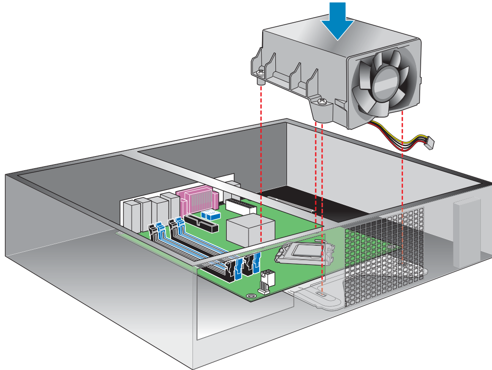
Figure 12. Position the Thermal Module Over the Mounting Holes
