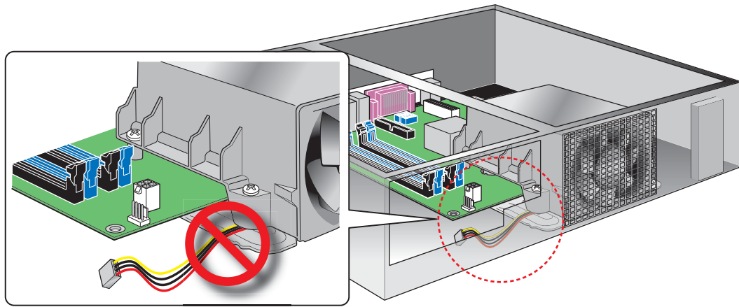
Figure 13. Use Care Routing the Thermal Module Fan Cable
