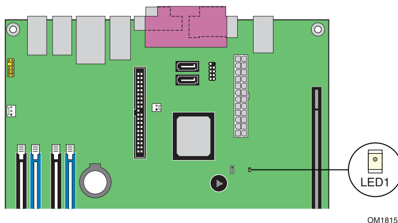
Figure 3. Location of Standby Power Indicator
