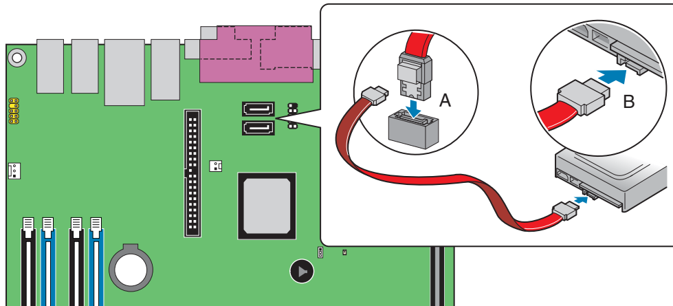
Figure 21. Connecting the Serial ATA Cable
