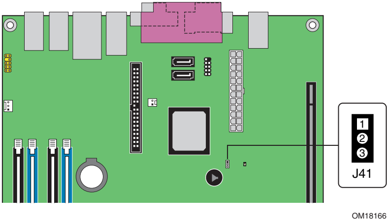
Figure 26. Location of the BIOS Configuration Jumper Block
