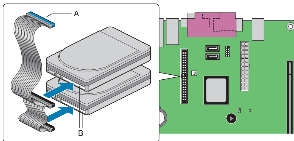
Figure 20. Connecting the IDE Cable
