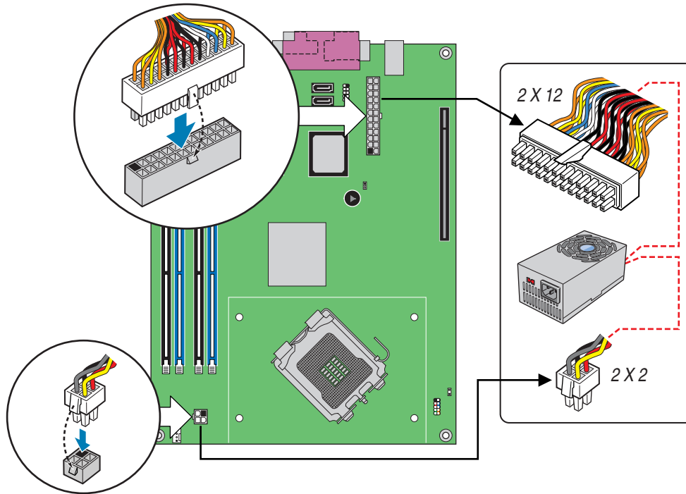
Figure 25. Connecting Power Supply Cables
