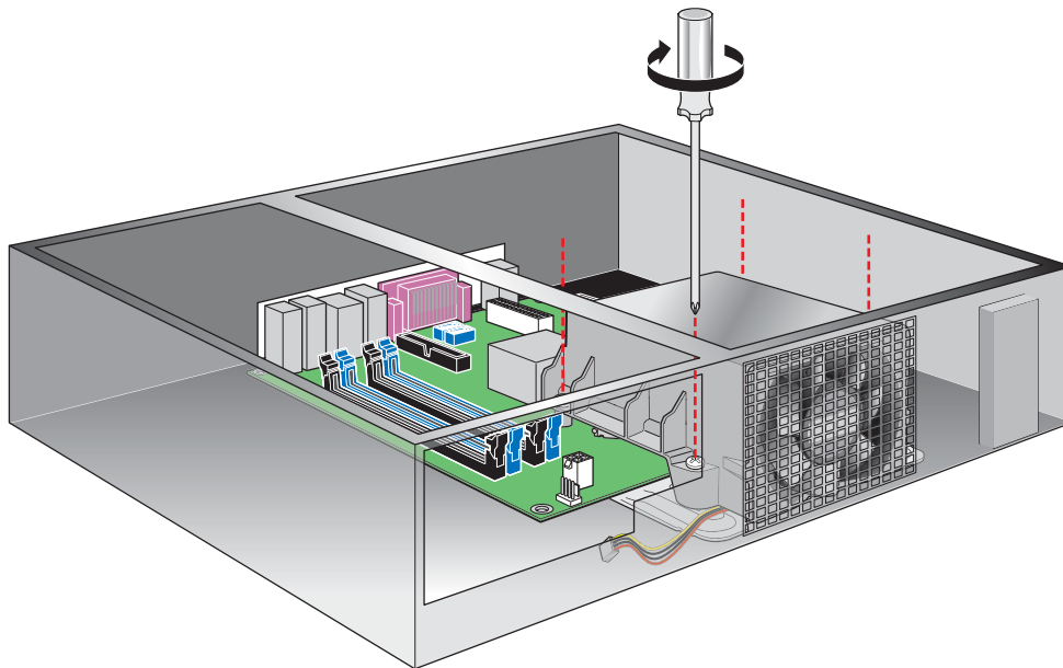
Figure 14. Secure the Thermal Module
