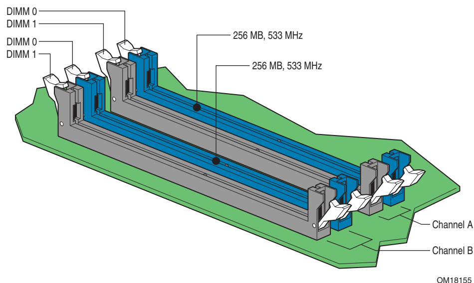
Figure 16. Dual Channel Memory Configuration Example 1
