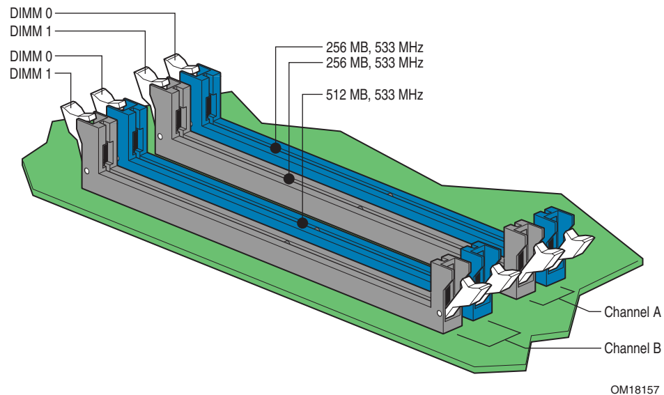
Figure 18. Dual Channel Memory Configuration Example 3
