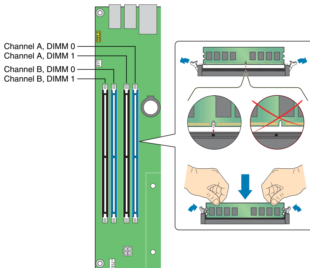
Figure 19. Installing a DIMM
