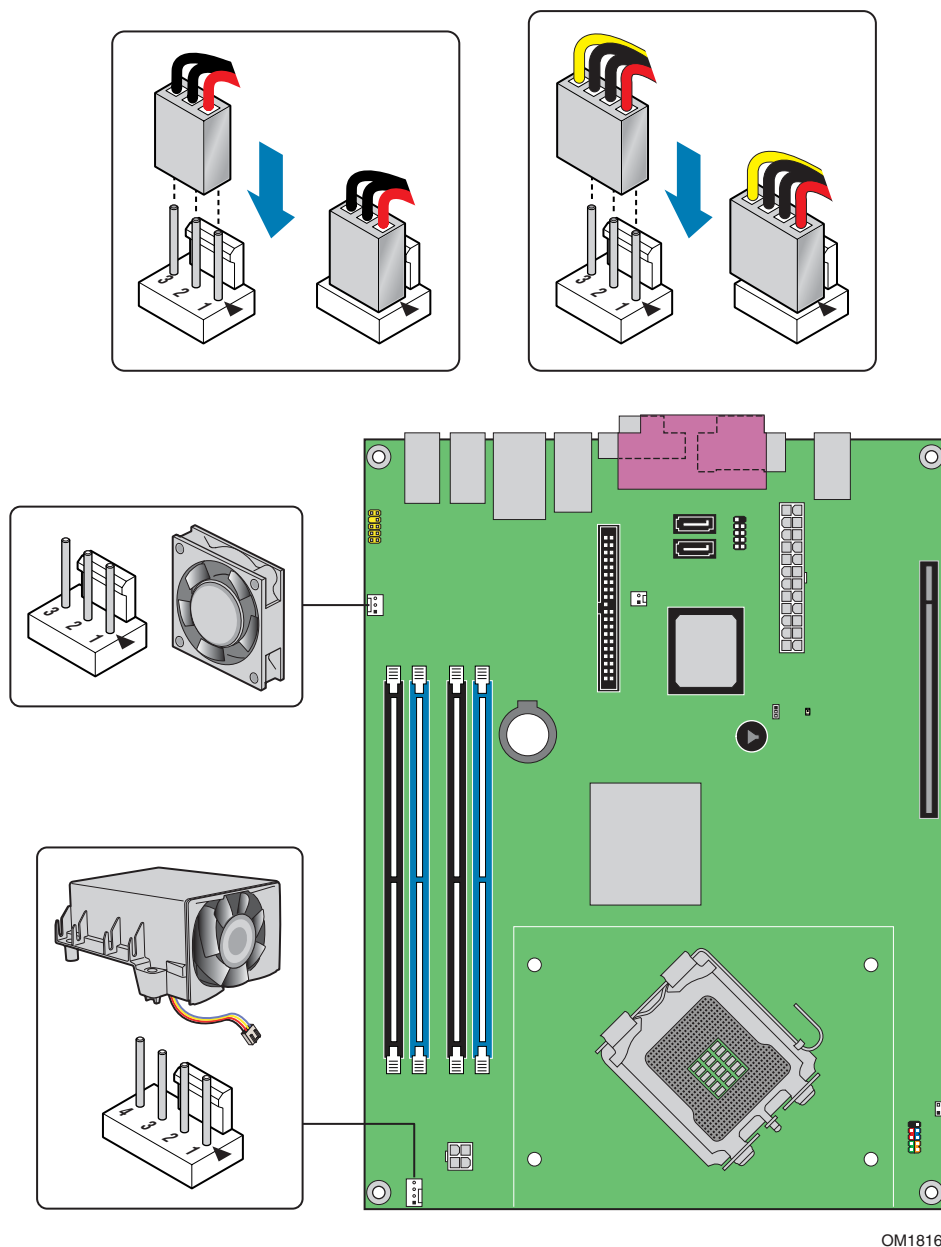
Figure 24. Location of Fan Headers
