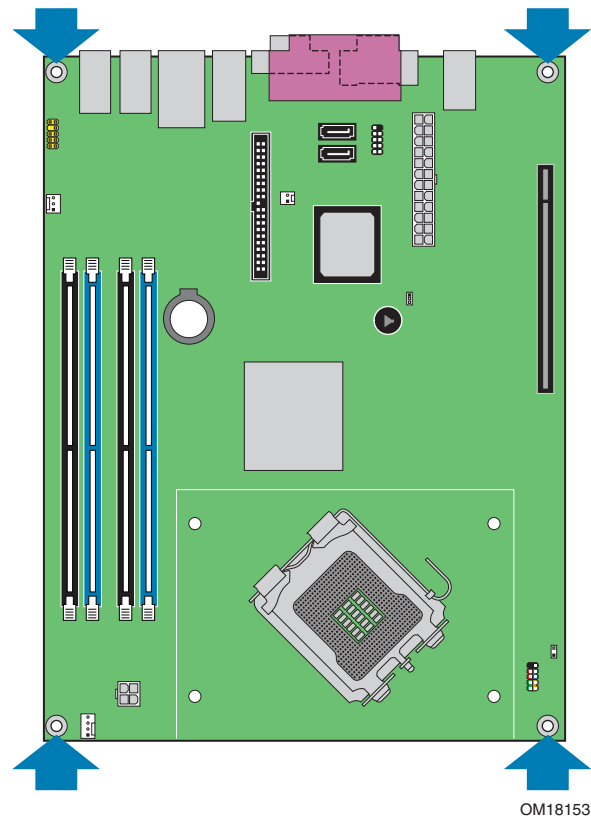
Figure 5. Desktop Board D945GRW Mounting Screw Hole Locations
