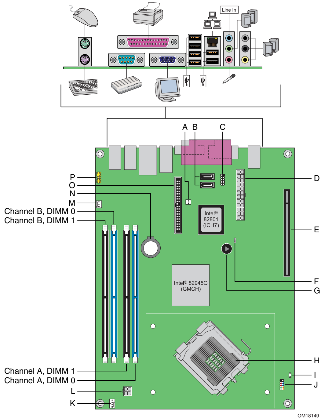
Figure 1. Desktop Board D945GRW Components
