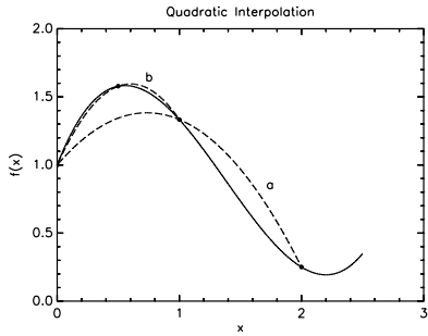
Figure 10.2 Quadratic interpolation follows the curves better if the curvature doesn't change sign.
