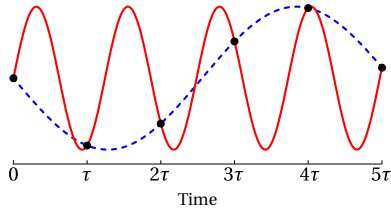
Figure 13.4 The sine of a negative frequency (dashed) and its aliased positive frequency (solid). In our wagon wheel example, these would be \omega_{-1} and \omega_0 . The dots indicate times at which the signal is sampled. There are infinitely many other frequencies that also cross these sampled points, as specified by Eq. (13.5).
