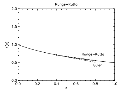
Figure 9.1 Runge-Kutta anticipates curving and beats Euler.
