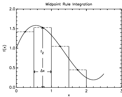
Figure 8.2 The midpoint rule works OK if the function is nearly straight across each interval.
