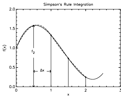
Figure 8.3 Fitting parabolas (Simpson's Rule) works better.
