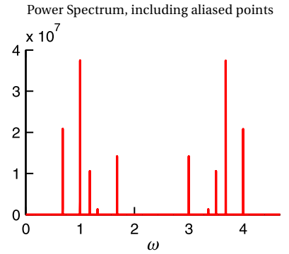
Figure 13.6 The fft of the same signal as Fig. 13.5 sampled with a slower rate ( \tau is about 4 times bigger) for the same amount of time. The “real” signal peaks are at \omega = 1, 3, 3.5, 4, 6 ; the rest of the peaks are aliased negative frequencies.
