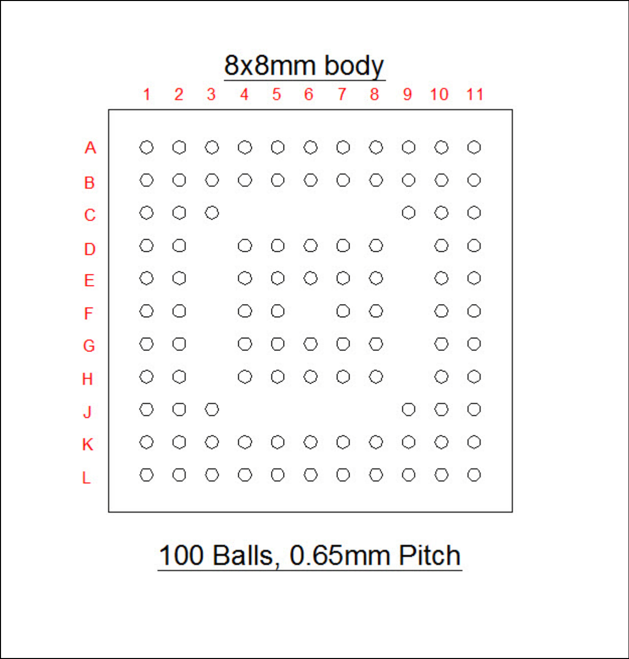
FIGURE 2-2: SCH3226 PIN DIAGRAM
