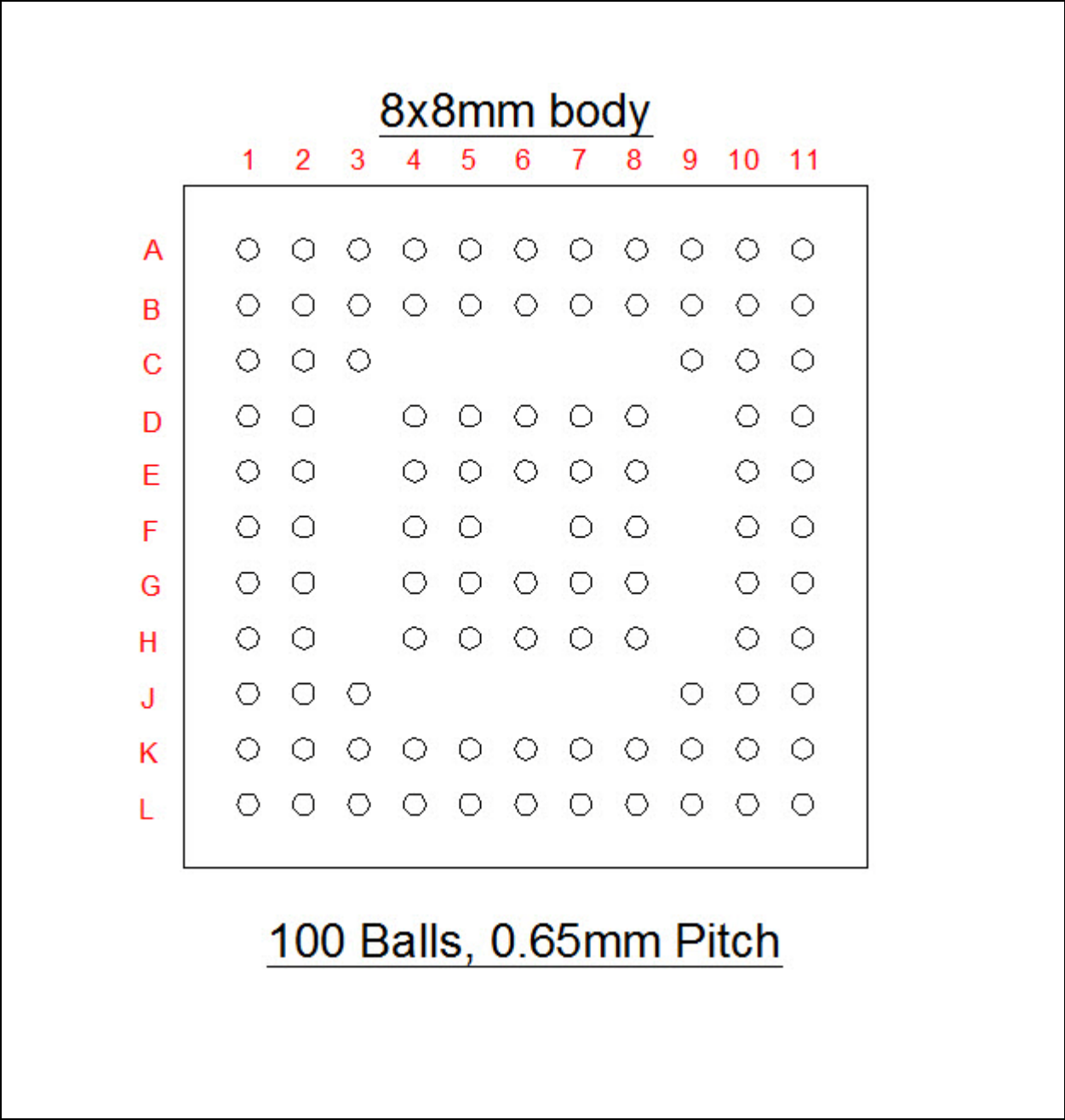
FIGURE 2-3: SCH3224 PIN DIAGRAM
