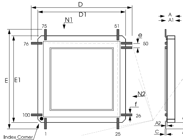
Figure 3. 100-Pin Ceramic Quad Flat Pack (MQFP)
