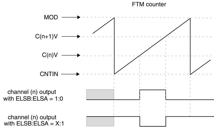
Figure 41-25. Channel (n) output if (CNTIN < C(n)V < MOD) and (CNTIN < C(n+1)V < MOD) and (C(n)V < C(n+1)V)
