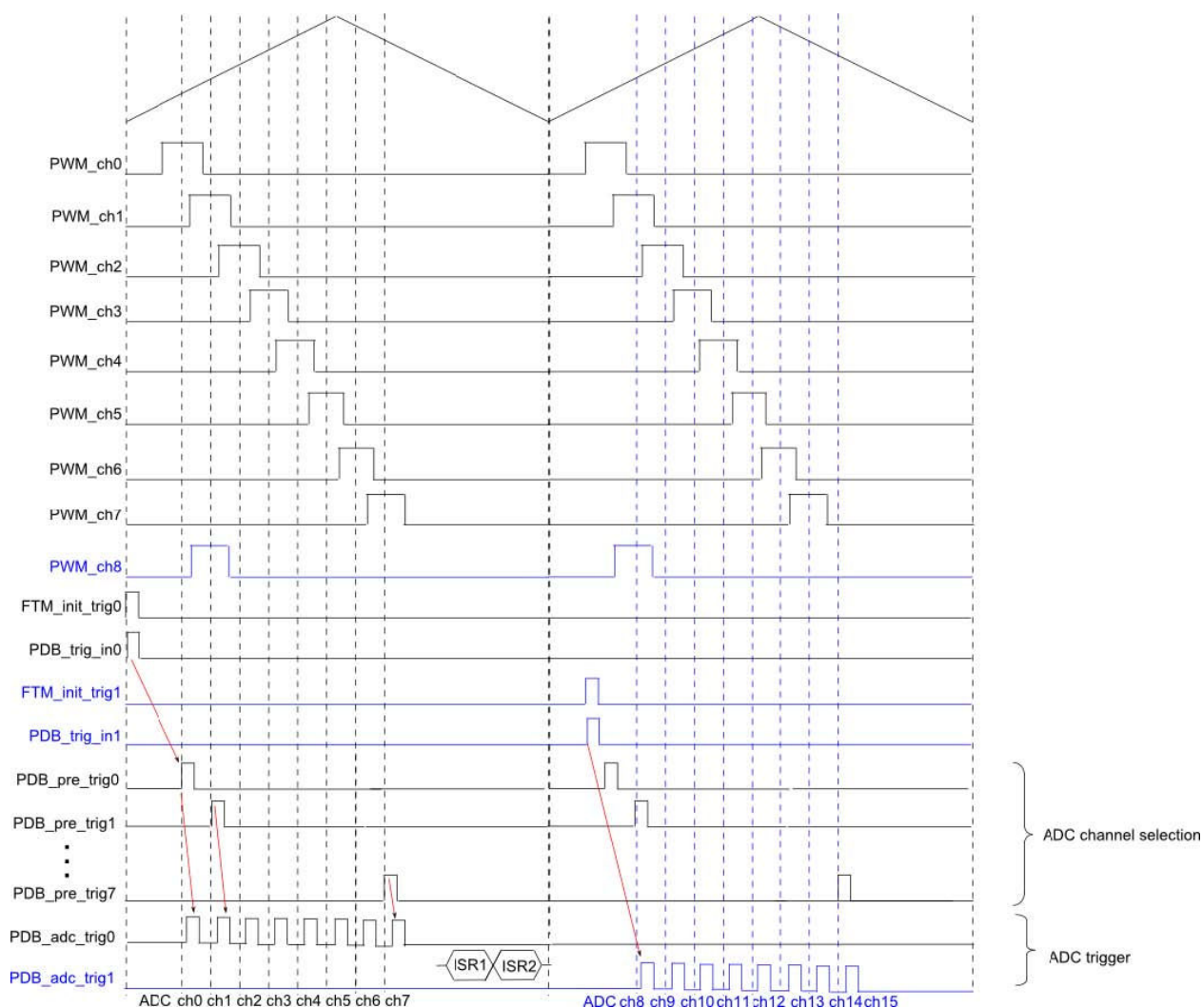
Figure 37-6. PWM Load Diagnosis – ADC Trigger Concept 2 (Timing)
