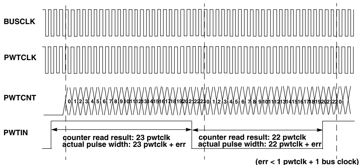
Figure 43-8. Example at PWTCLK is bus clock divided by 1
