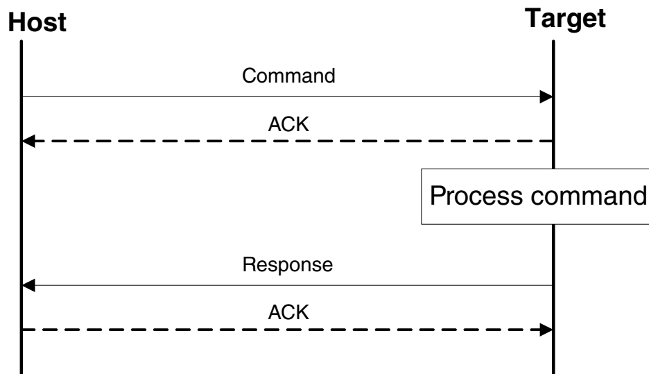
Figure 23-3. Command with No Data Phase
