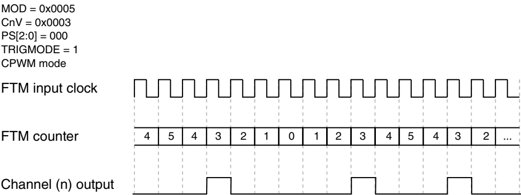
Figure 41-78. Example of trigger generation in the output channel for up-down counting mode
