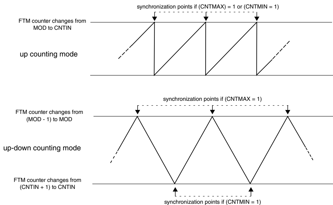
Figure 41-45. Synchronization Points
