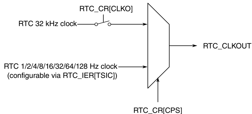
Figure 45-1. RTC_CLKOUT generation
