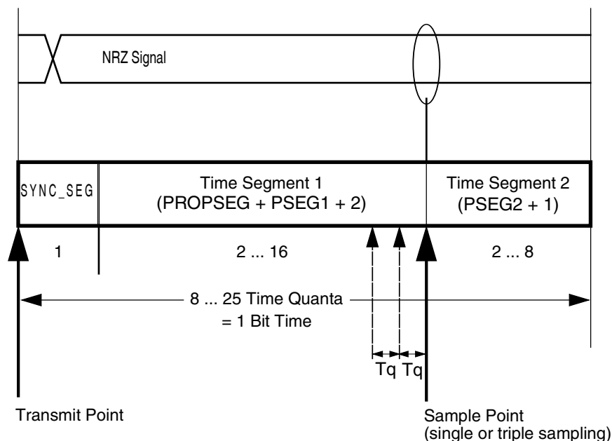
Figure 50-3. Segments within the bit time (example using CAN_CTRL1 bit timing variables for Classical CAN format)
