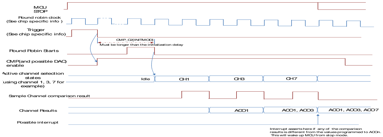
Figure 38-16. Trigger mode
