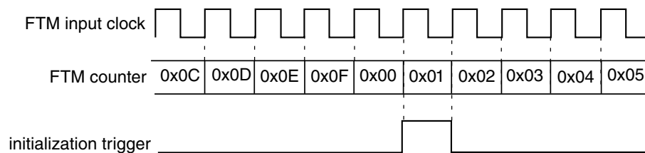
Figure 41-79. Initialization trigger is generated when the FTM counting achieves the CNTIN register value and ITRIGR = 0
