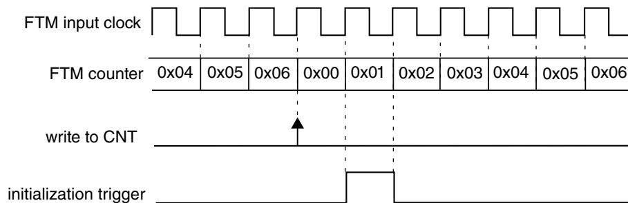
Figure 41-80. Initialization trigger is generated when there is a write to CNT register
