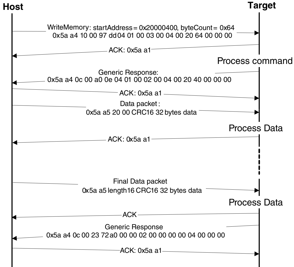
Figure 23-14. Protocol Sequence for WriteMemory Command
