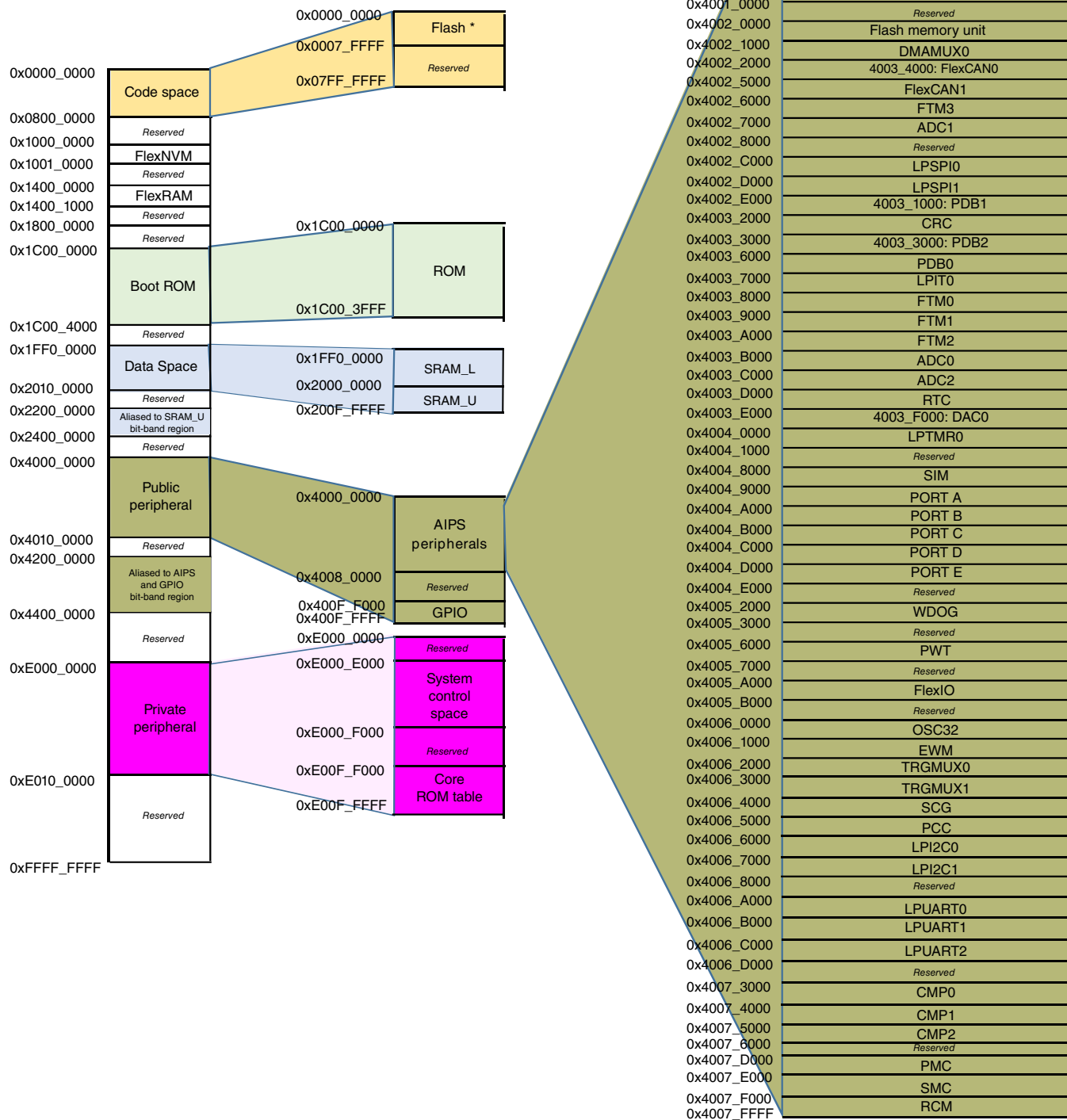
Figure 13-1. Memory map
