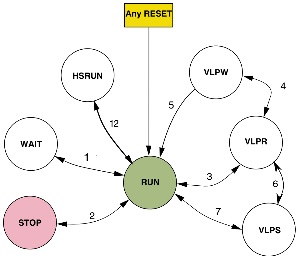
Figure 26-1. Power mode state diagram
