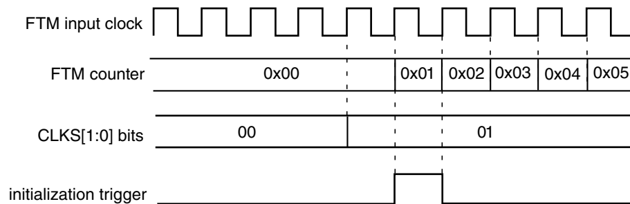
Figure 41-82. Initialization trigger is generated if (CNT = CNTIN), (CLKS[1:0] = 0:0), and a value different from zero is written to CLKS[1:0] bits
