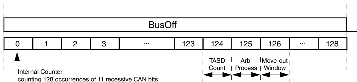
Figure 50-6. Arbitration at the end of bus off and move-out time windows
