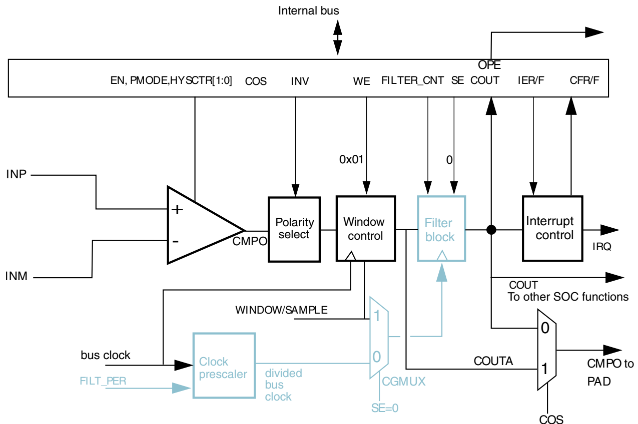
Figure 38-11. Windowed mode
