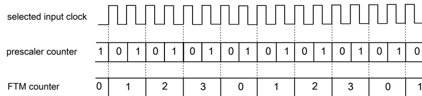
Figure 41-3. Example of the prescaler counter
