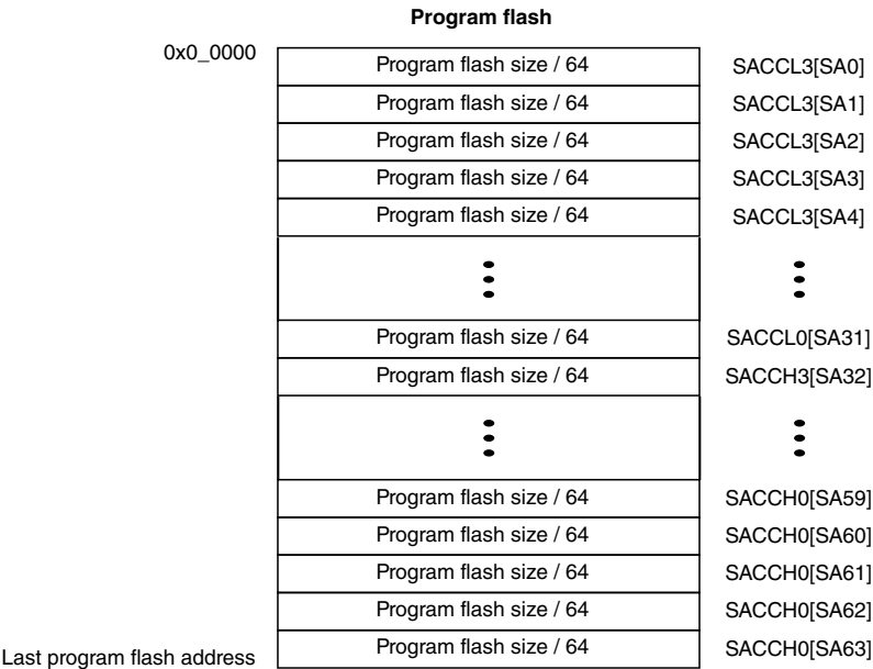
Figure 17-6. Program flash supervisor access control
