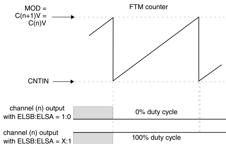
Figure 41-33. Channel (n) output if (C(n)V = C(n+1)V = \text{MOD})
