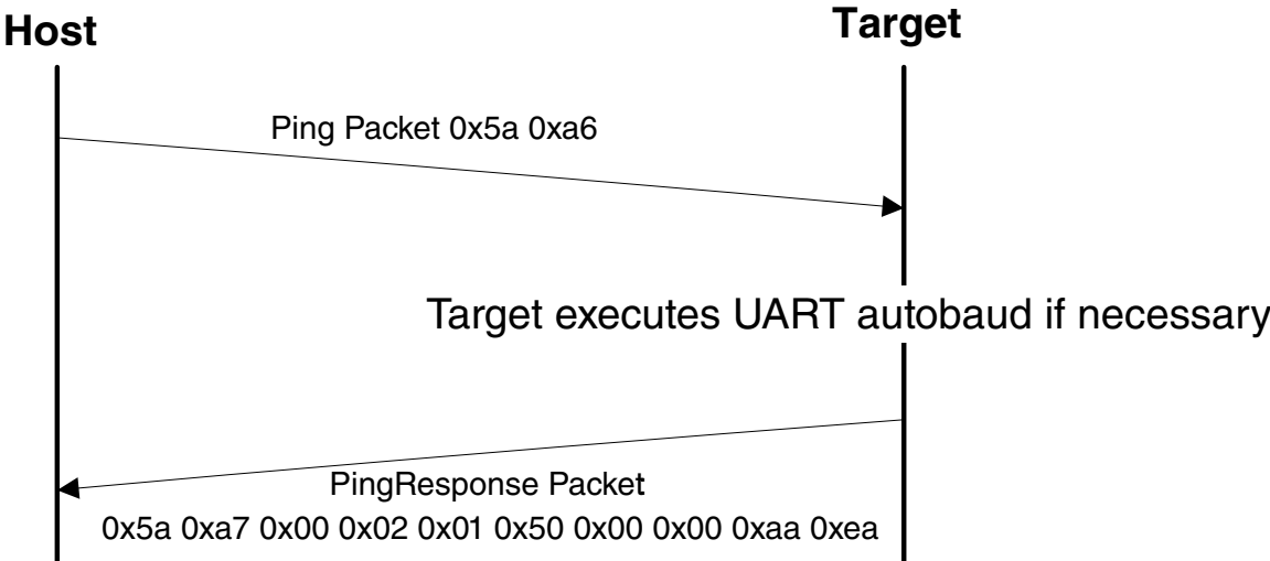
Figure 23-6. Ping Packet Protocol Sequence
