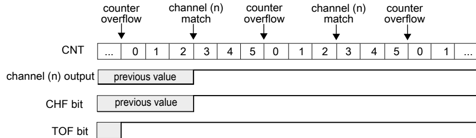
Figure 41-17. Example of the Output Compare mode when the match sets the channel output
