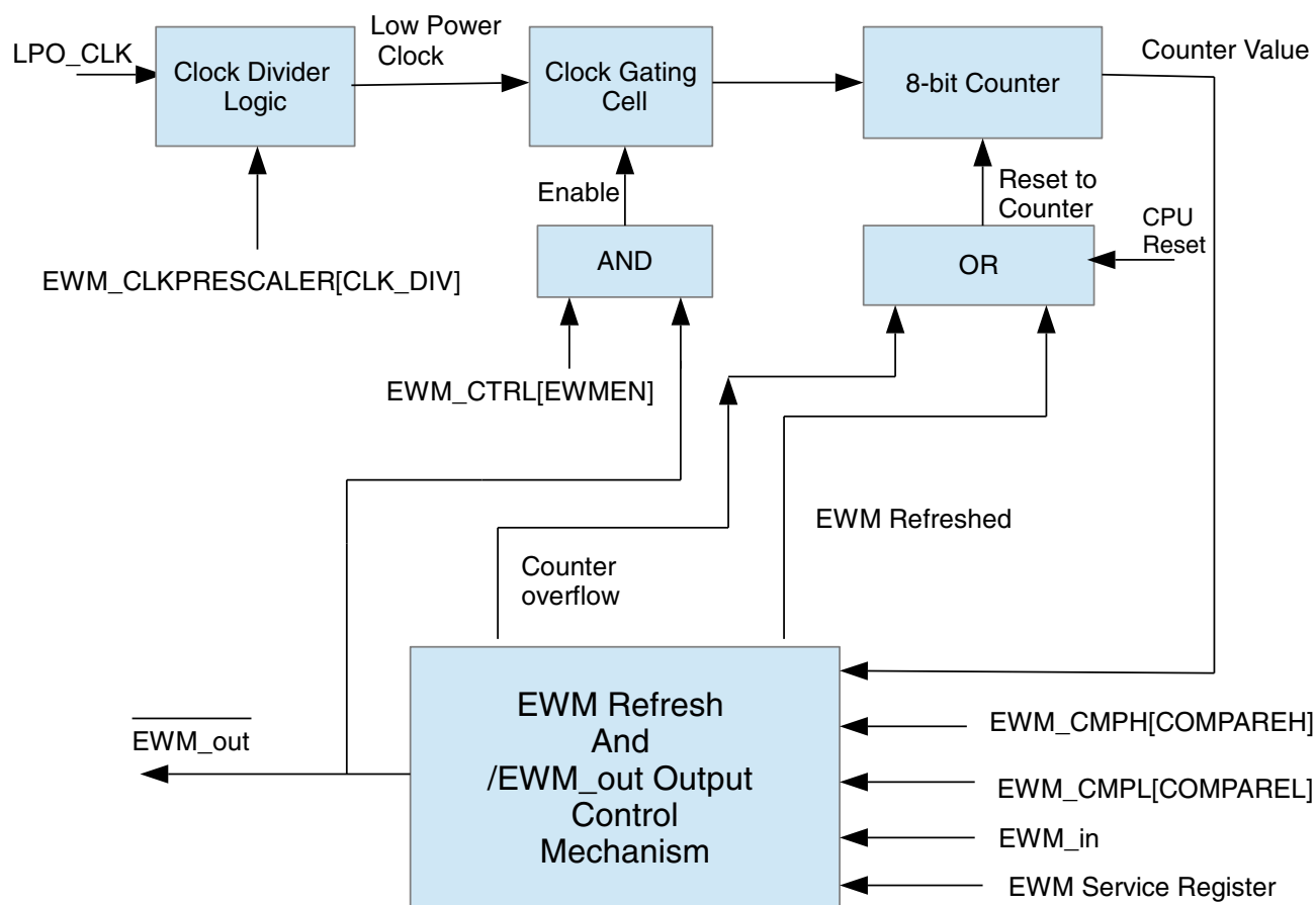
Figure 29-1. EWM Block Diagram
