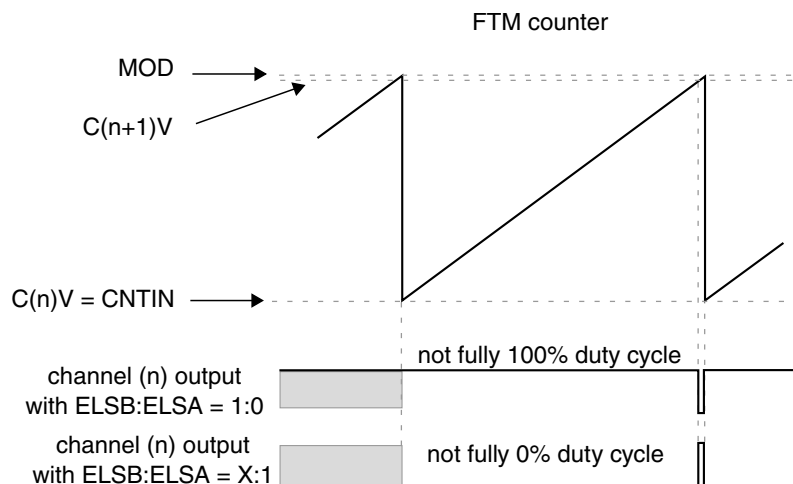
Figure 41-29. Channel (n) output if (C(n)V = \text{CNTIN}) and (\text{CNTIN} < C(n+1)V < \text{MOD}) and C(n+1)V is Almost Equal to \text{MOD}
