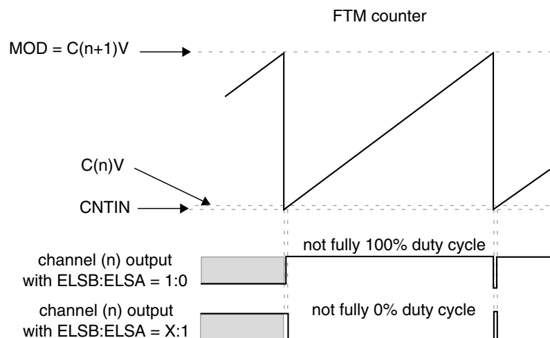
Figure 41-28. Channel (n) output if (\text{CNTIN} < C(n)V < \text{MOD}) and C(n)V is Almost Equal to \text{CNTIN} and C(n+1)V = \text{MOD}
