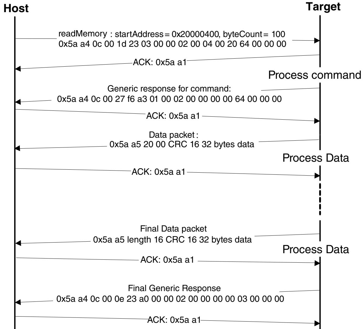
Figure 23-15. Command sequence for read memory
