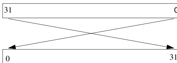
Figure 31-3. Transpose type 10
