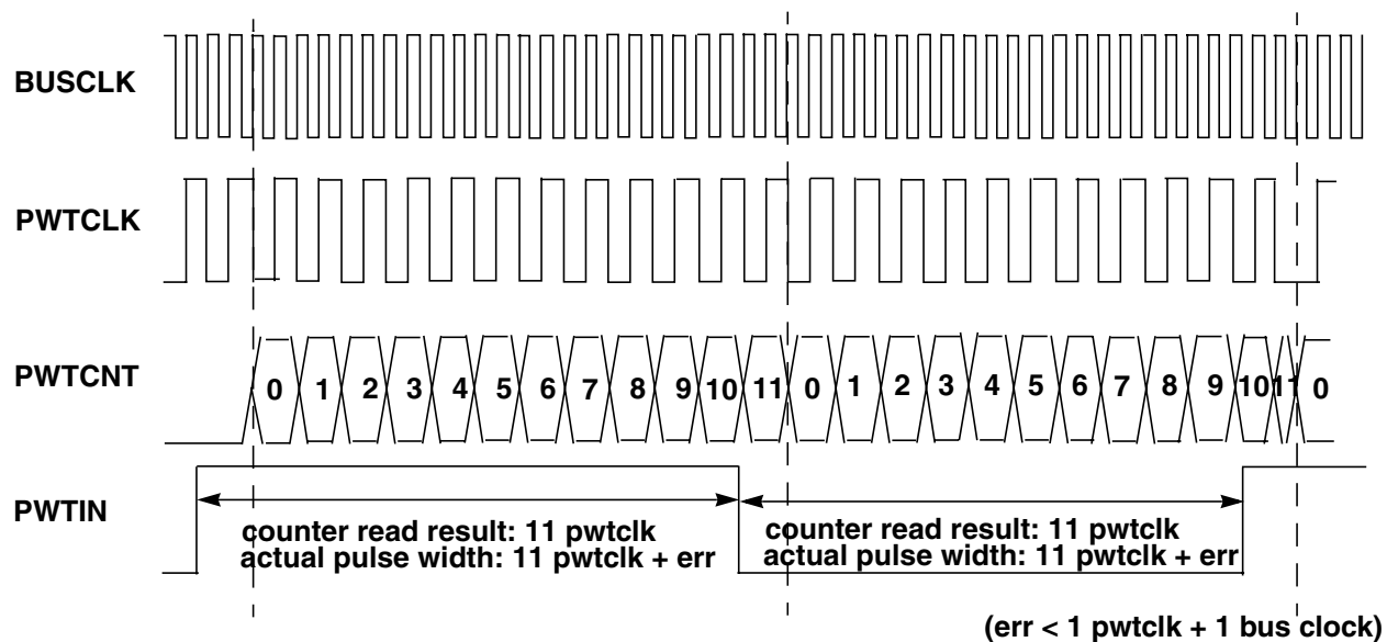
Figure 43-9. Example at PWTCLK is Bus Clock divided by 2
