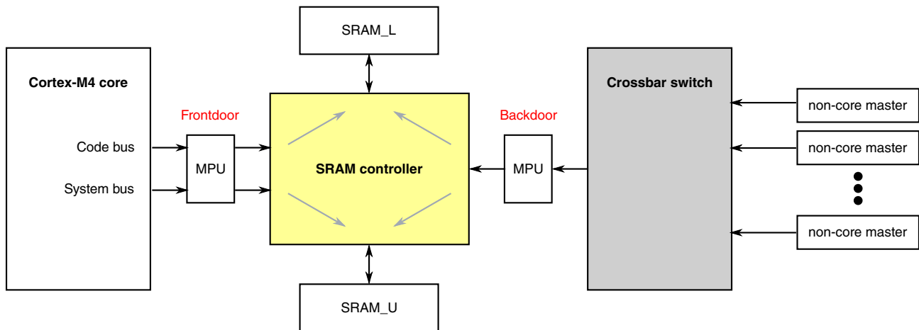
Figure 13-2. SRAM access diagram
