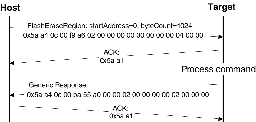
Figure 23-11. Protocol Sequence for FlashEraseRegion Command
