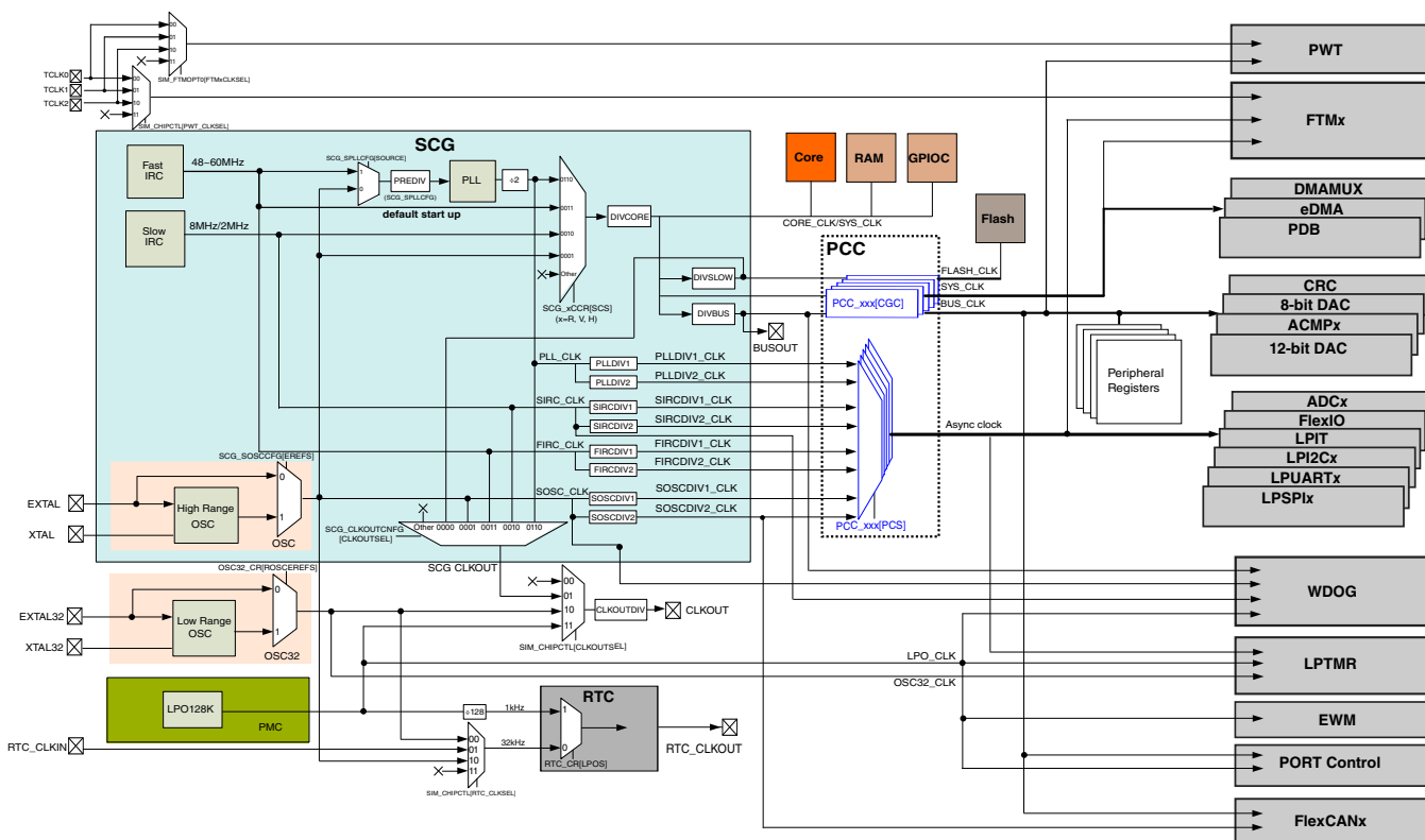
Figure 18-1. Clocking Diagram
