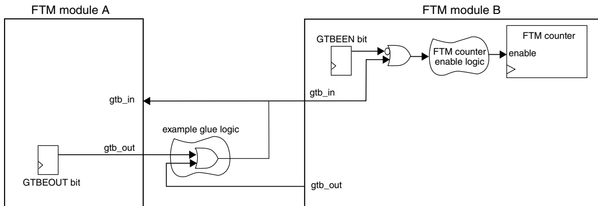
Figure 41-101. Global time base (GTB) block diagram
