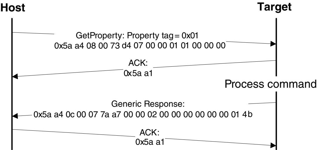
Figure 23-8. Protocol Sequence for GetProperty Command
