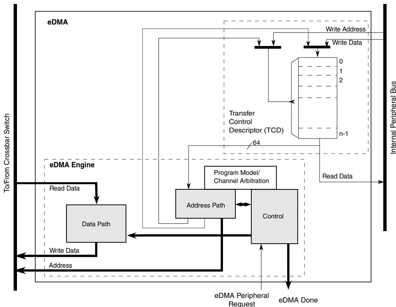
Figure 12-3. eDMA operation, part 2
