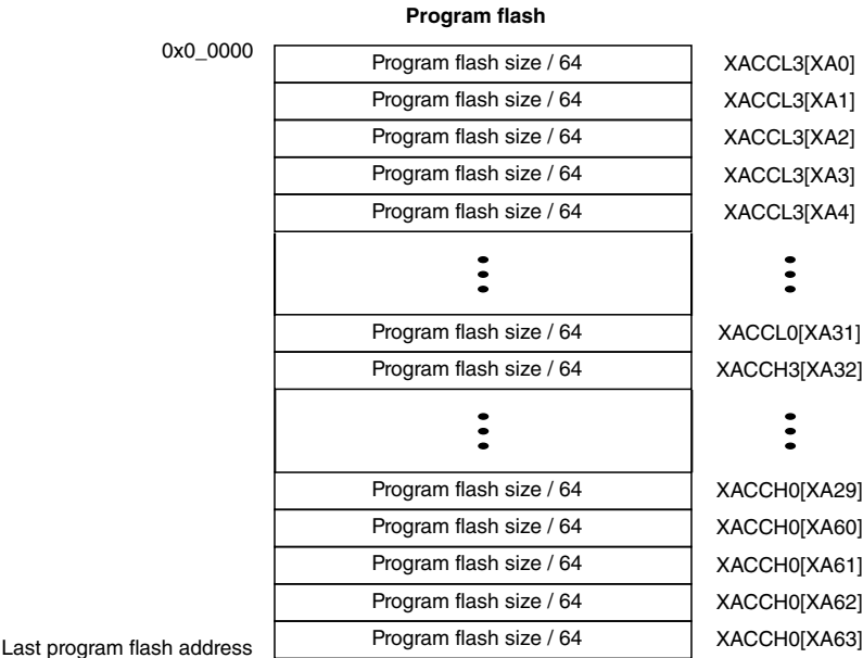
Figure 17-5. Program flash execute-only access control
