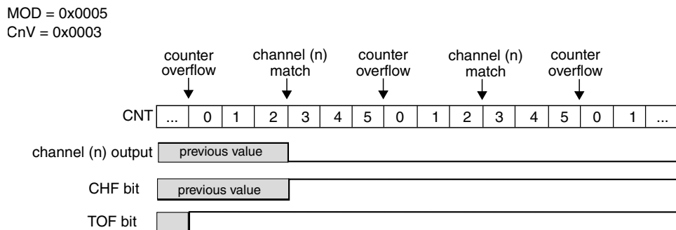
Figure 41-16. Example of the Output Compare mode when the match clears the channel output
