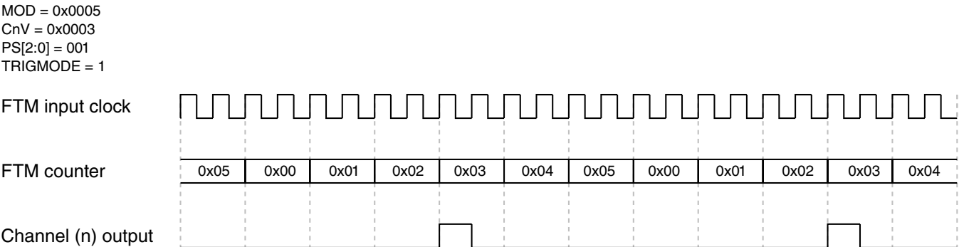
Figure 41-77. Example of trigger generation in the output channel for up counting mode
