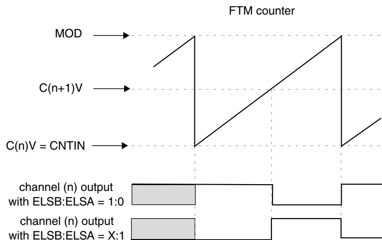
Figure 41-27. Channel (n) output if (C(n)V = \text{CNTIN}) and (\text{CNTIN} < C(n+1)V < \text{MOD})
