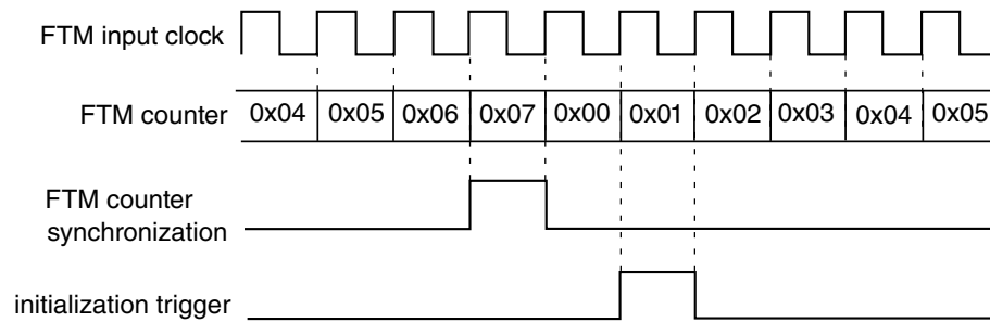
Figure 41-81. Initialization trigger is generated when there is the FTM counter synchronization
