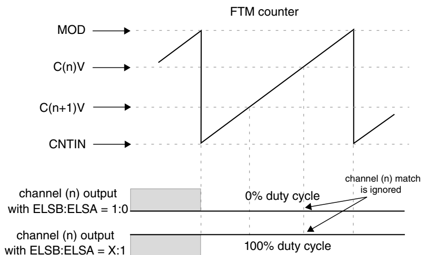
Figure 41-34. Channel (n) output if (\text{CNTIN} < C(n)V < \text{MOD}) and (\text{CNTIN} < C(n+1)V < \text{MOD}) and (C(n)V > C(n+1)V)
