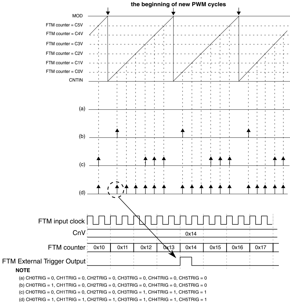
Figure 41-76. External Trigger
