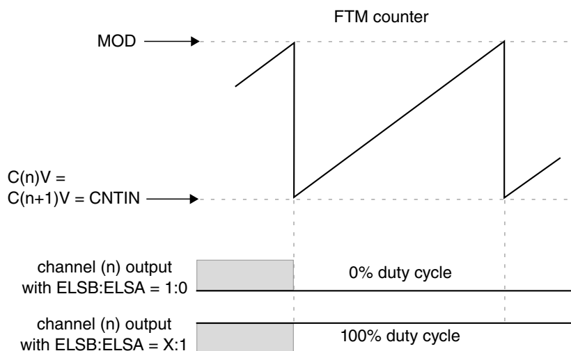
Figure 41-32. Channel (n) output if (C(n)V = C(n+1)V = \text{CNTIN})
