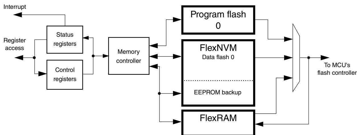
Figure 17-1. FTFE block diagram
