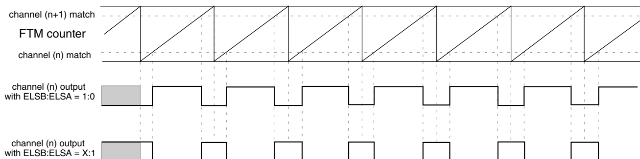
Figure 41-24. Combine mode
