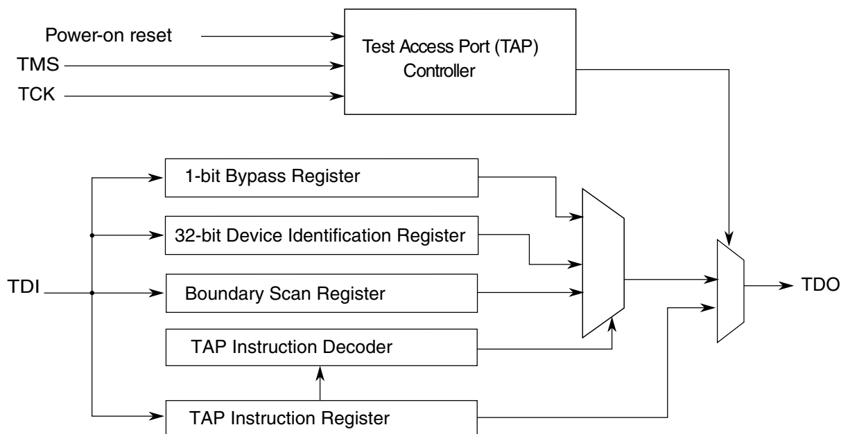
Figure 33-1. JTAG (IEEE 1149.1) block diagram
