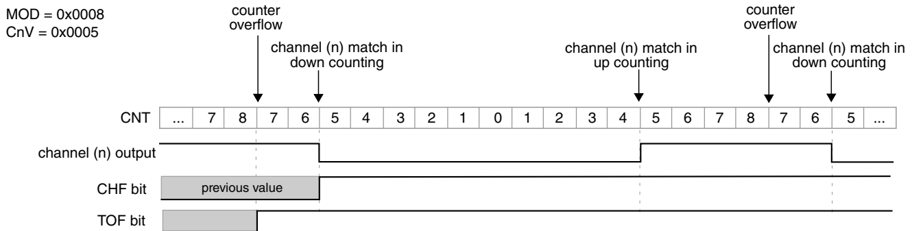
Figure 39-25. CPWM signal with ELSB:ELSA = X:1
