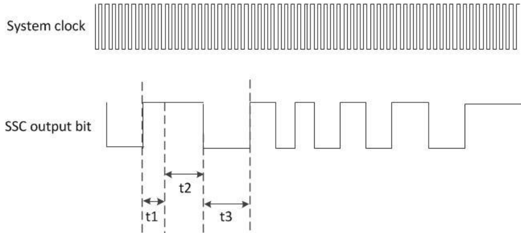
Figure 48-9. Spread spectrum clacking timing
