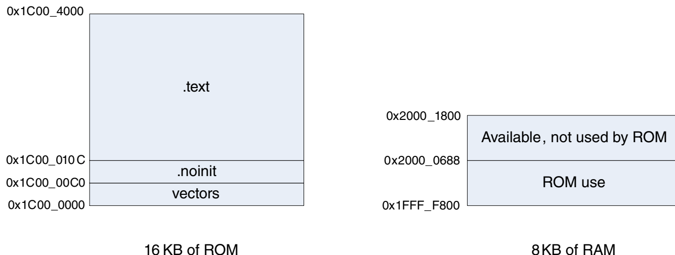
Figure 22-1. Kinetis Bootloader ROM/RAM Memory Maps
