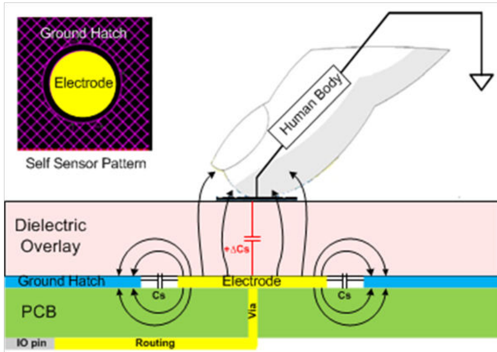
Figure 48-2. Self-cap Touch Sensor structure and Electric field
