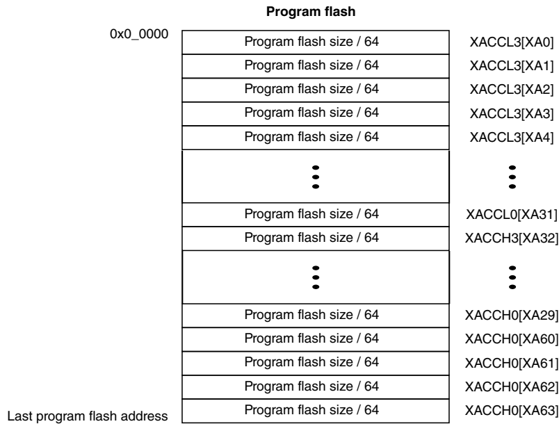
Figure 16-5. Program flash execute-only access control
