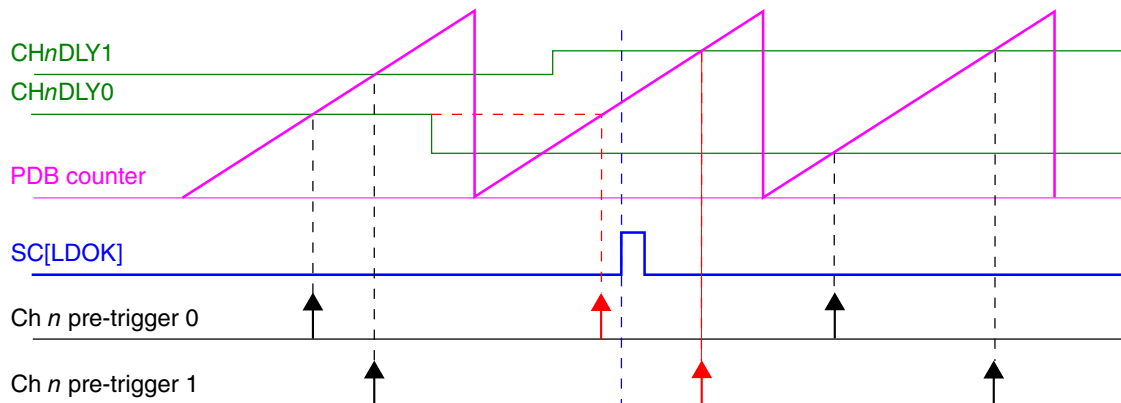
Figure 38-4. Registers update with SC[LDMOD] = 00
