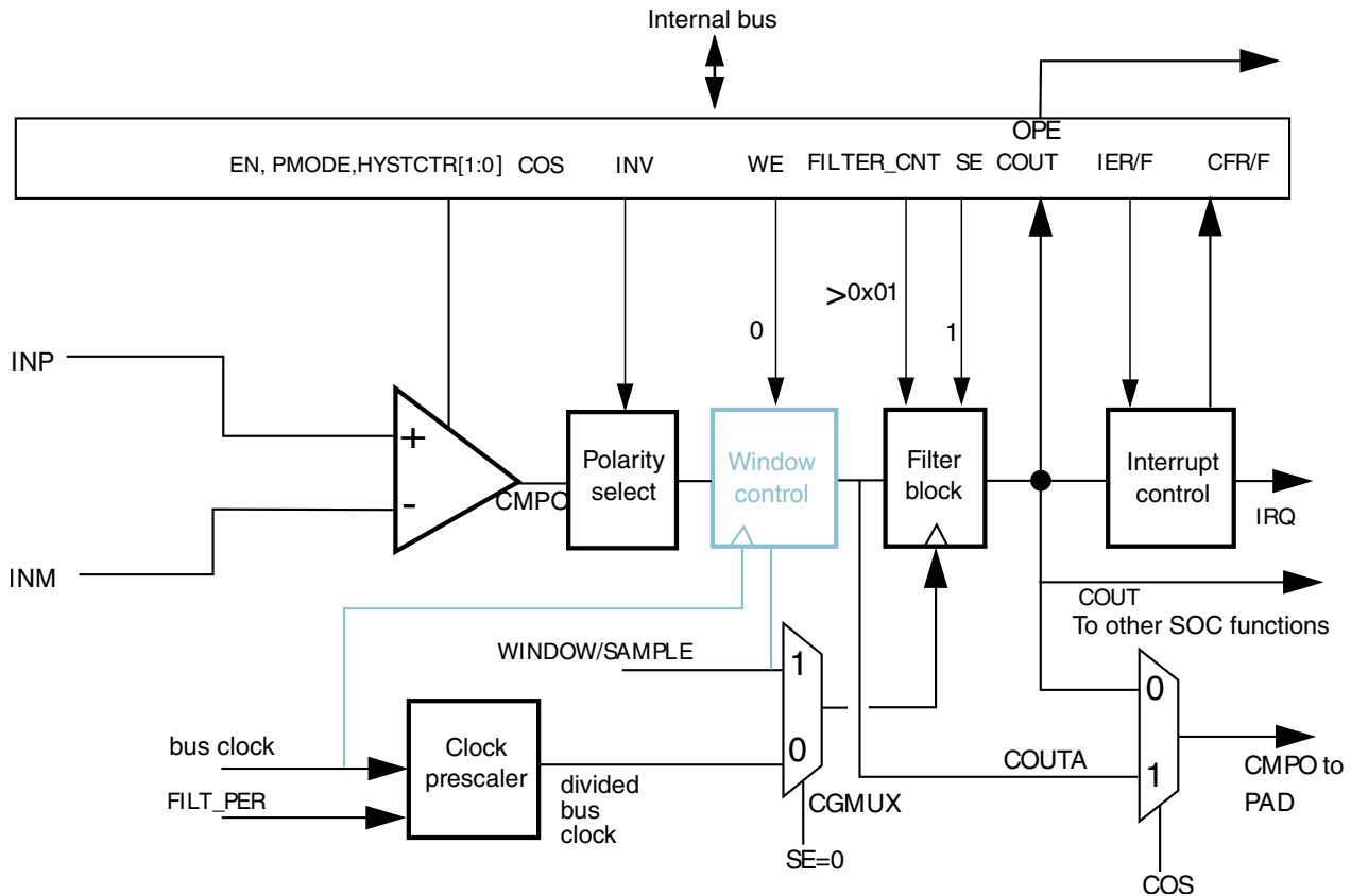
Figure 37-9. Sampled, Filtered (# 4B): sampling point internally derived
