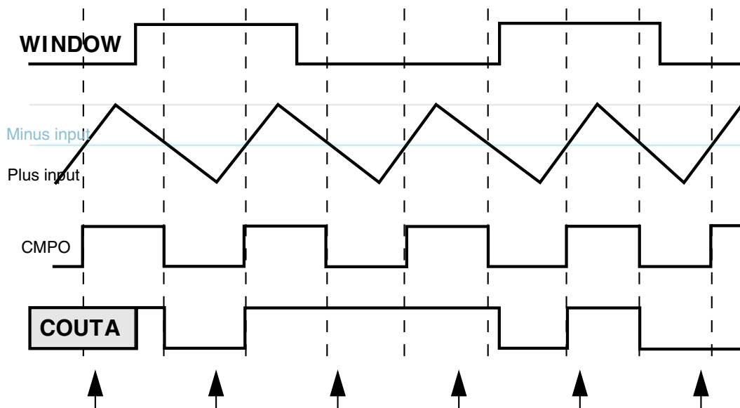
Figure 37-10. Windowed mode timing diagram
