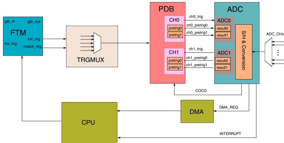
Figure 36-3. PWM Load Diagnosis – ADC Trigger Concept (block diagram)
