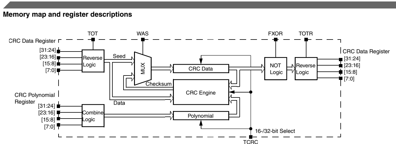
Figure 30-1. Programmable cyclic redundancy check (CRC) block diagram
