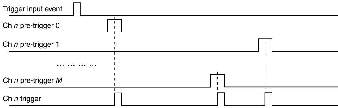
Figure 38-2. Pre-trigger and trigger outputs
