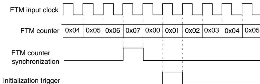
Figure 39-83. Initialization trigger is generated when there is the FTM counter synchronization
