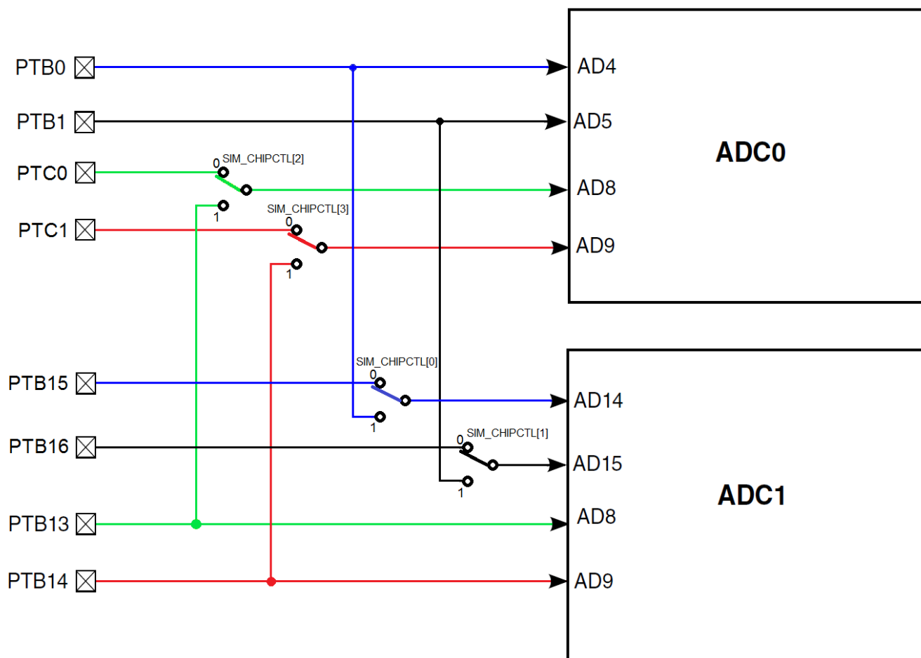
Figure 36-1. ADC0 and ADC1 hardware interleaved channels integration
