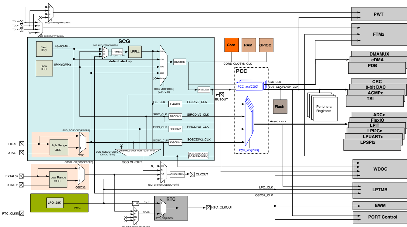
Figure 17-1. Clocking Diagram
