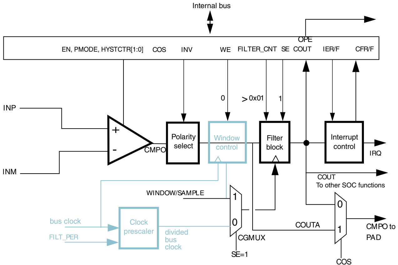
Figure 37-8. Sampled, Filtered (# 4A): sampling point externally driven
