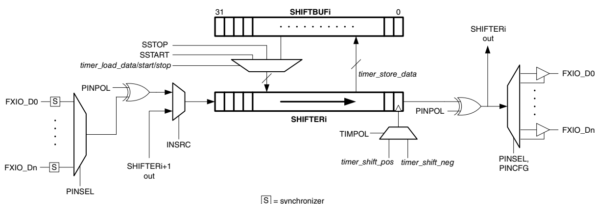
Figure 47-2. Shifter Microarchitecture
