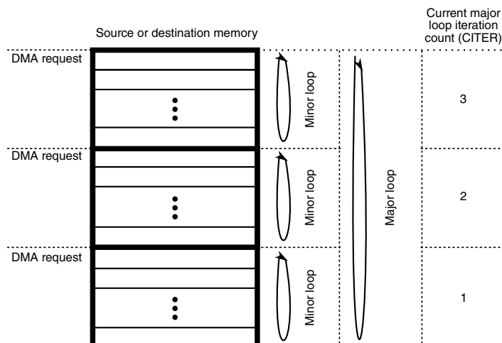
Figure 13-5. Example of multiple loop iterations
