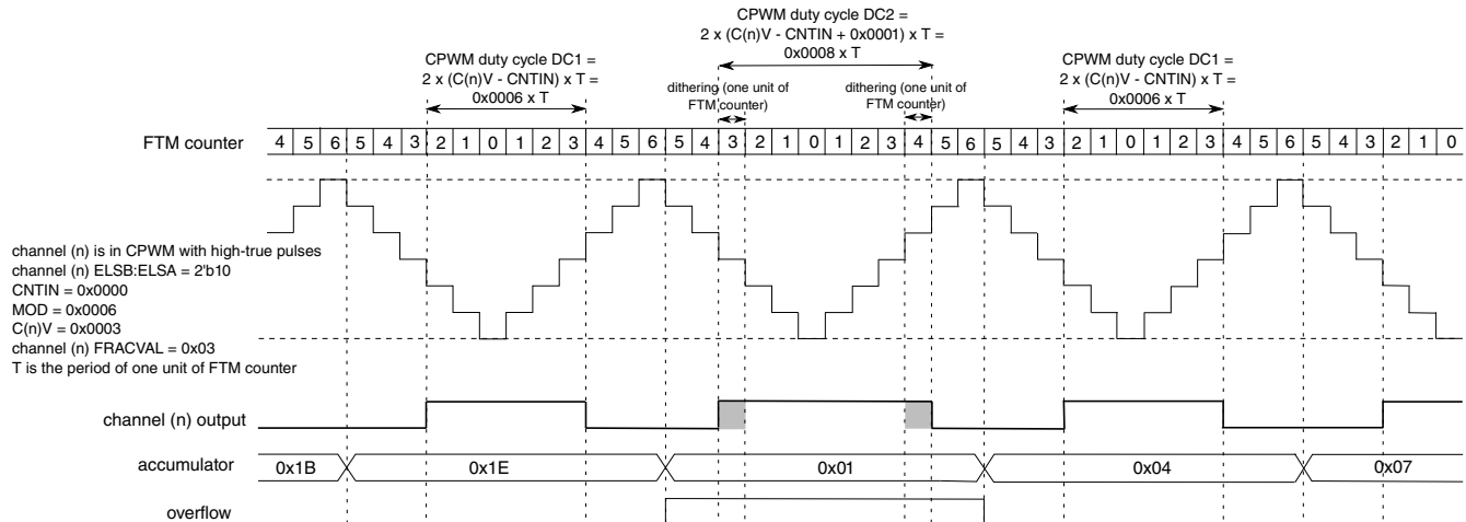
Figure 39-109. Channel (n) is in CPWM Mode with PWM Edge Dithering
