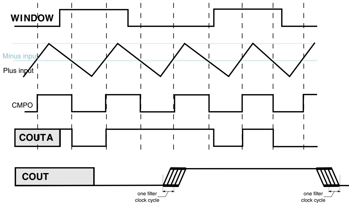
Figure 37-14. Windowed/Filtered mode operation
