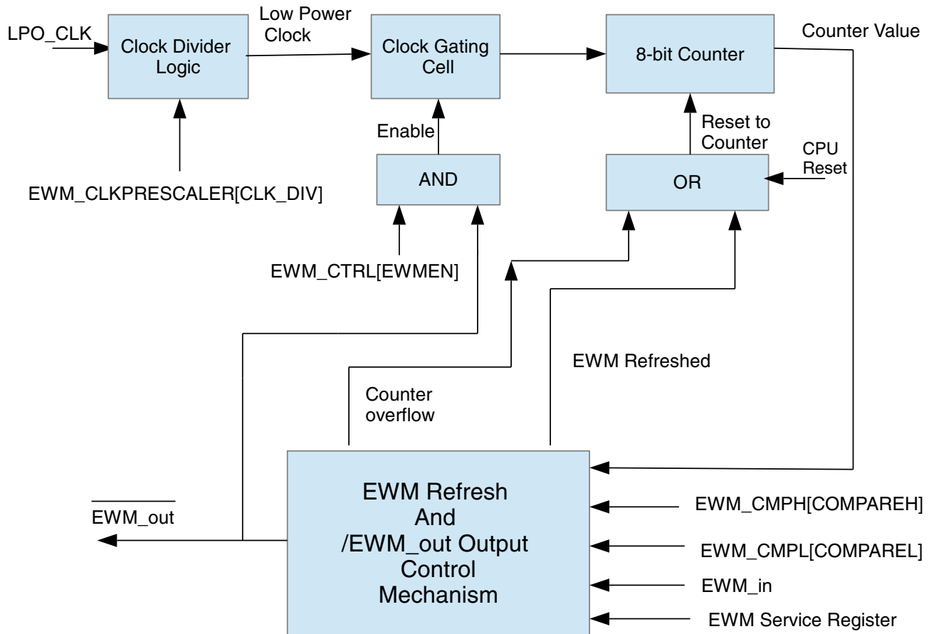
Figure 28-1. EWM Block Diagram
