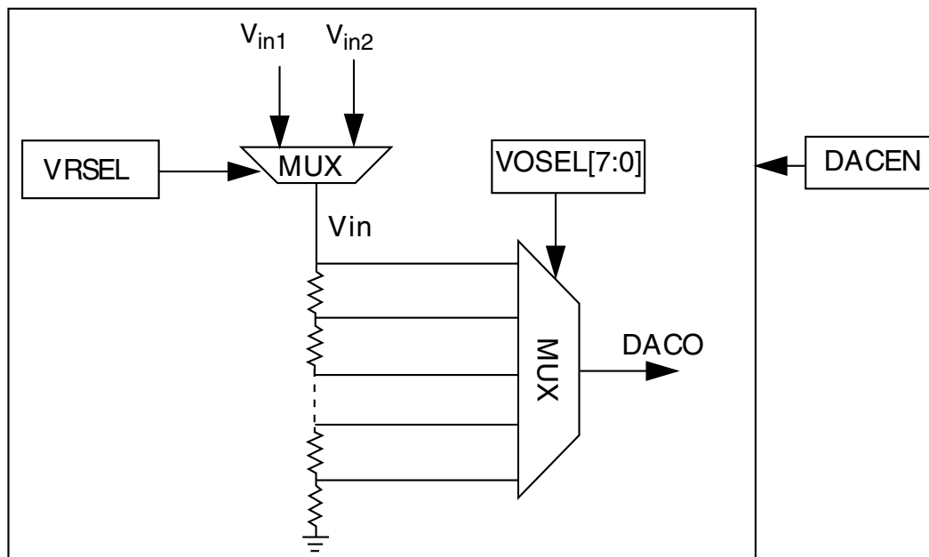
Figure 37-15. 8-bit DAC block diagram
