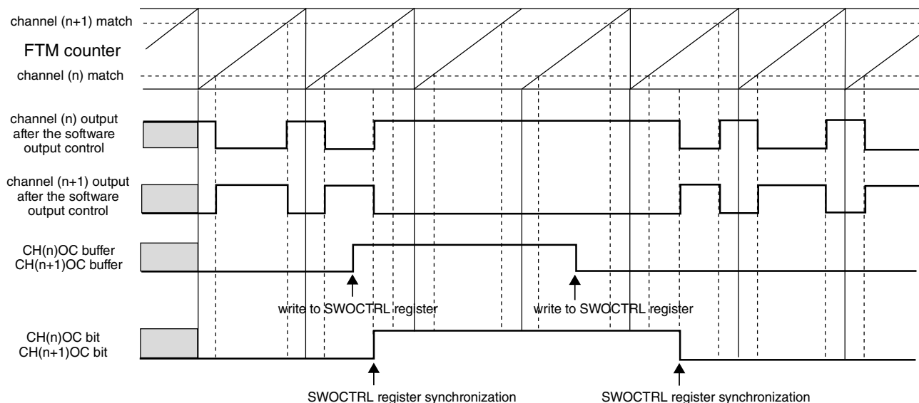
Figure 39-67. Example of software output control in Combine and Complementary mode
