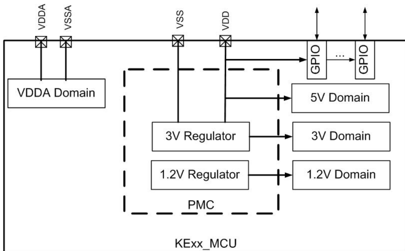
Figure 24-1. Power Infrastructure
