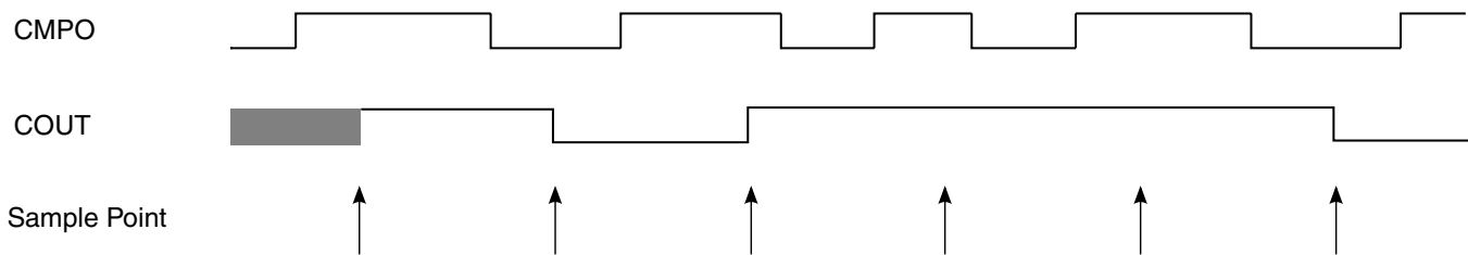
Figure 37-7. Sampled, Non-Filtered Mode Timing Diagram
