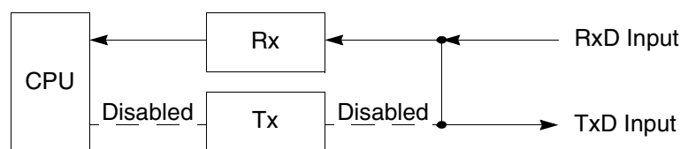
Figure 15-13 Automatic Echo
