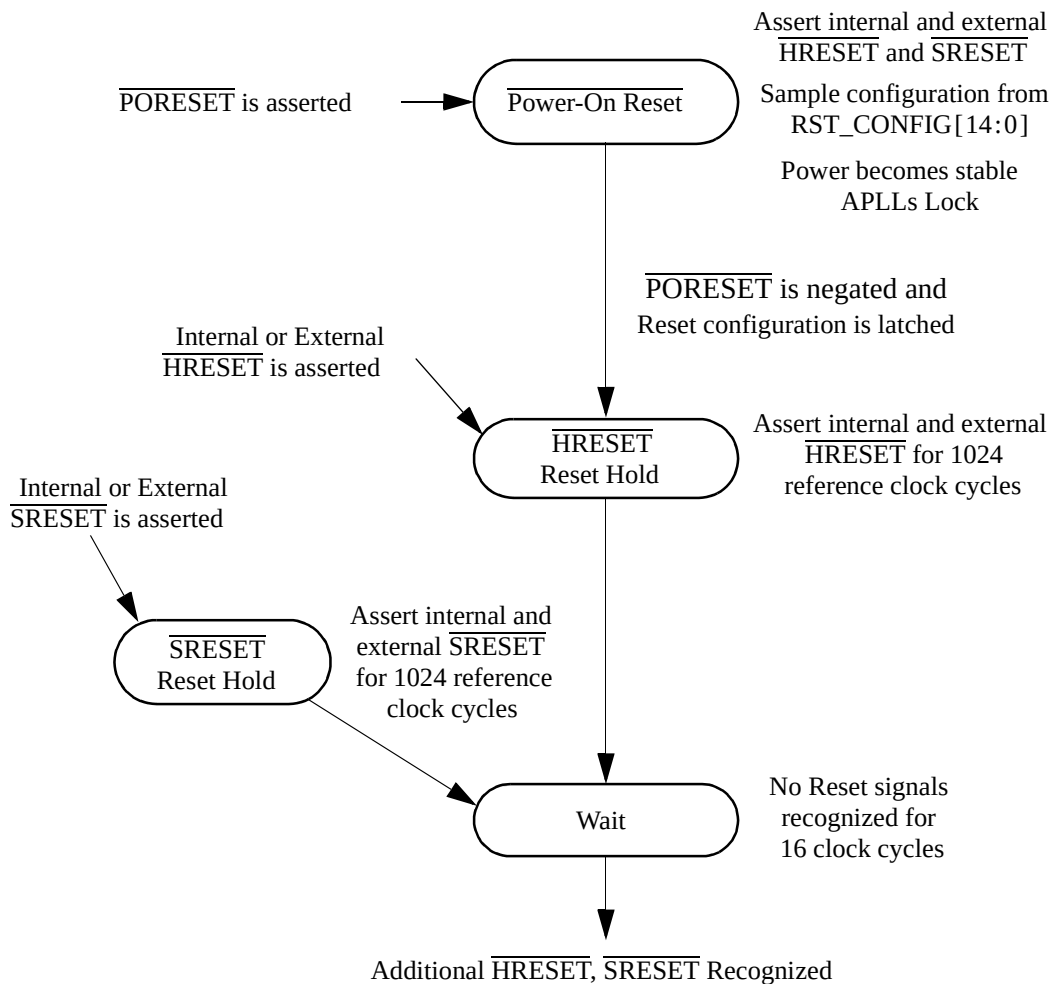
Figure 4-1 Reset sequence
