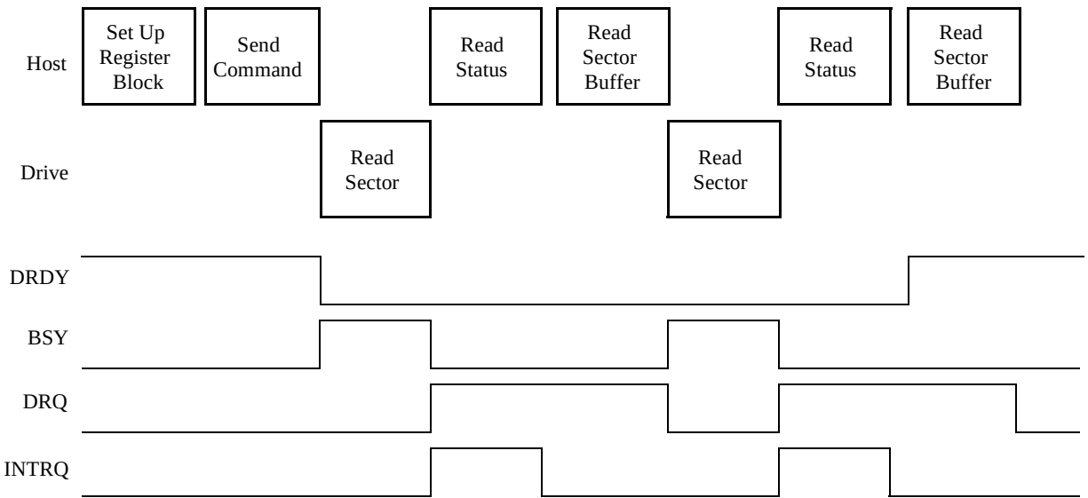
Figure 11-5 Timing Diagram—PIO Read Command (Class 1)
