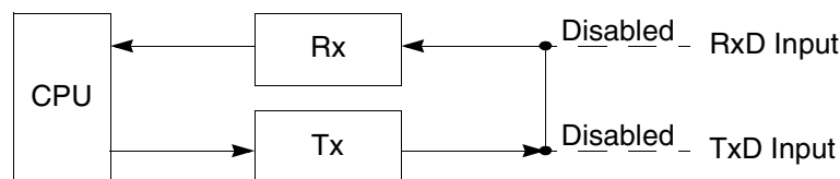
Figure 15-14 Local Loop-Back
