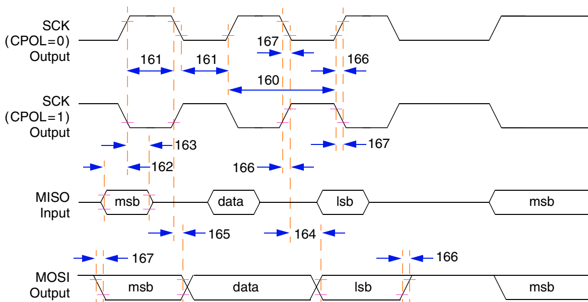
Figure A-31 Timing Diagram—SPI Master (CPHA=0)
