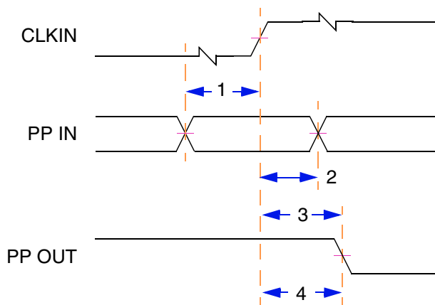
Figure A-38 Timing Diagram—General-Purpose I/O
