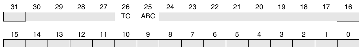
Figure 14-3 Transmit Frame Control Word Format
