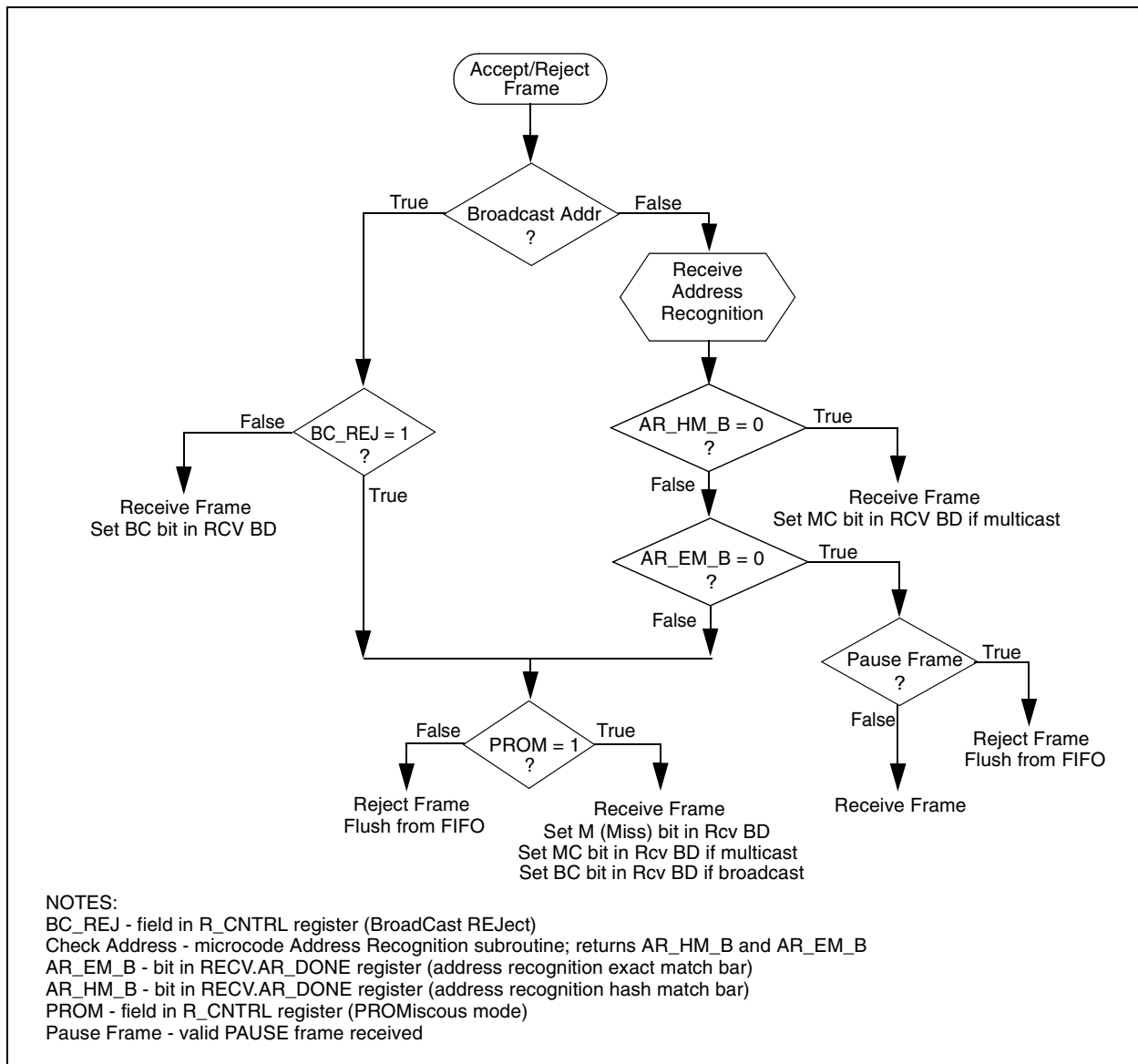
Figure 14-4 Ethernet Address Recognition - receive block decisions
