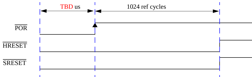
Figure 4-2 \overline{\text{PORESET}} Assertion
