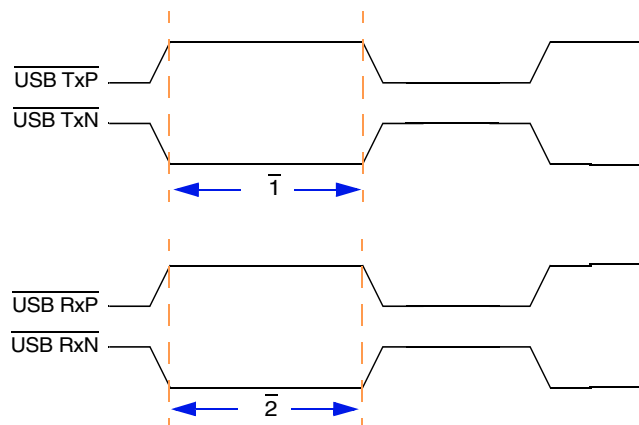
Figure A-30 Timing Diagram—USB
