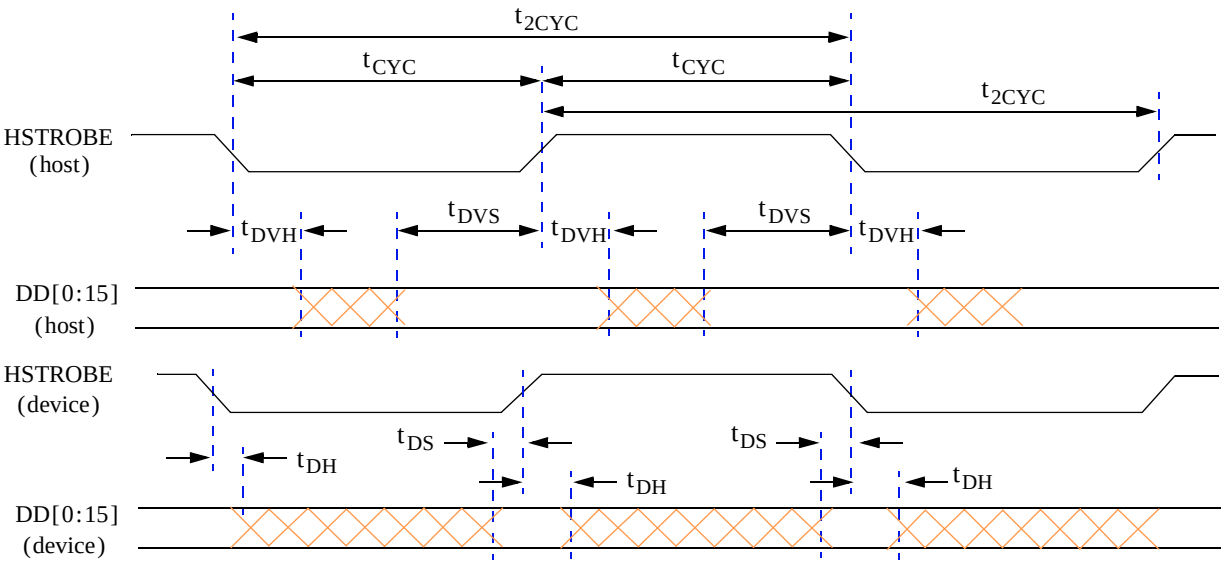
Figure 11-19 Timing Diagram—Sustained Ultra DMA Data Out Burst
