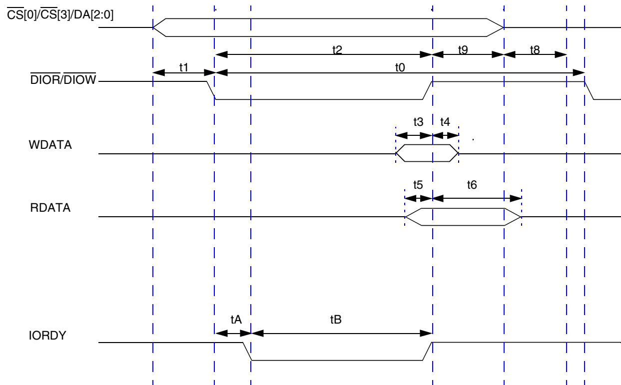
Figure A-12 PIO Mode Timing
