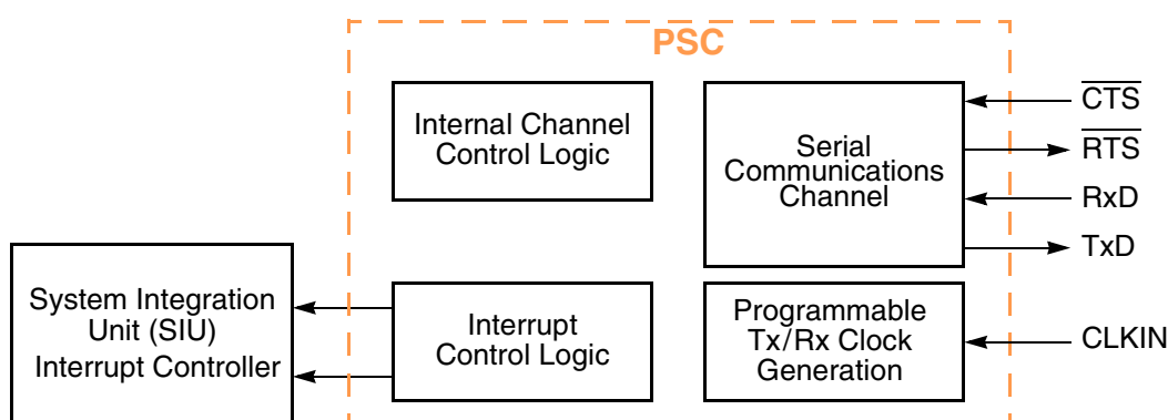
Figure 15-1 Simplified Block Diagram
