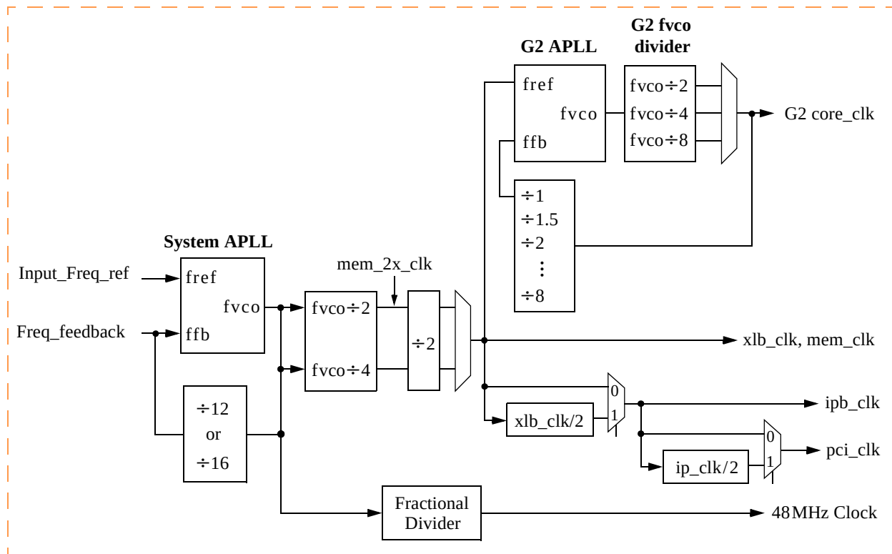
Figure 5-3 Bus Clock Ratios
