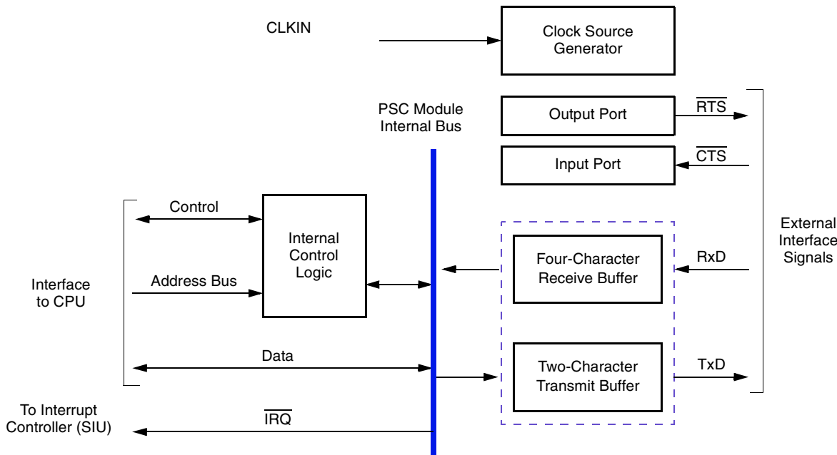
Figure 15-2 Block Diagram—PSC
