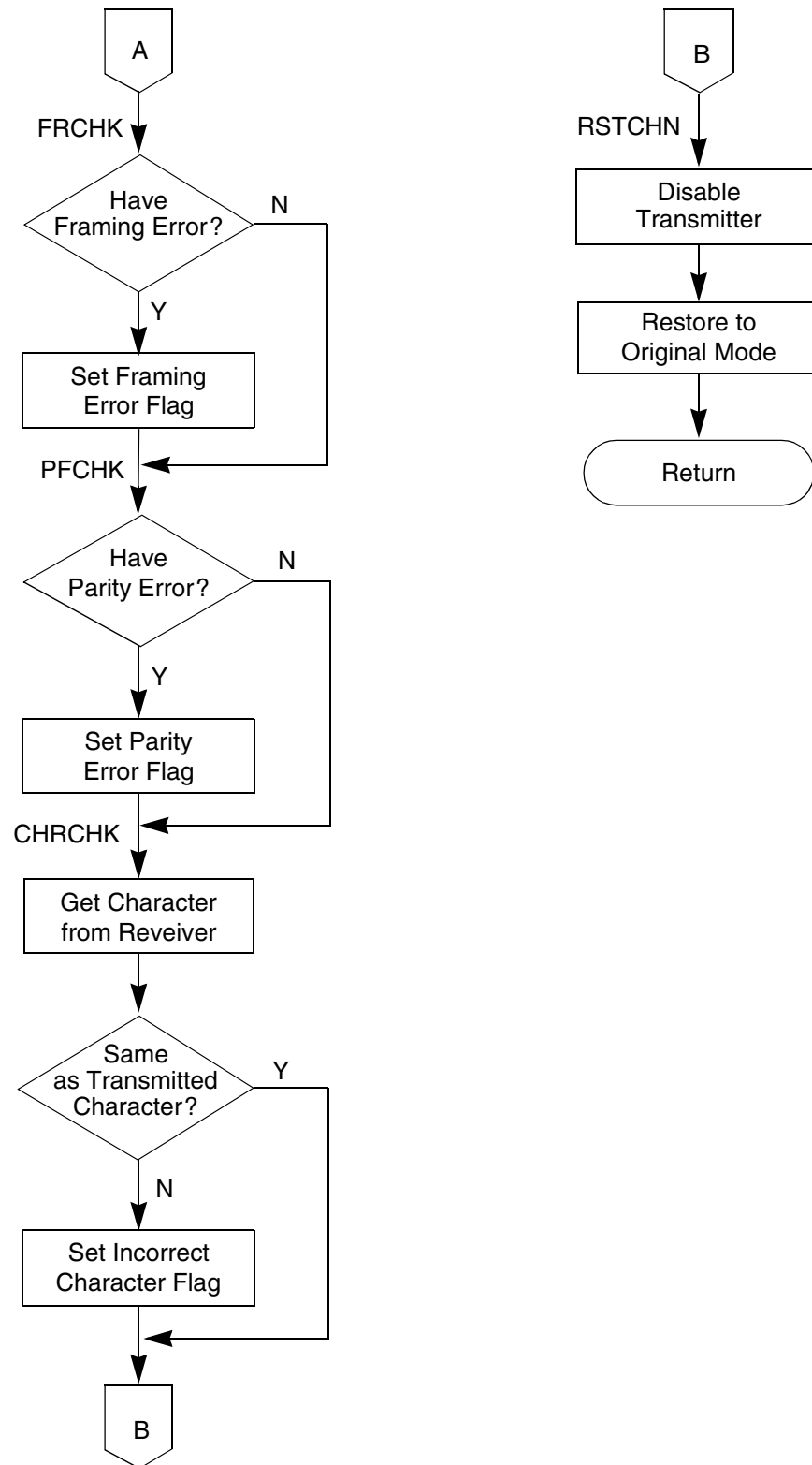
Figure 15-19 Programming Flowchart—UART Mode (sheet 3 of 5)
