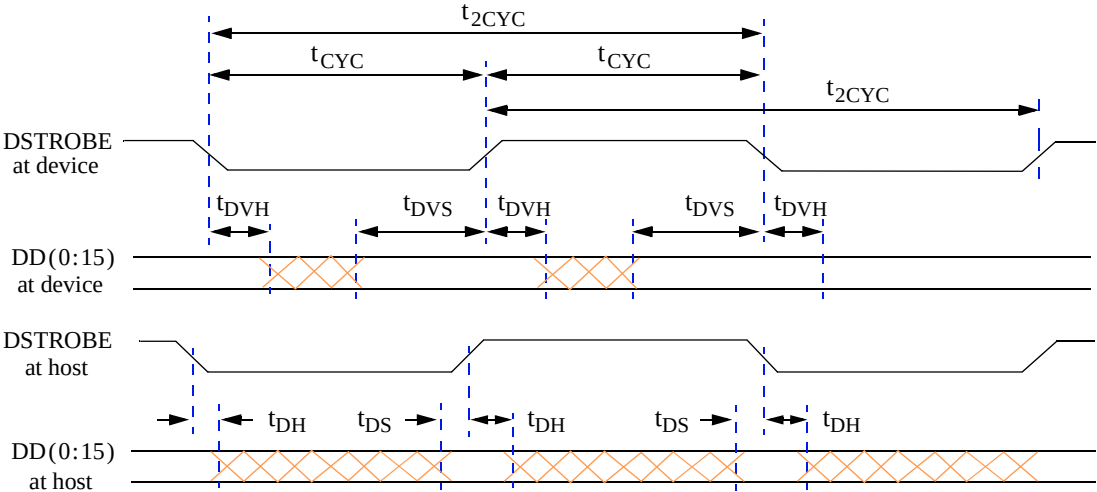
Figure 11-14 Timing Diagram—Sustained Ultra DMA Data In Burst
