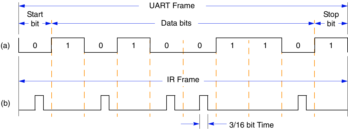
Figure A-23 IrDA Timing Diagram—Low-Speed Data Format
