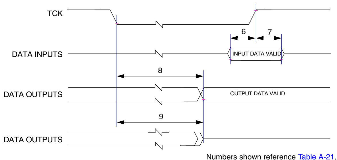
Figure A-28 Timing Diagram—JTAG Boundary Scan
