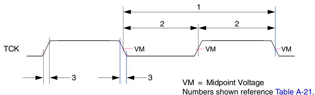
Figure A-26 Timing Diagram—JTAG Clock Input
