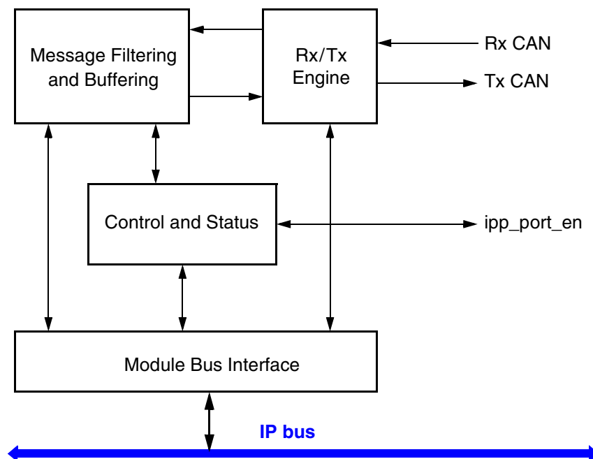
Figure 20-1 Block Diagram—MSCAN
