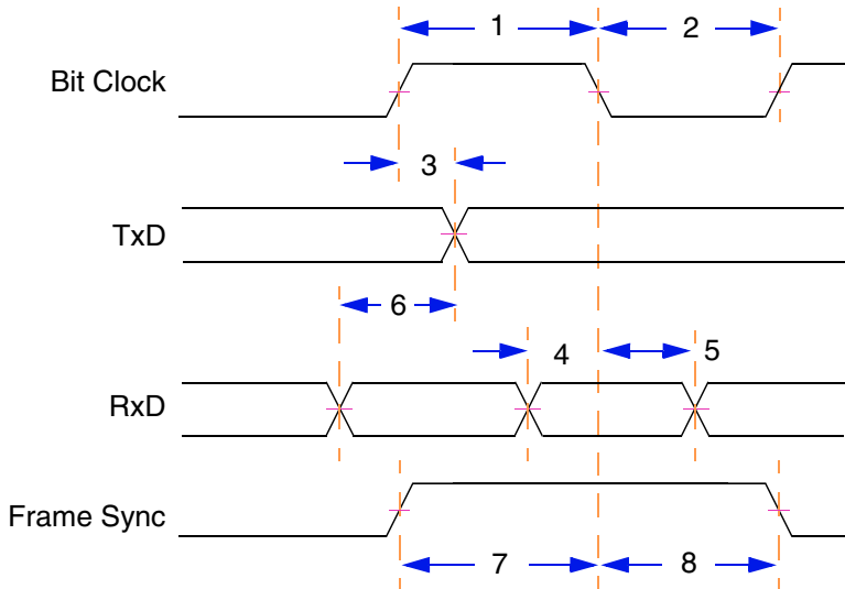
Figure A-36 Timing Diagram—8- and 16-bit CODEC Mode
