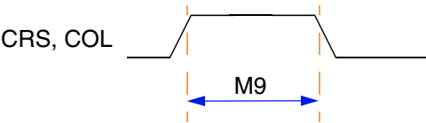
Figure A-20 Ethernet Timing Diagram—MII Async
