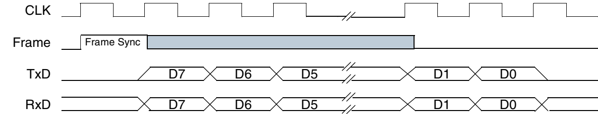
Figure 15-10 Timing Diagram—8-Bit CODEC Interface (msb First)
