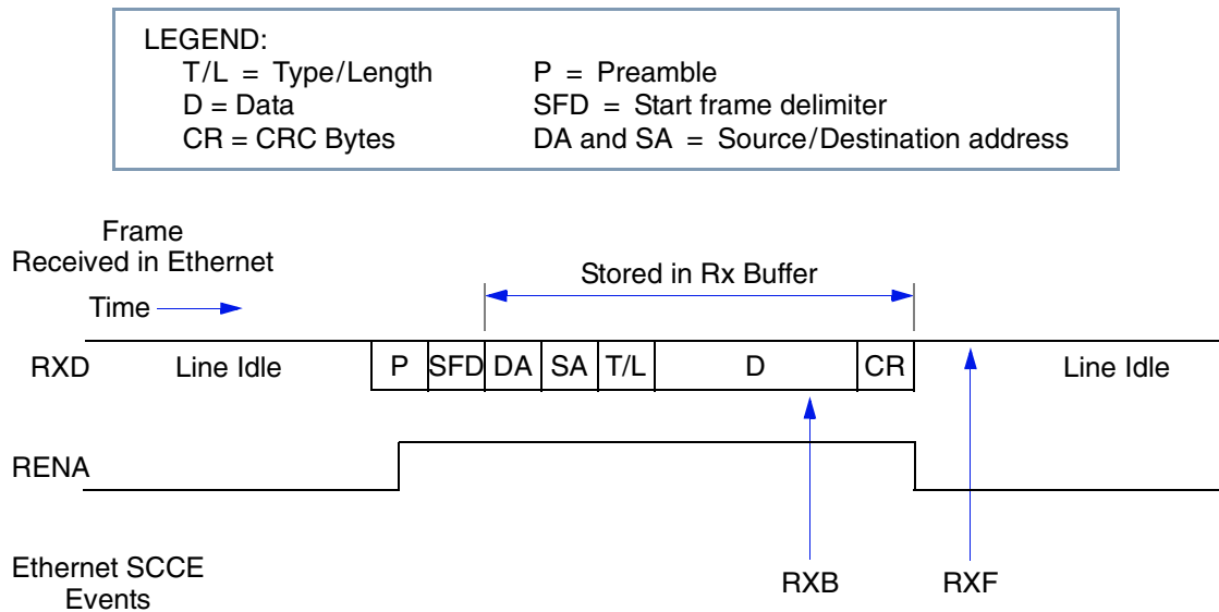
Figure A-15 Ethernet Timing Diagram—Interrupt Events Tx Example
