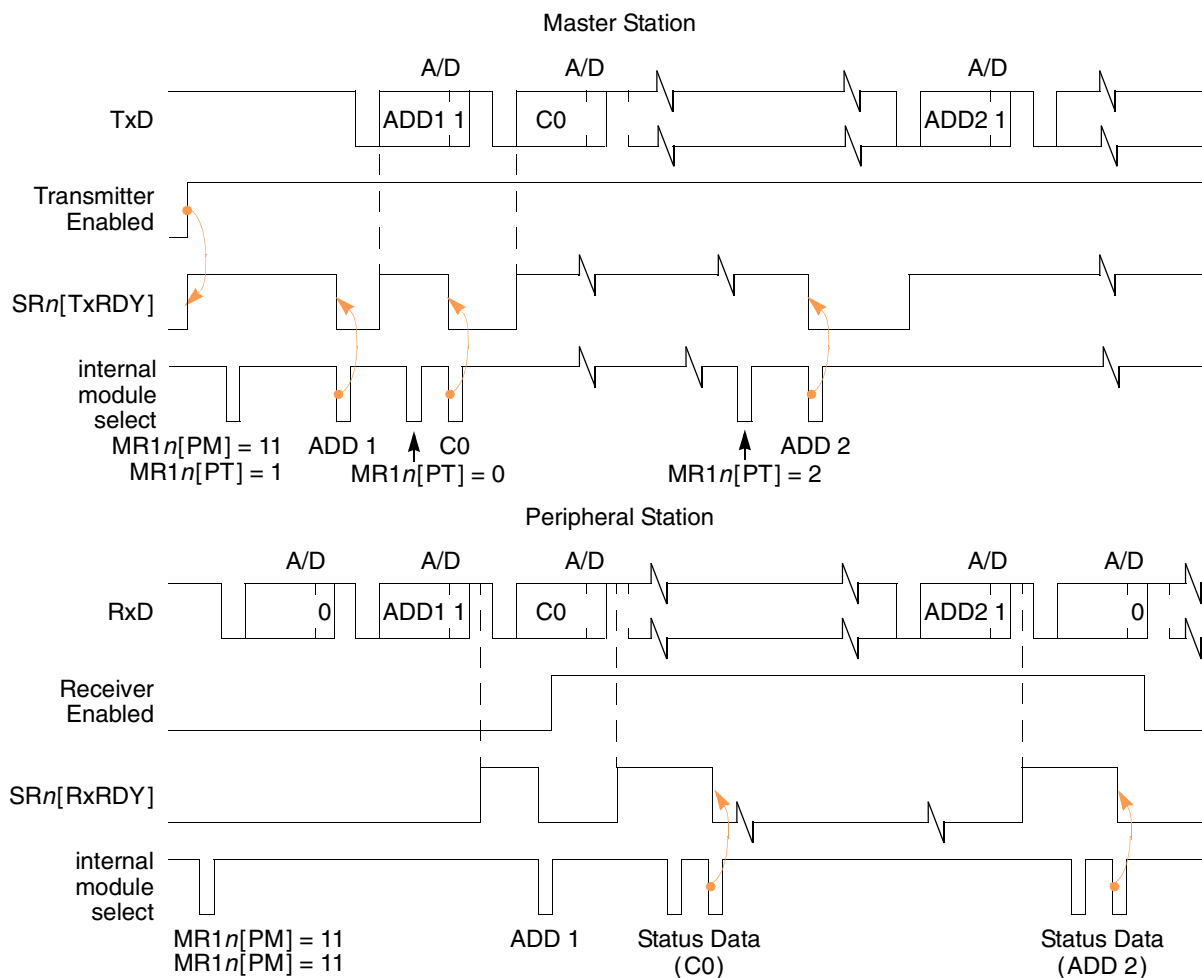
Figure 15-16 Timing Diagram—Multidrop Mode
