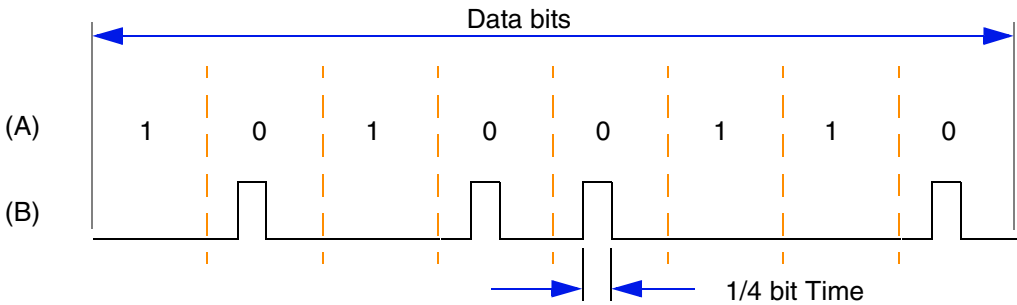
Figure A-24 IrDA Timing Diagram—Middle-Speed Data Format
