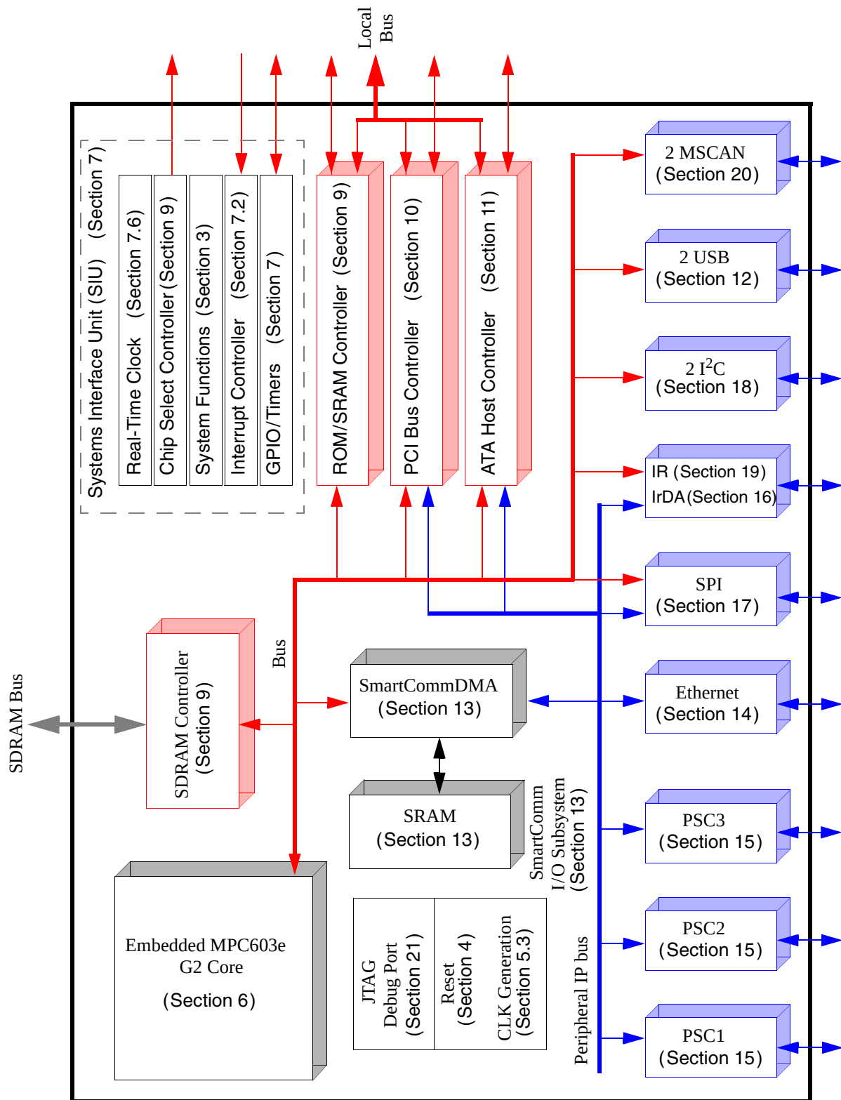
Figure 1-1 Simplified Block Diagram—MGT5100
