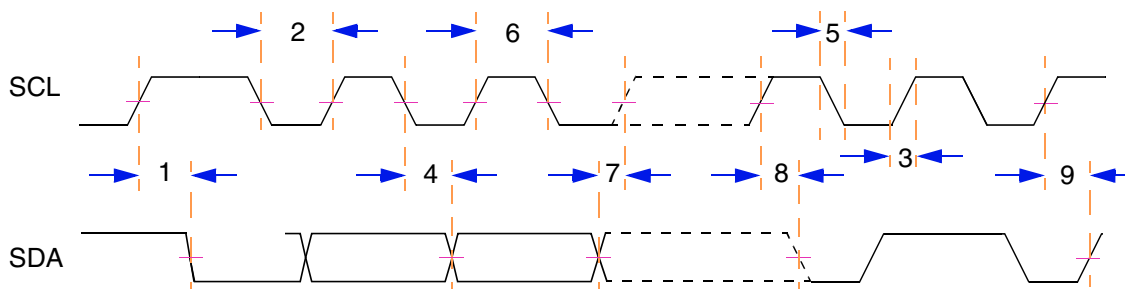
Figure A-34 Timing Diagram—I 2 C Input/Output
