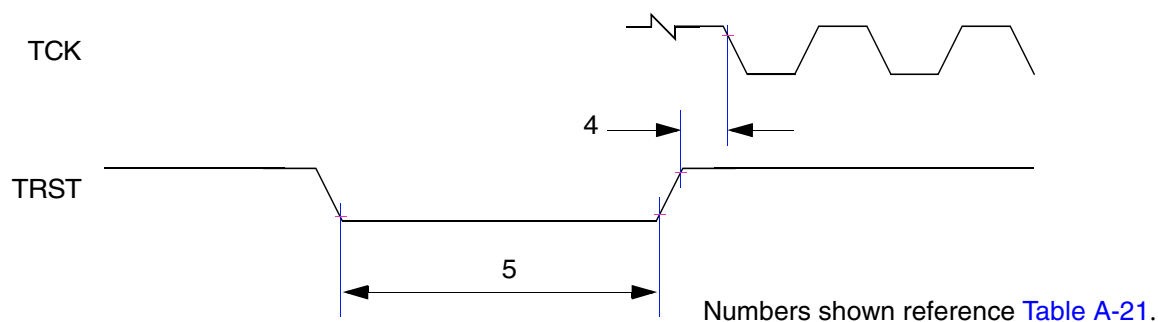
Figure A-27 Timing Diagram—JTAG TRST
