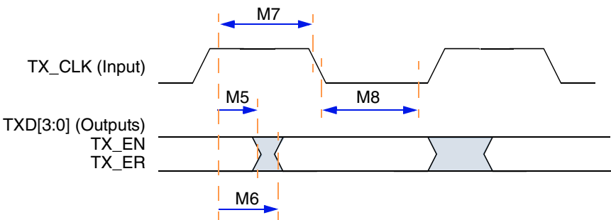
Figure A-19 Ethernet Timing Diagram—MII Tx Signal
