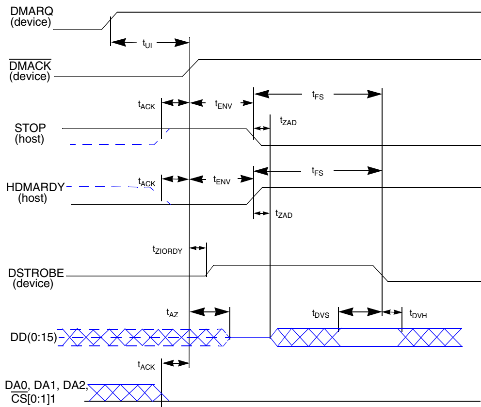
Figure A-14 Initiating an Ultra DMA Data In Burst
