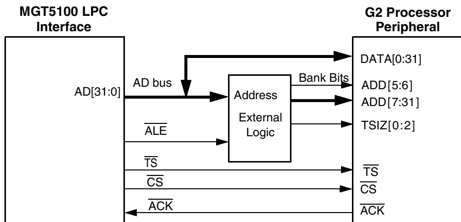
Figure 9-3 Using ALE Transactions
