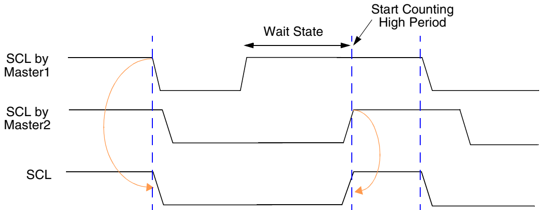
Figure 18-6 Timing Diagram—Clock Synchronization
