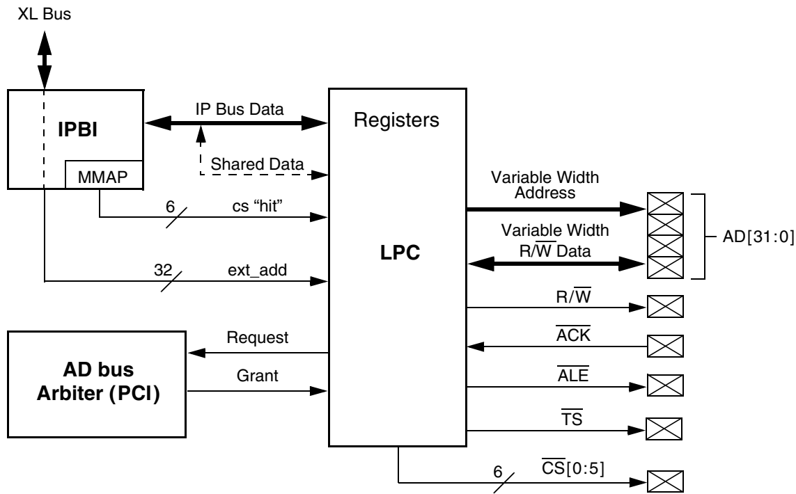
Figure 9-2 LPC Concept Diagram
