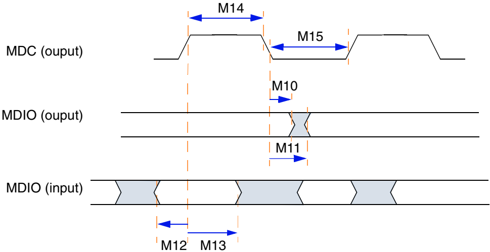
Figure A-21 Ethernet Timing Diagram—MII Serial Management
