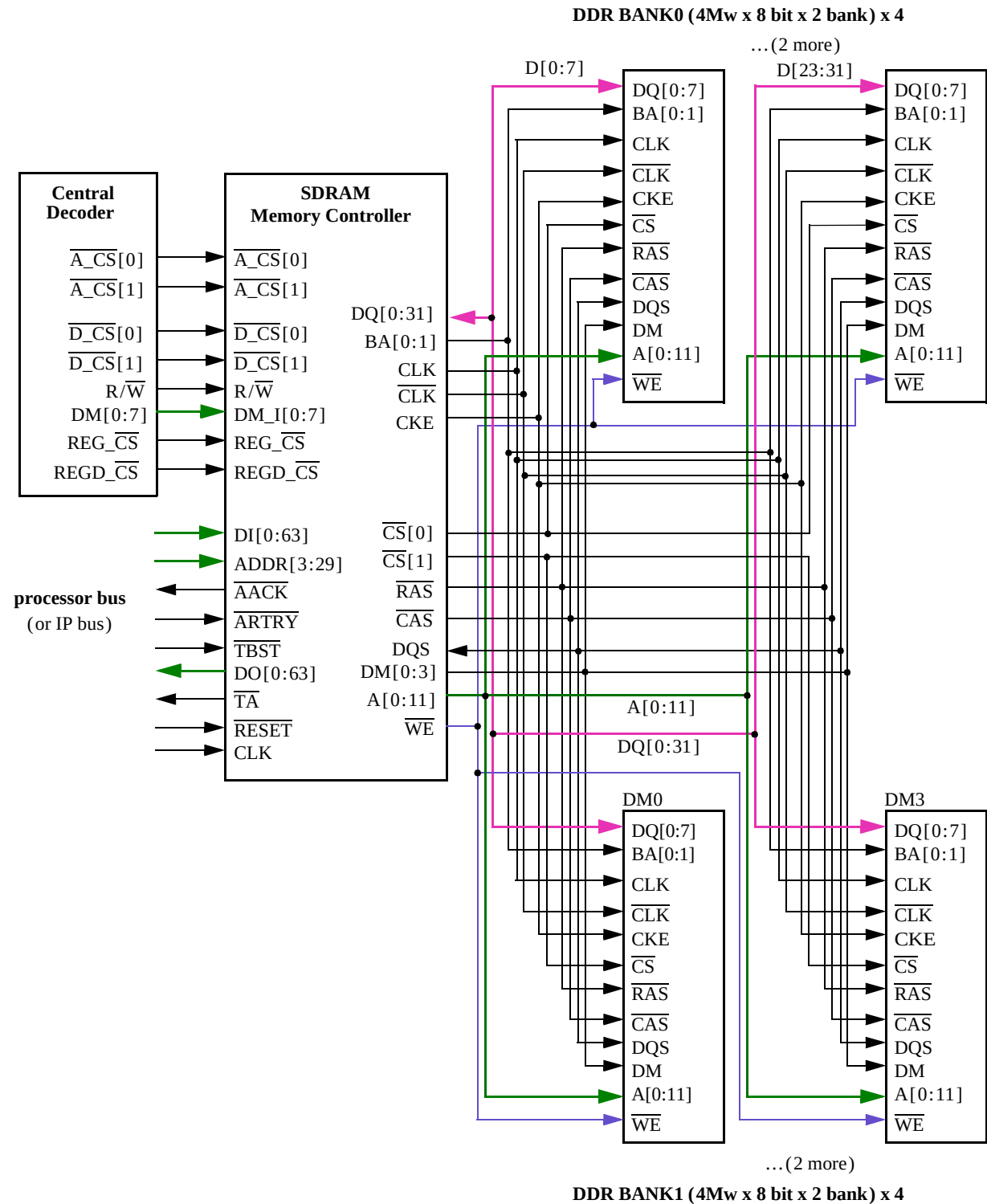
Figure 8-1 Block Diagram—SDRAM Subsystem Example
