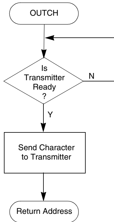
Figure 15-21 Programming Flowchart—UART Mode (sheet 5 of 5)
