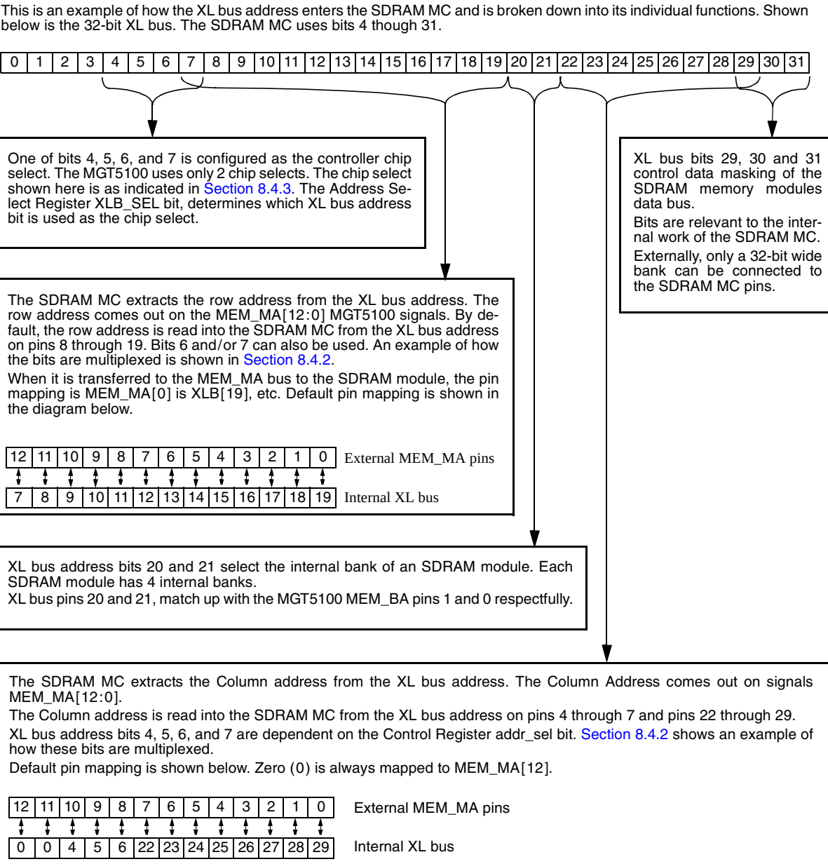
Figure 8-3 Example—Address Bus Mapping
