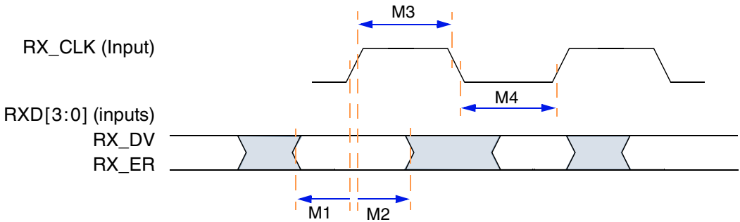
Figure A-17 Ethernet Timing Diagram—MII Rx Signal
