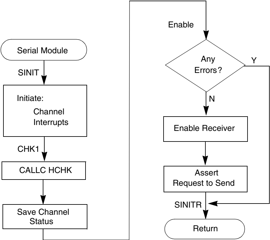
Figure 15-17 Programming Flowchart—UART Mode (sheet 1 of 5)
