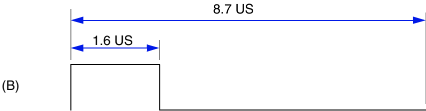
Figure A-22 IR Timing Diagram—SIP Waveform
