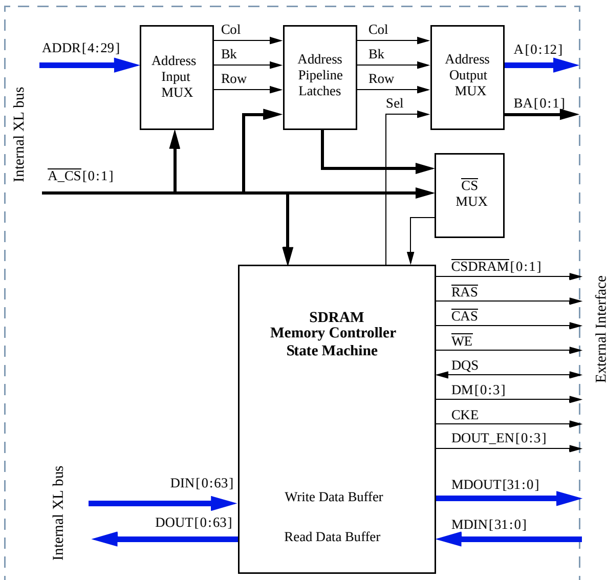
Figure 8-2 Block Diagram—SDRAM Memory Controller
