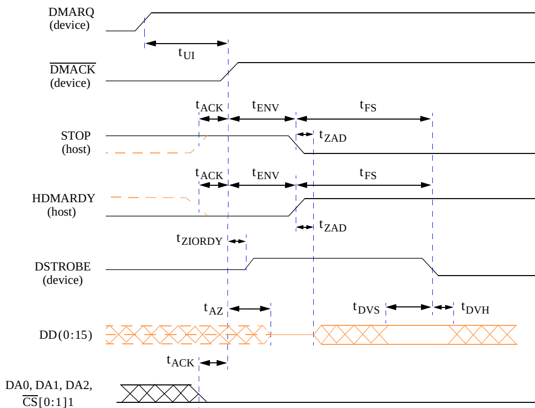
Figure 11-13 Timing Diagram—Initiating an Ultra DMA Data In Burst
