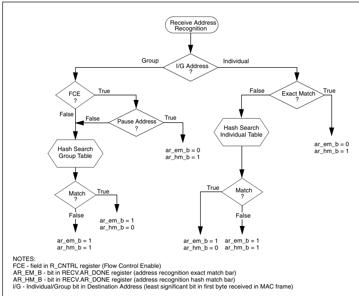
Figure 14-5 Ethernet Address Recognition - microcode decisions
