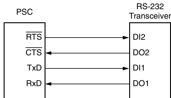
Figure 15-3 PSC/RS-232 Interface
