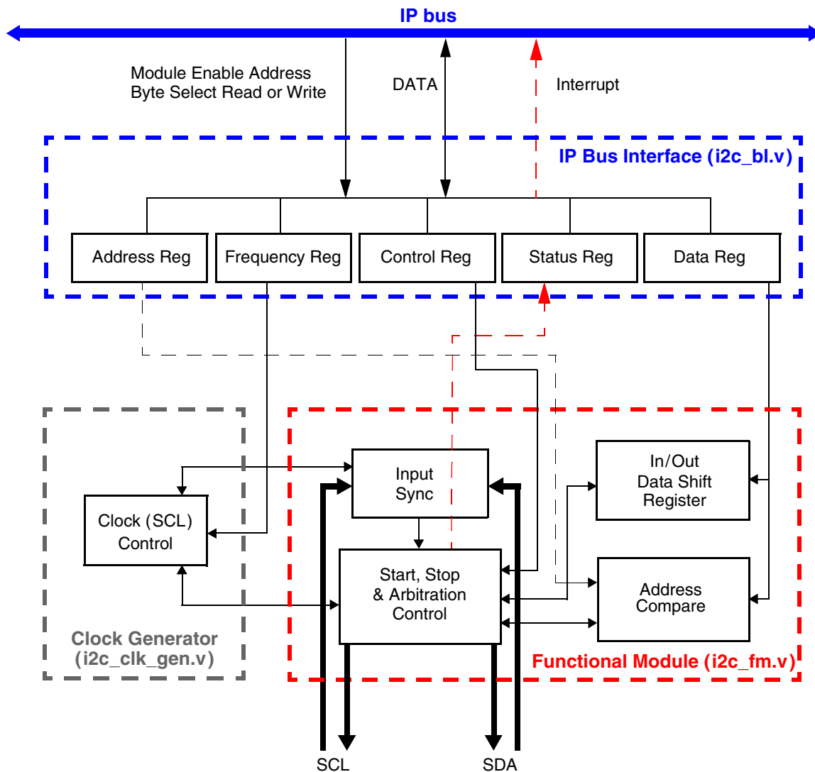
Figure 18-1 Block Diagram—I 2 C
