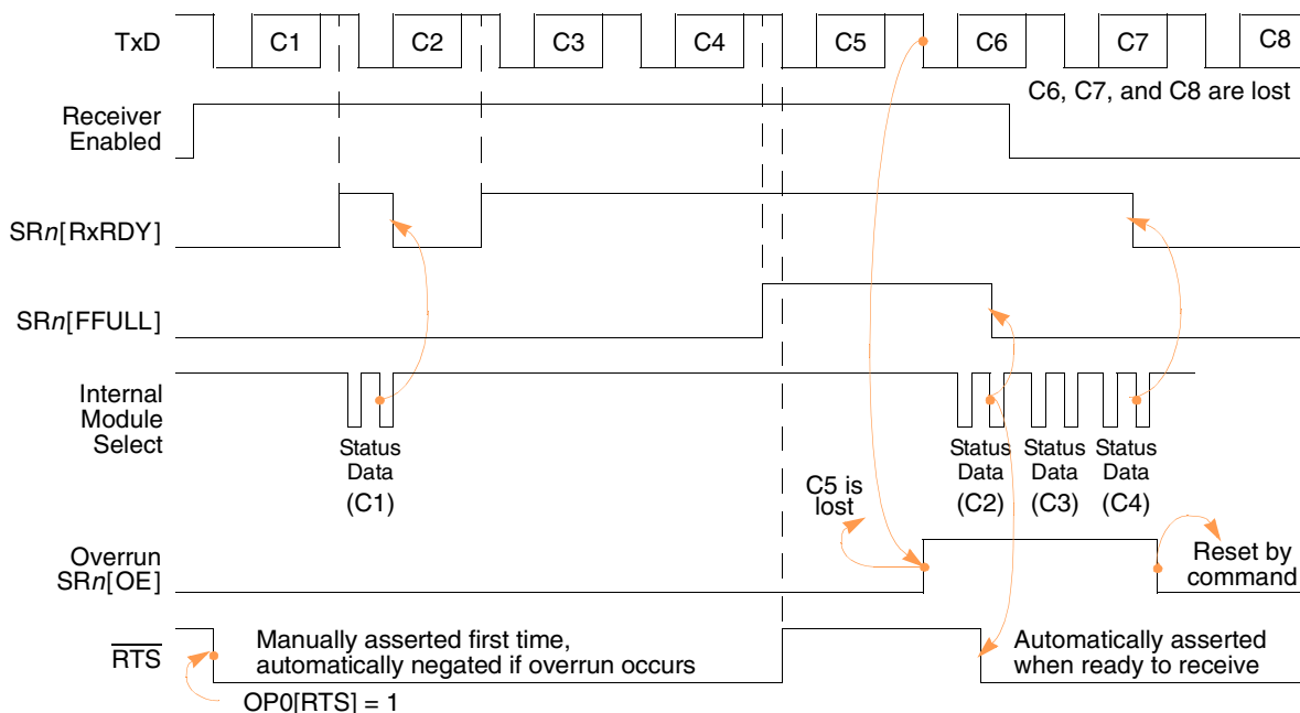
Figure 15-12 Timing Diagram—Receiver
