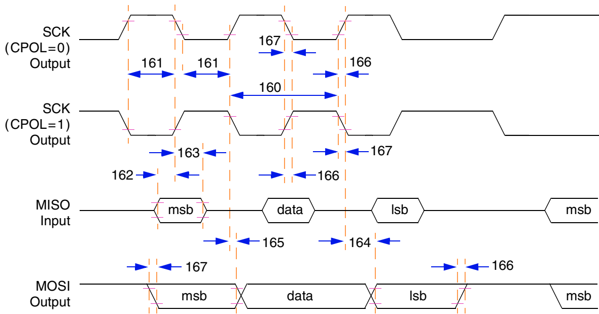
Figure A-32 Timing Diagram—SPI Master (CPHA=1)
