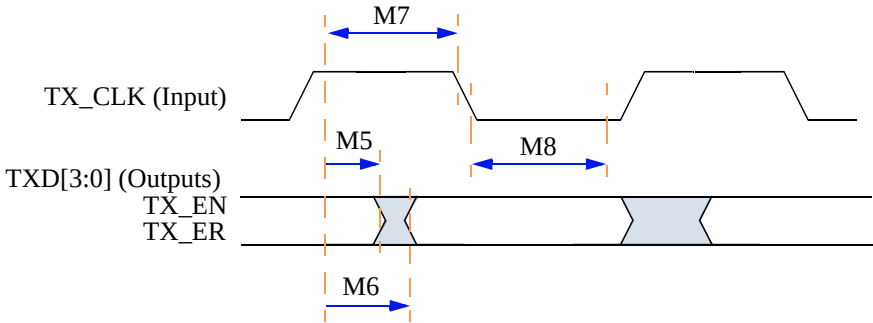
Figure A-18 Ethernet Timing Diagram—MII Tx Signal
