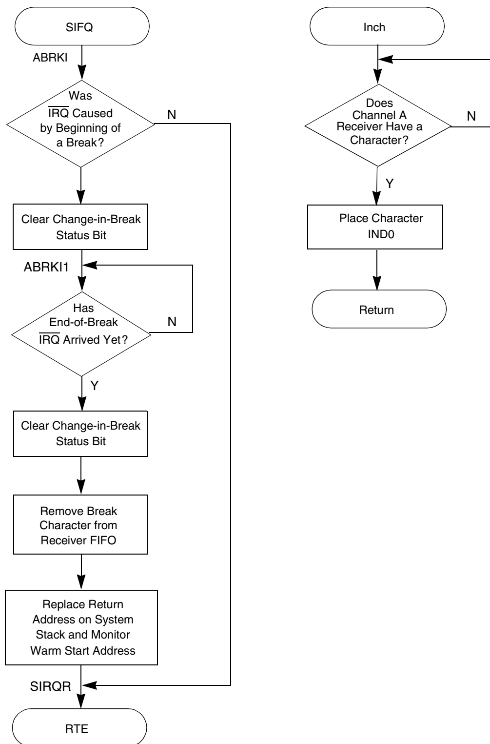
Figure 15-20 Programming Flowchart—UART Mode (sheet 4 of 5)
