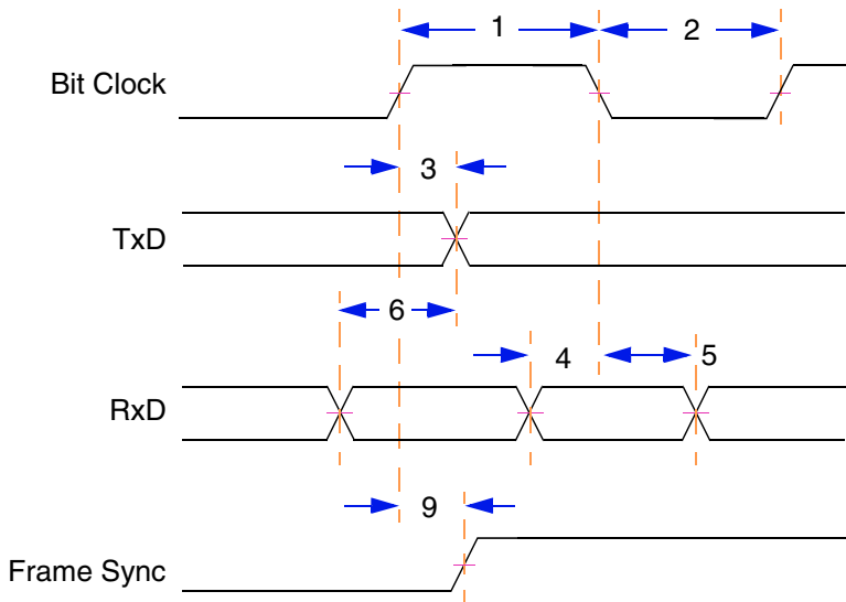
Figure A-37 Timing Diagram—AC97 Mode
