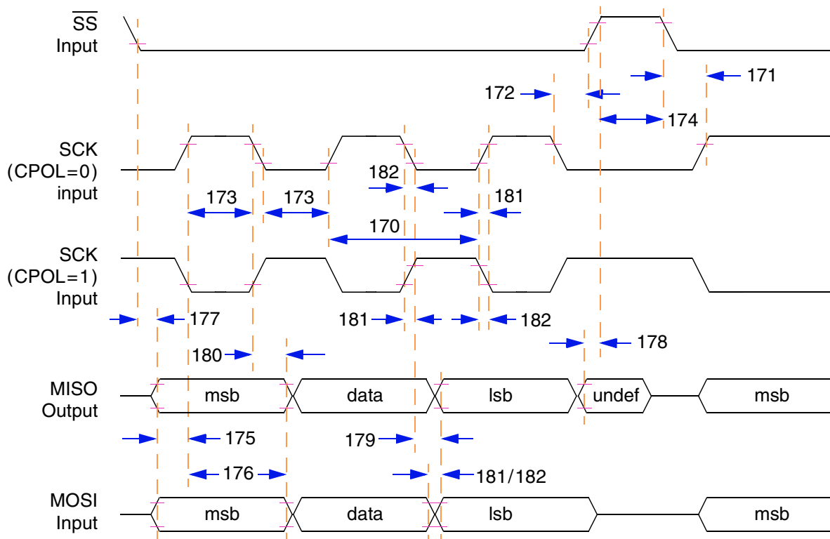
Figure A-33 Timing Diagram—SPI Slave (CPHA=0)
