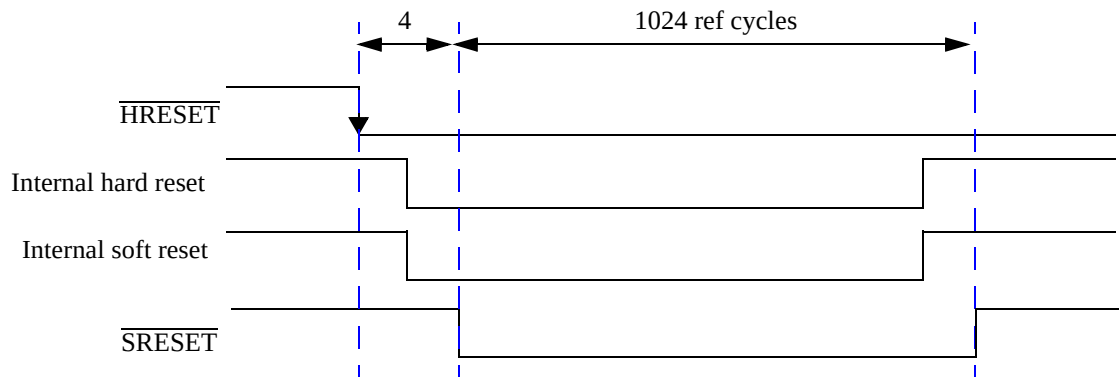
Figure 4-4 \overline{\text{HRESET}} Asserted more than 1024 Reference Clock Cycles
