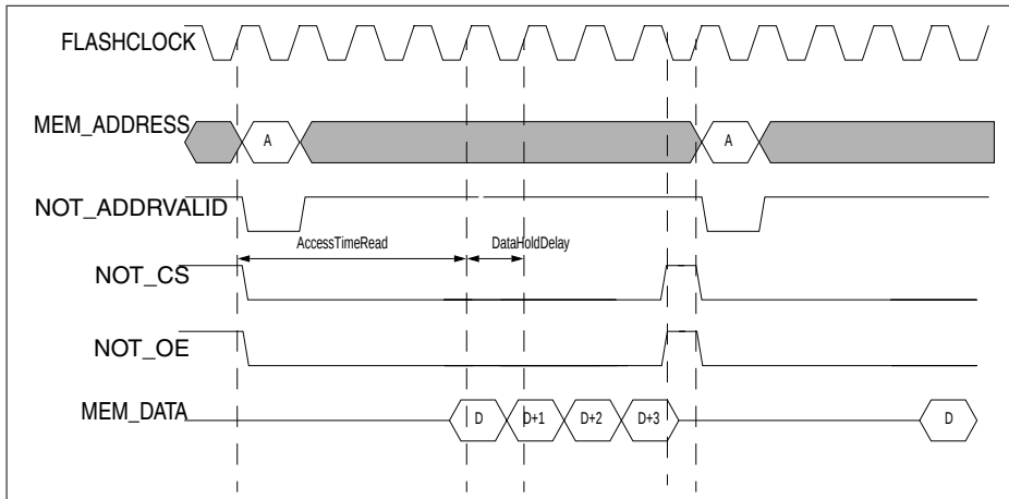
Figure 7: Synchronous burst mode flash read (burst length = 4)
