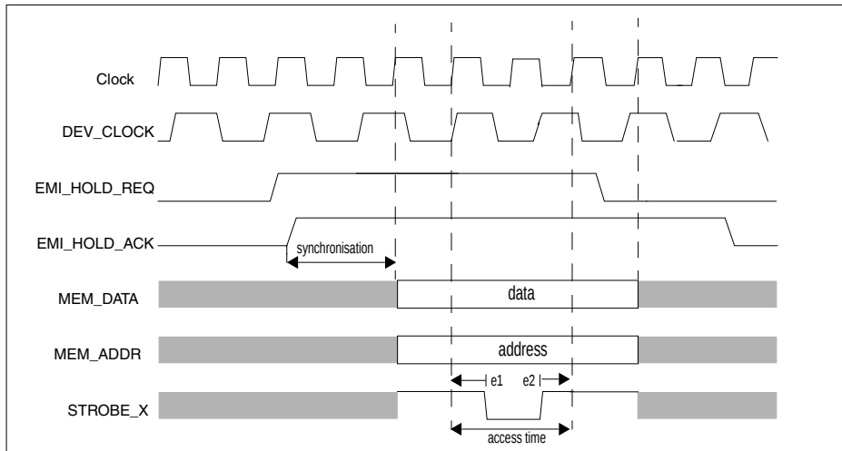
Figure 3: Signal timings
