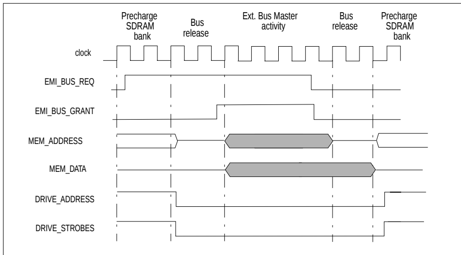
Figure 4: Signal timings
