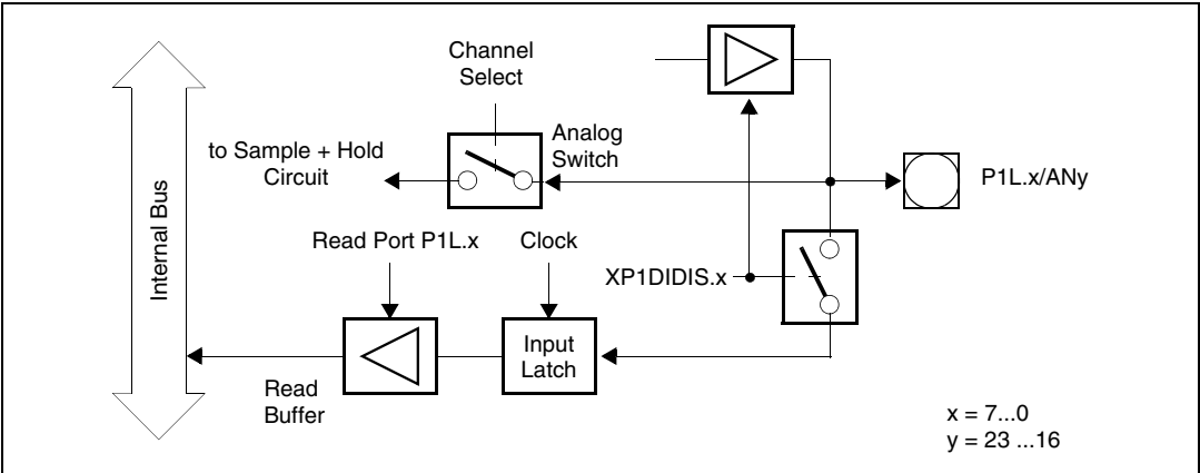
Figure 31. Block diagram of input section of a P1L pin
