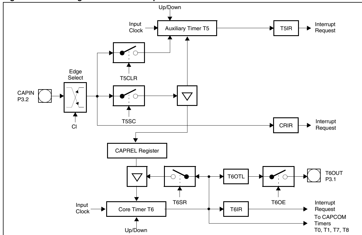
Figure 98. GPT2 register CAPREL in capture-and-reload mode
