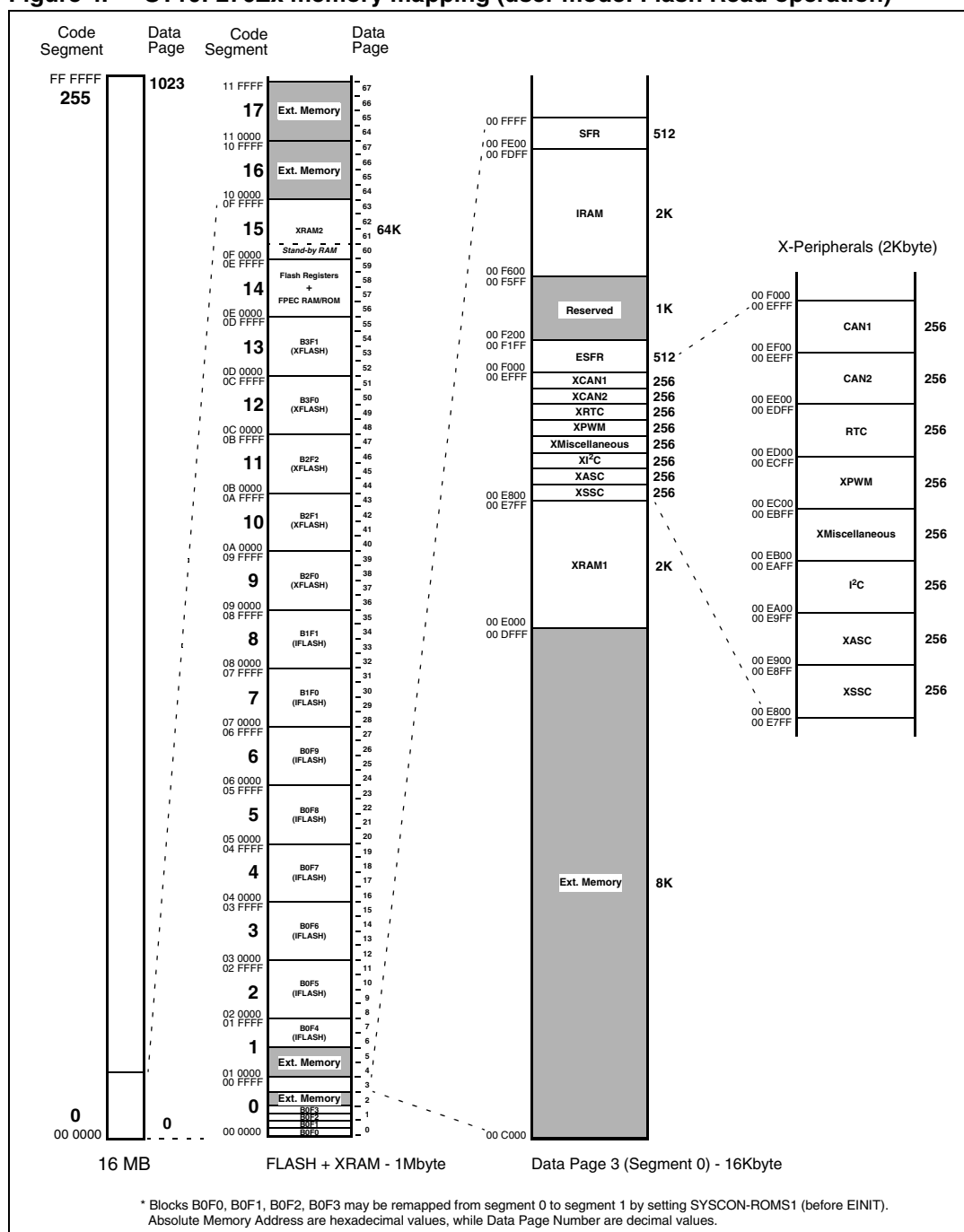
Figure 4. ST10F276Zx memory mapping (user mode: Flash Read operation)
