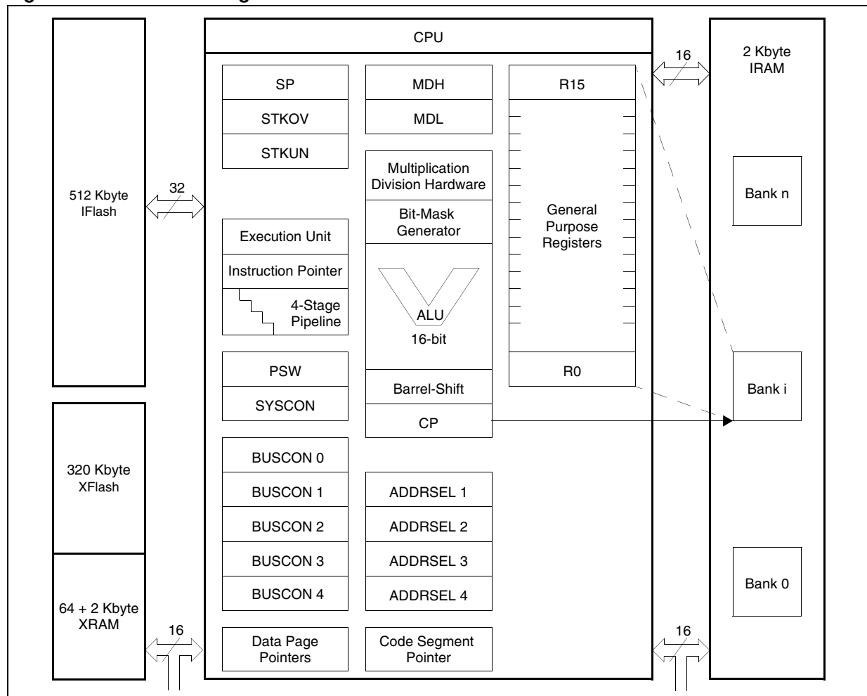
Figure 8. CPU block diagram
