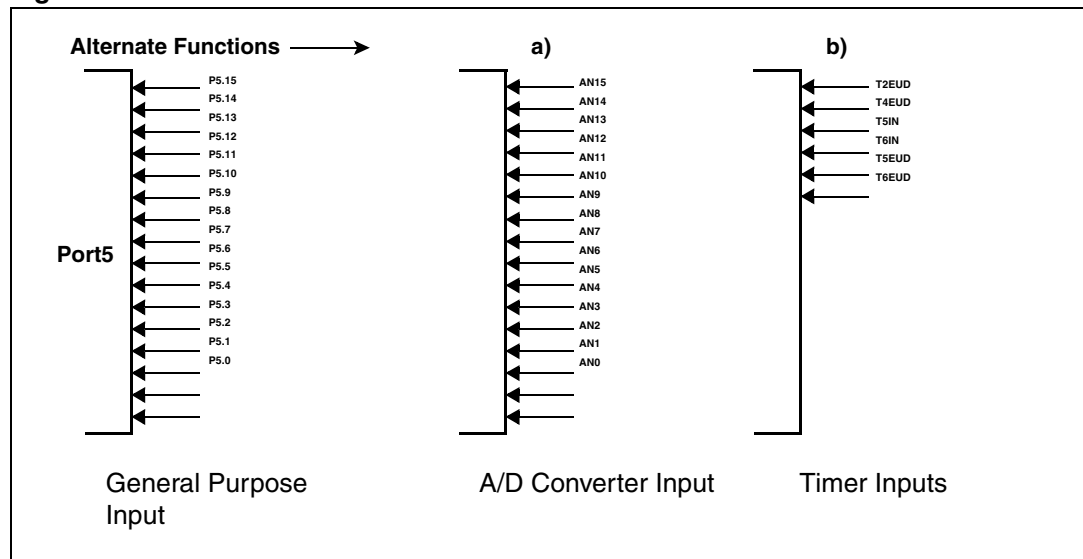
Figure 44. Port5 I/O and alternate functions
