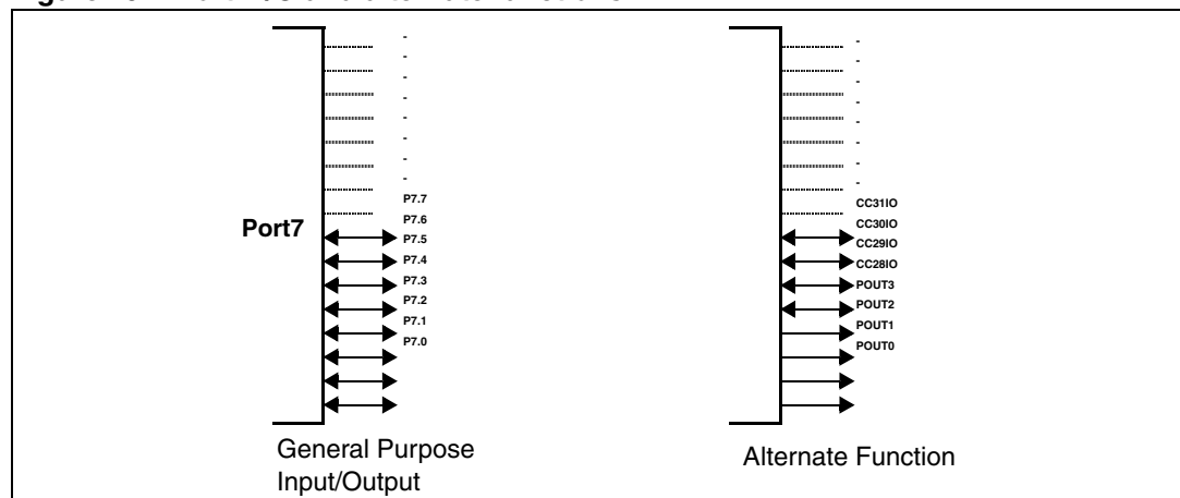
Figure 49. Port7 I/O and alternate functions
