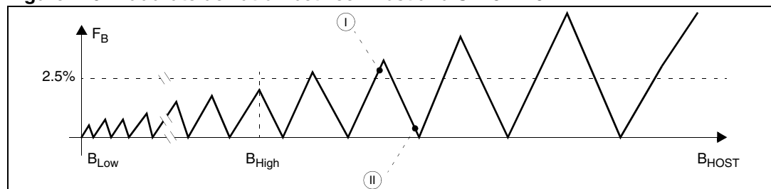
Figure 129. Baudrate deviation between host and ST10F276Zx
