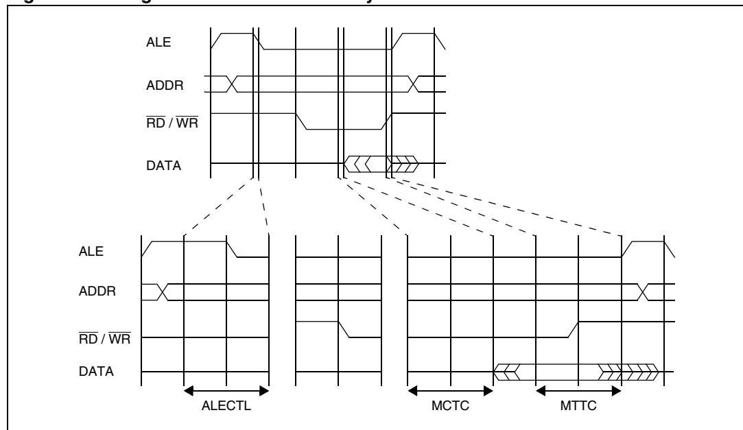
Figure 61. Programmable external bus cycle
