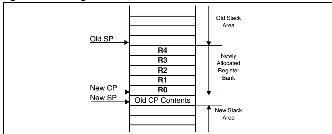
Figure 215. Local registers
