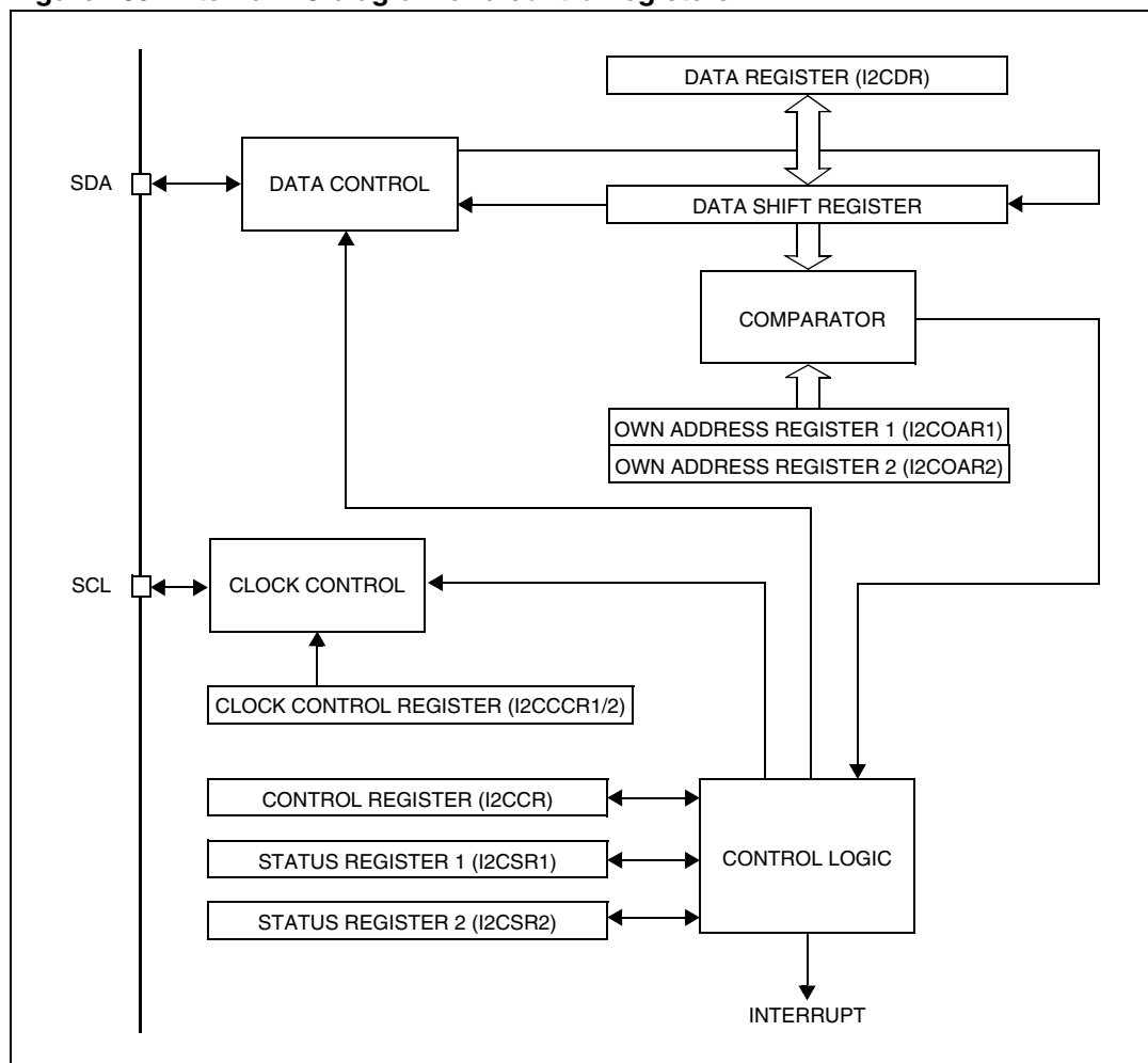
Figure 169. Internal I 2 C diagram and control registers
