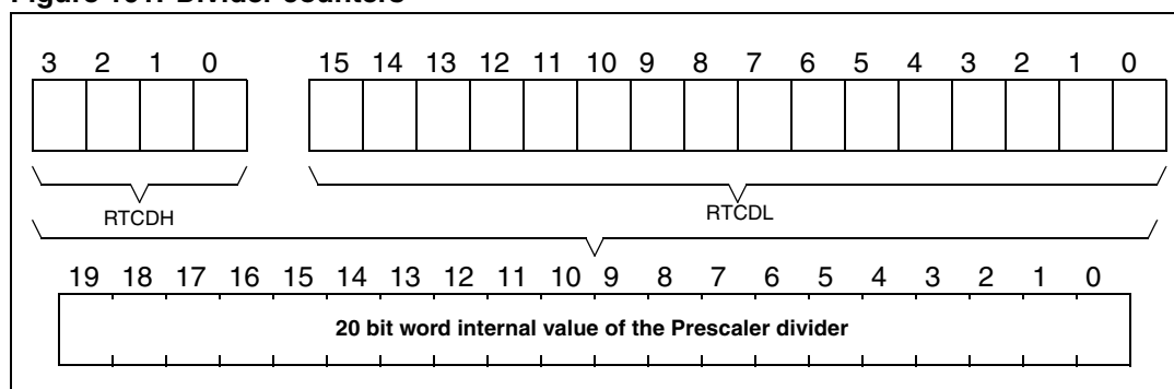
Figure 191. Divider counters
