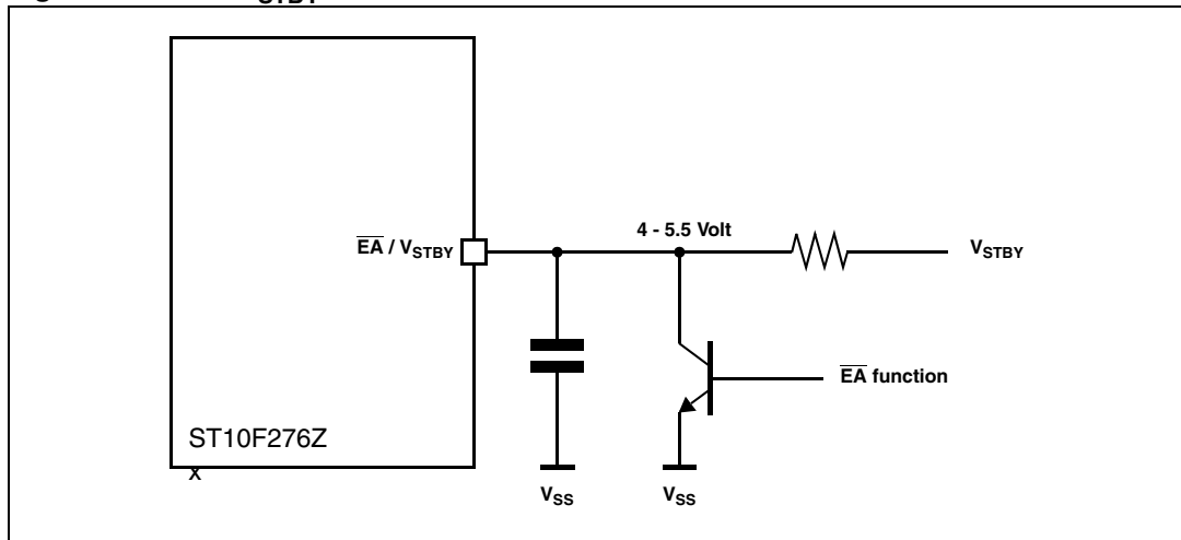
Figure 74. \overline{EA} / V_{STBY} external circuit
