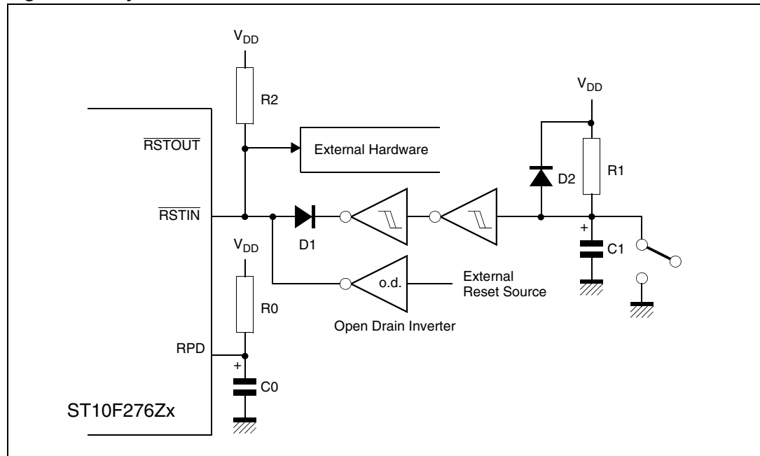
Figure 206. System reset circuit
