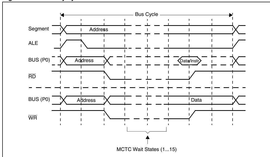
Figure 63. Memory cycle time
