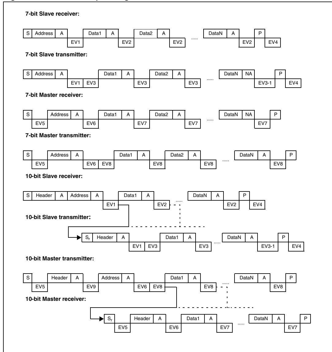
Figure 170. Transfer sequencing
