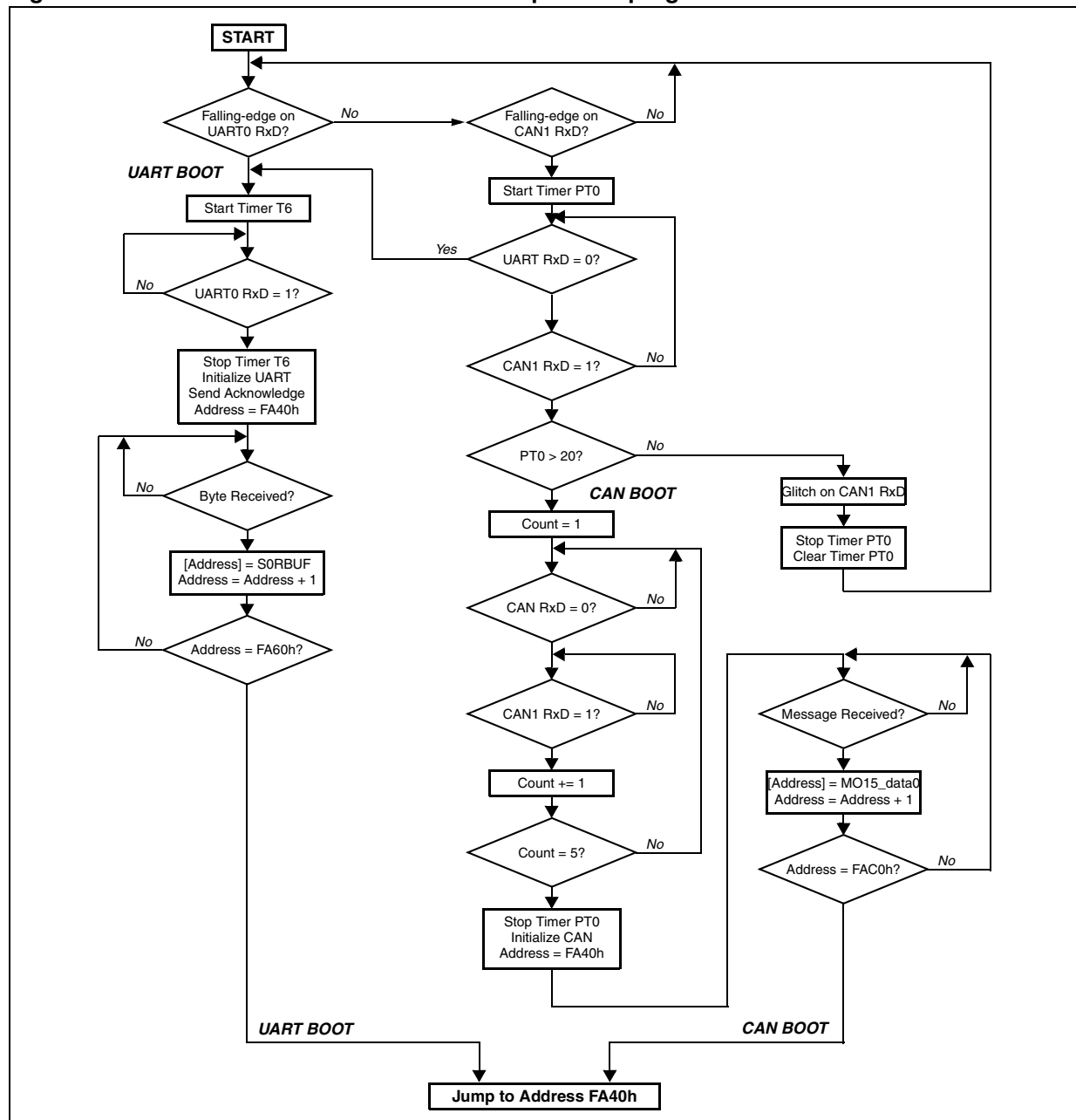
Figure 124. ST10F276Zx new standard bootstrap loader program flow
