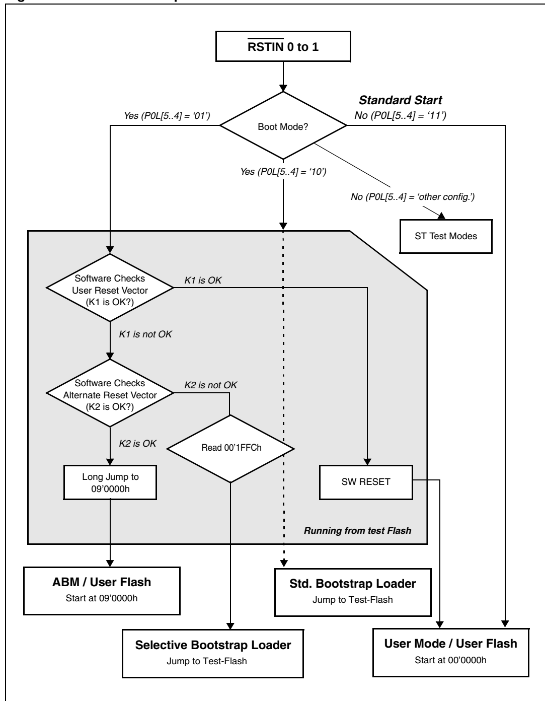
Figure 132. Reset boot sequence
