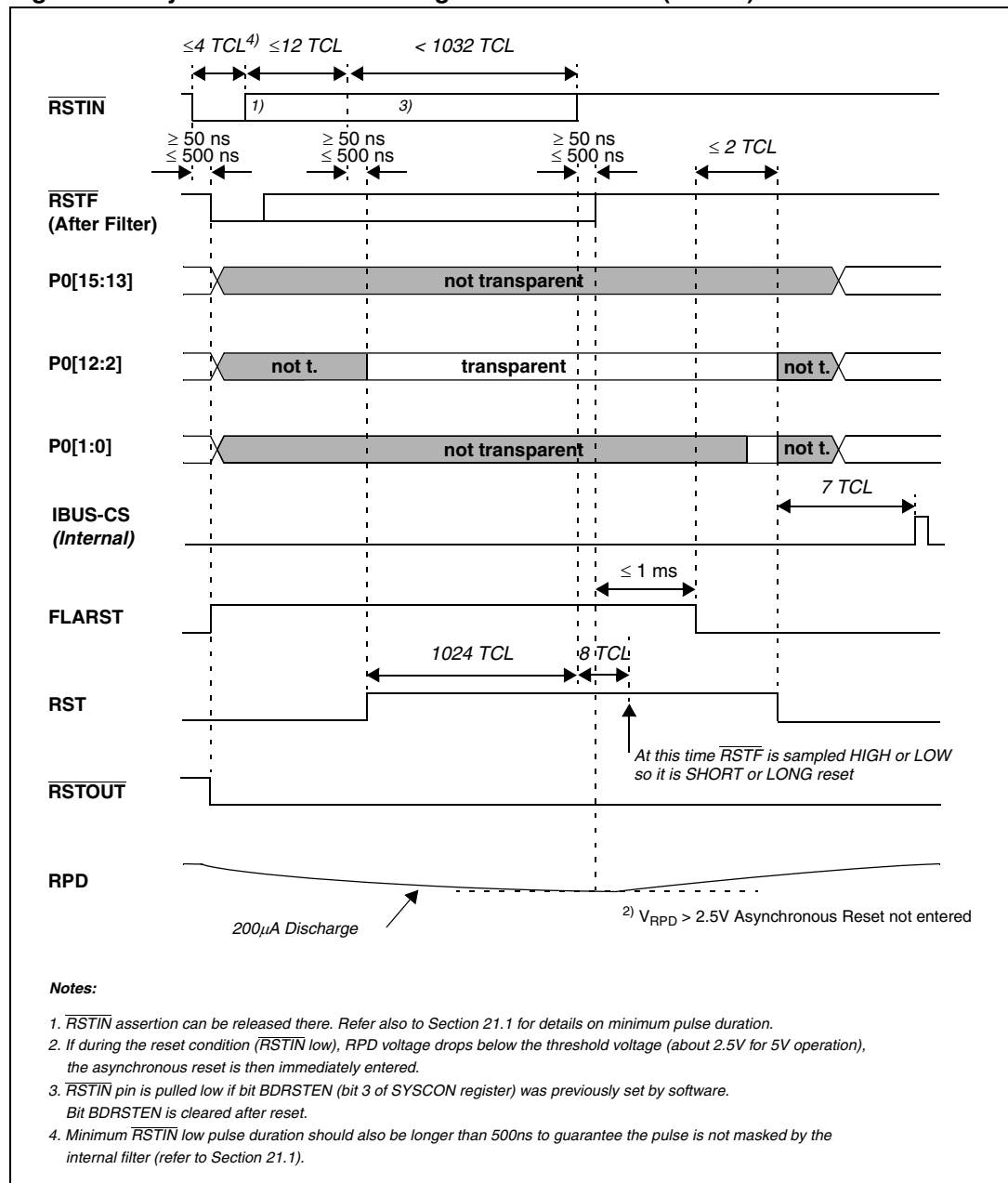
Figure 196. Synchronous short / long hardware RESET ( \overline{EA} = 1 )
