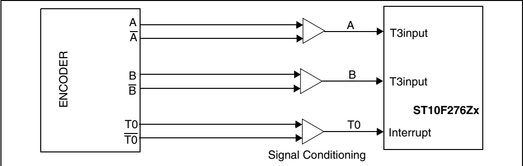
Figure 81. Connection of the encoder to the ST10F276Zx
