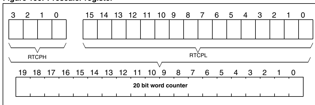
Figure 190. Prescaler register
