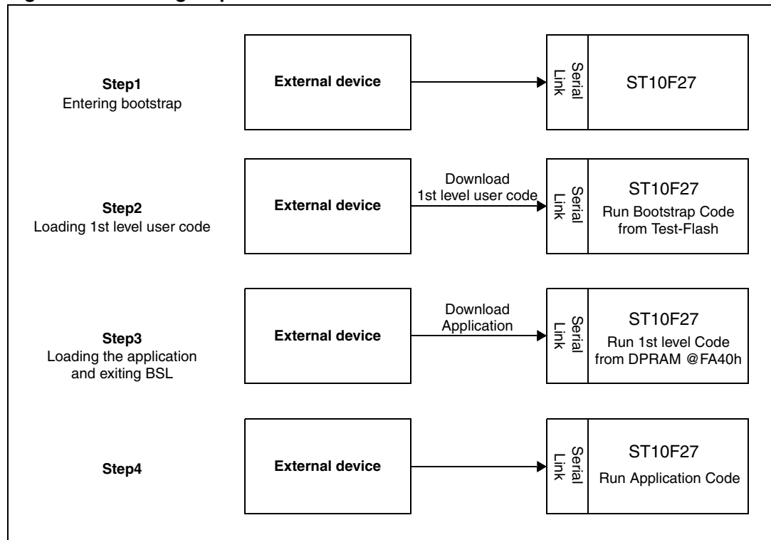
Figure 125. Booting steps for ST10F276Zx
