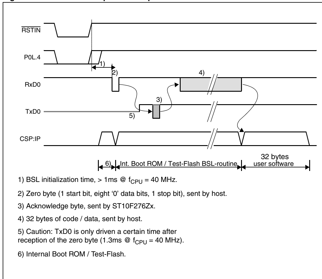
Figure 128. UART bootstrap loader sequence
