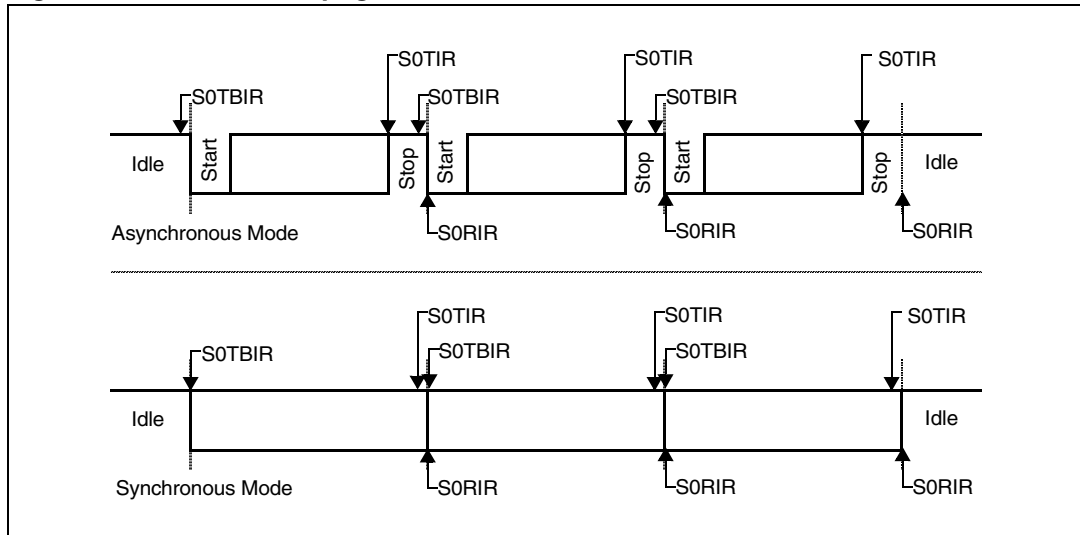
Figure 104. ASC0 interrupt generation
