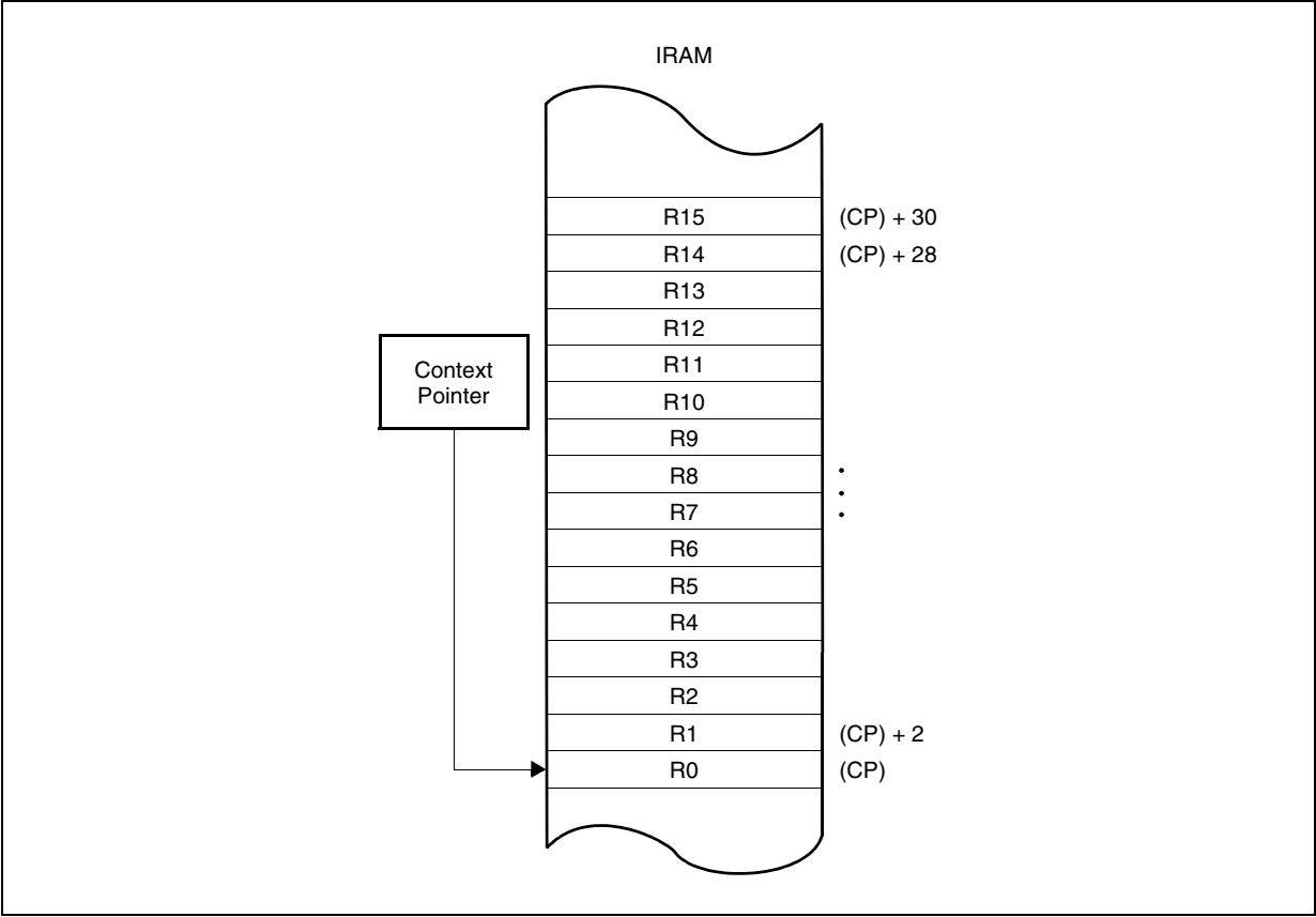
Figure 14. Register bank selection via register CP
