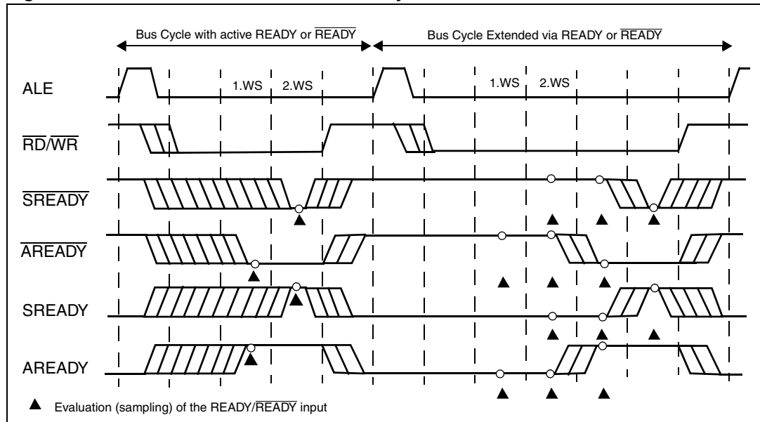
Figure 66. \text{READY}/\overline{\text{READY}} controlled bus cycles
