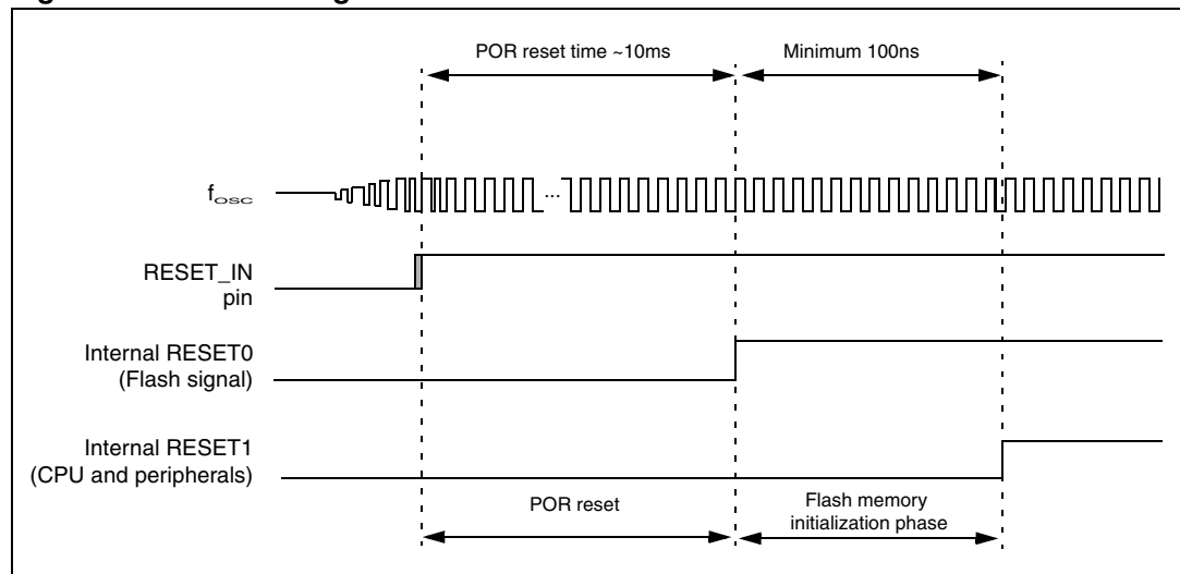
Figure 21. Reset timing
