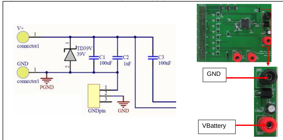
Figure 6. L9958 evaluation board power supply
