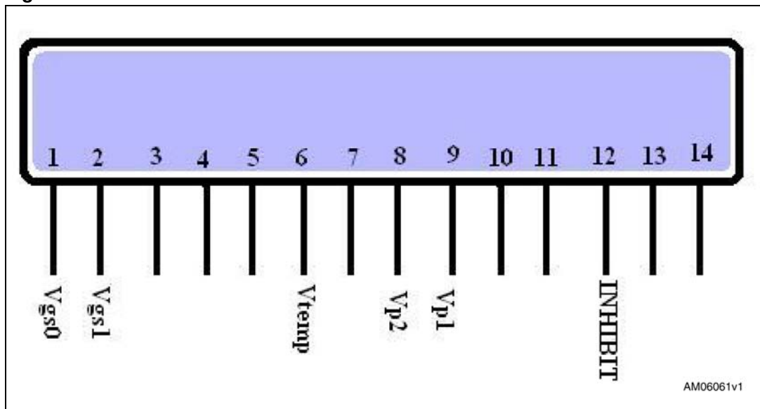
Figure 3. Pin-out scheme
