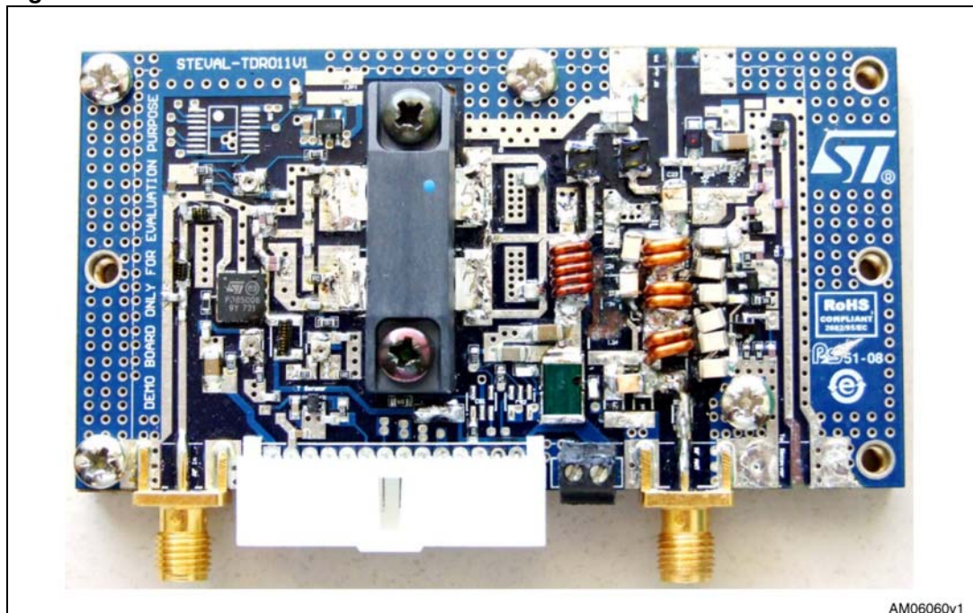
Figure 1. STEVAL-TDR011V1 demonstration board
