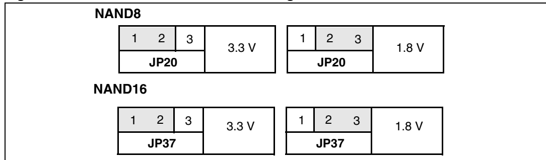
Figure 9. SPEAr NAND8/16 Flash I/O voltage selector
