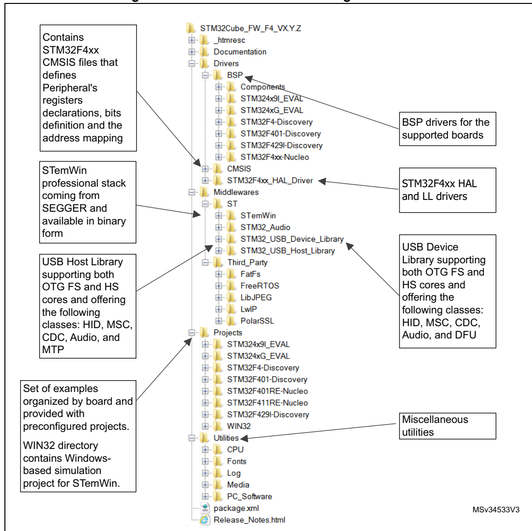
Figure 3. STM32CubeF4 MCU Package structure
