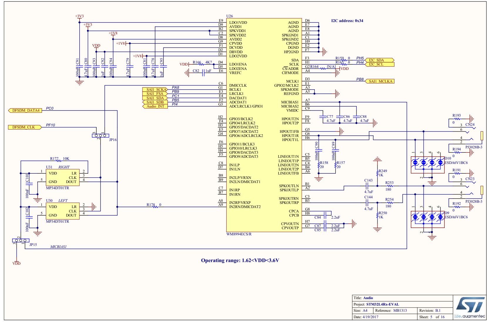
Figure 27. Audio codec device
