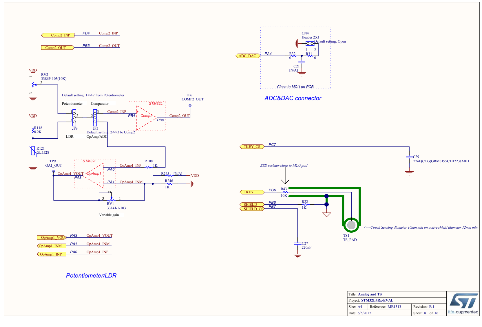
Figure 30. Analog input and output and touch-sensing device
