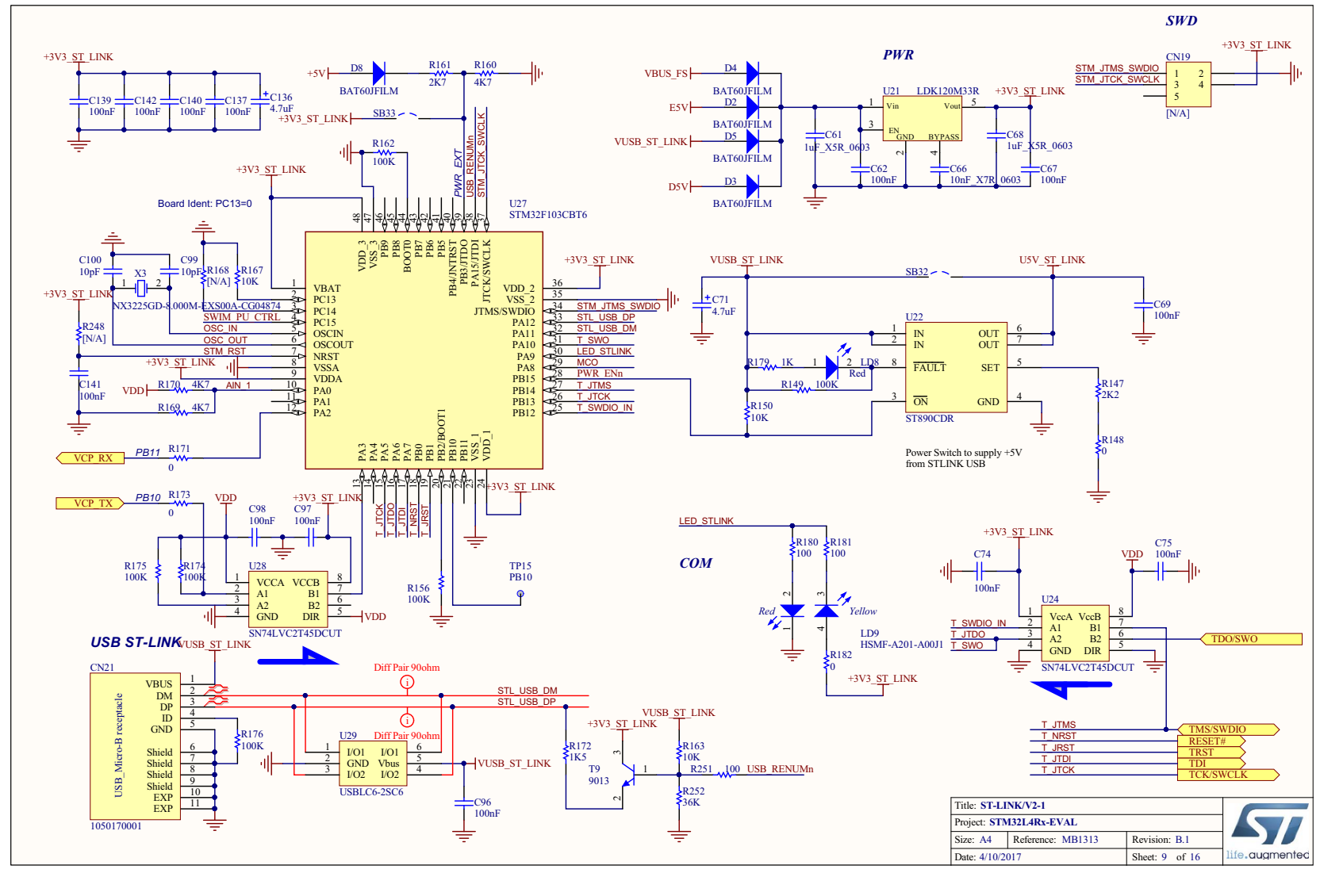
Figure 31. ST-LINK/V2-1
