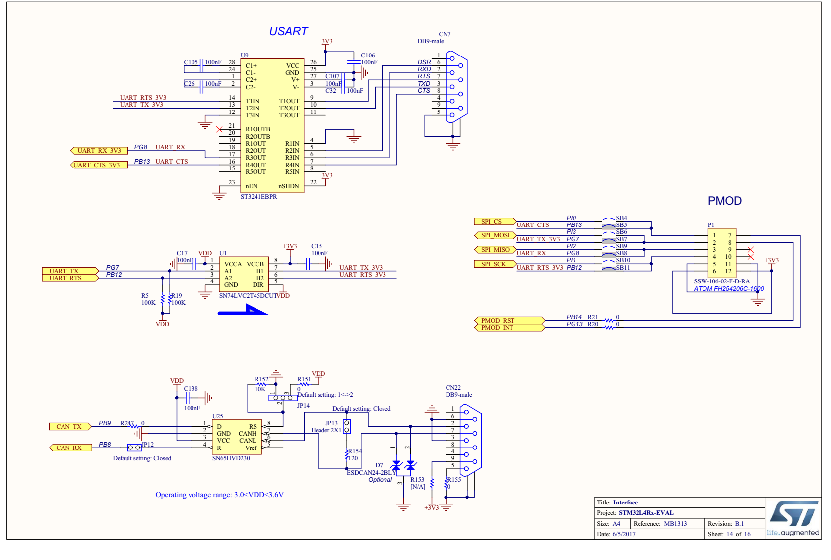
Figure 36. USART, CAN transceiver and PMOD connector
