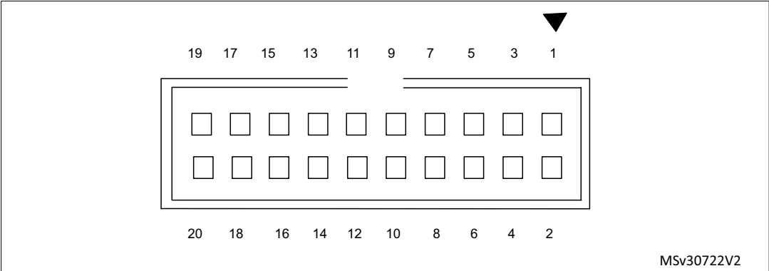
Figure 19. JTAG/SWD debugging connector CN17 (Top view)
