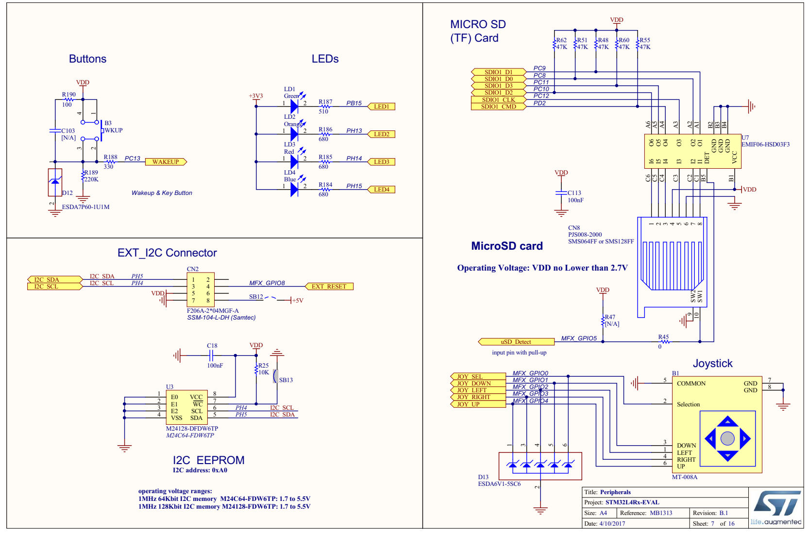
Figure 29. Physical control peripherals, microSD card and EEPROM
