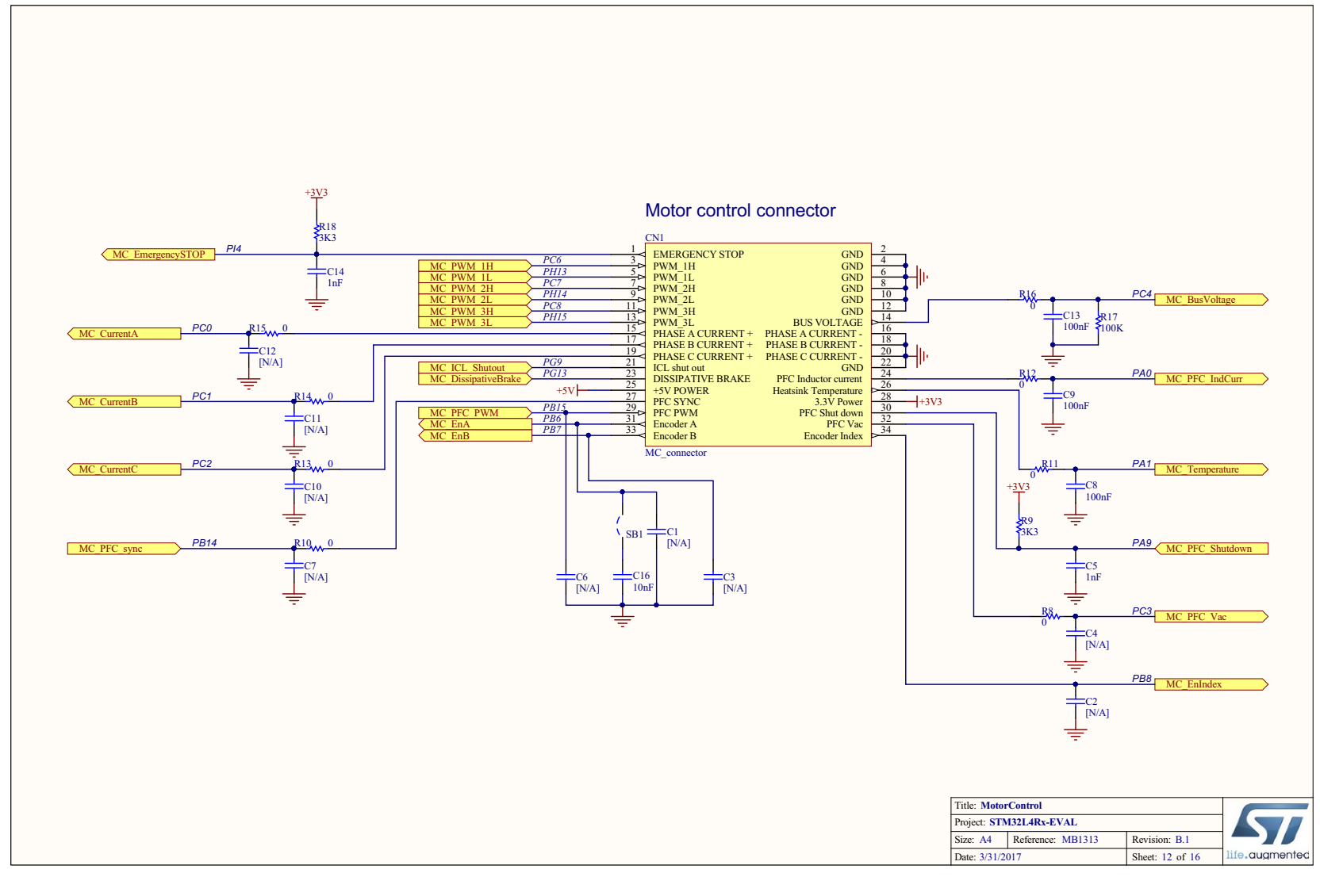
Figure 34. Motor-control connector
