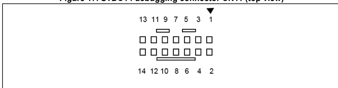
Figure 17. STDC14 debugging connector CN11 (top view)
