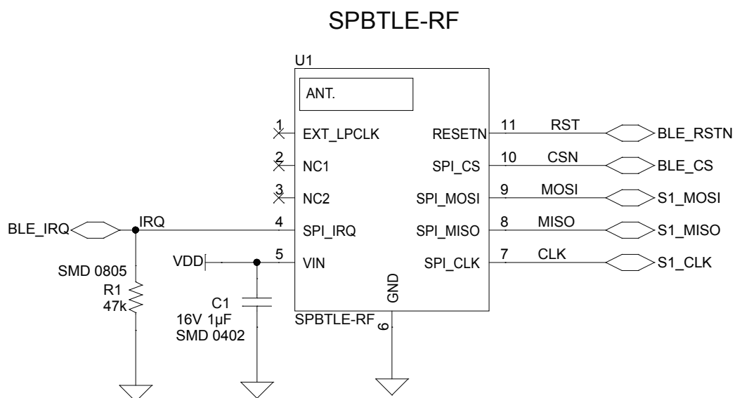
Figure 8. STEVAL-FCU001V1 – circuit schematic (1 of 4)
