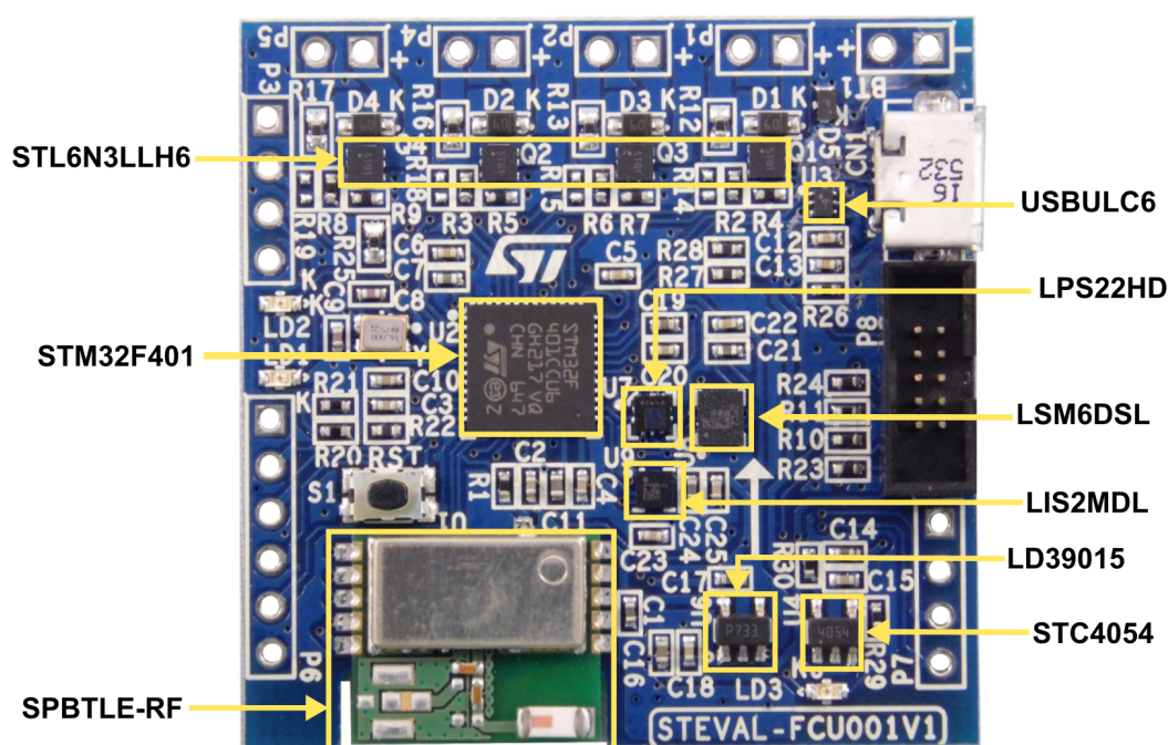
Figure 4. STEVAL-FCU001V1 evaluation board components
