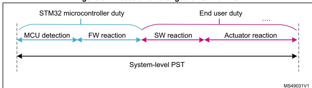
Figure 5. Allocation and target for STM32 PST
