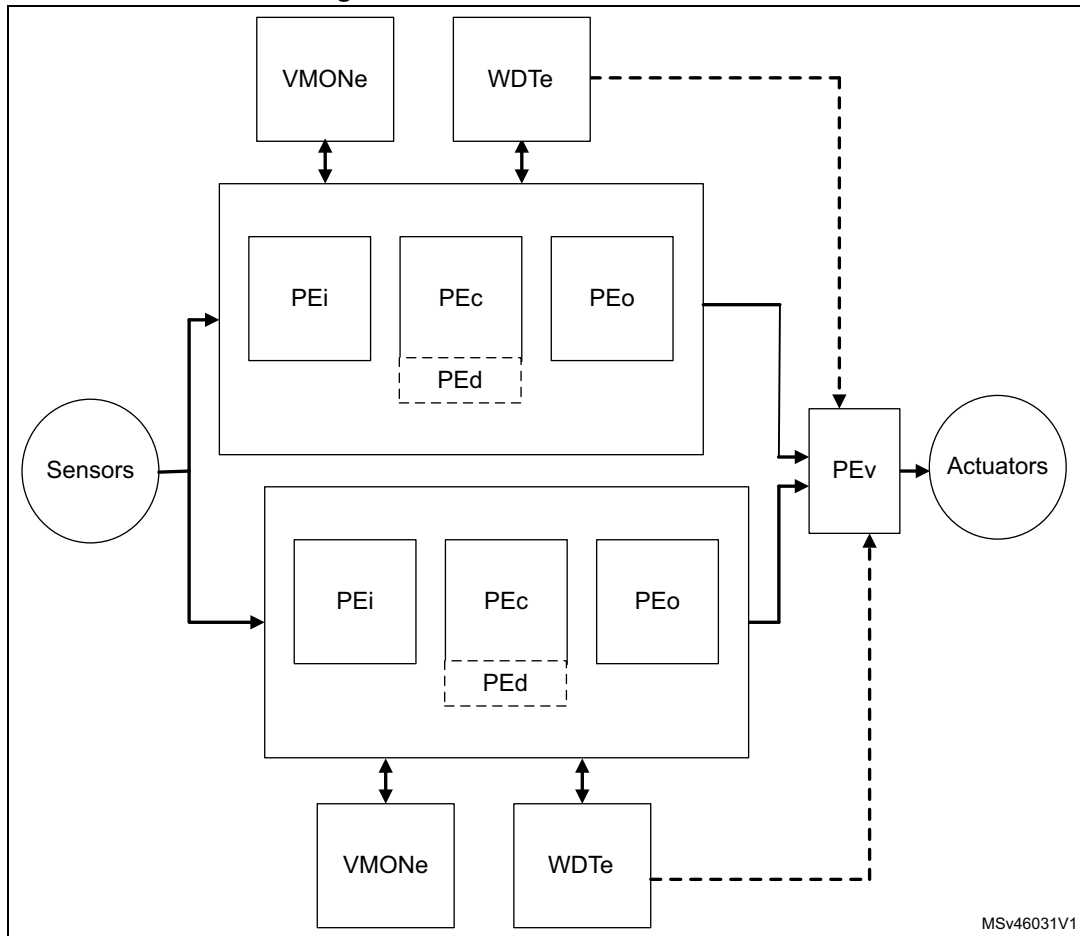
Figure 4. 1002 reference architecture
