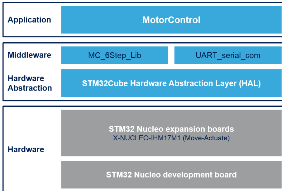
Figure 2. X-CUBE-SPN17 architecture
