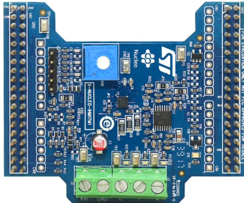
Figure 5. X-NUCLEO-IHM17M1 expansion board
