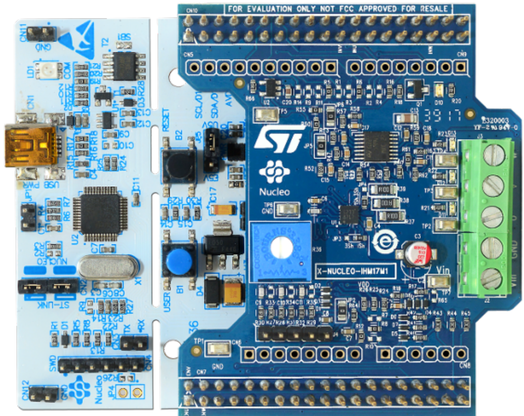
Figure 6. STM32 Nucleo board plus X-Nucleo-IHM17M1 expansion board
