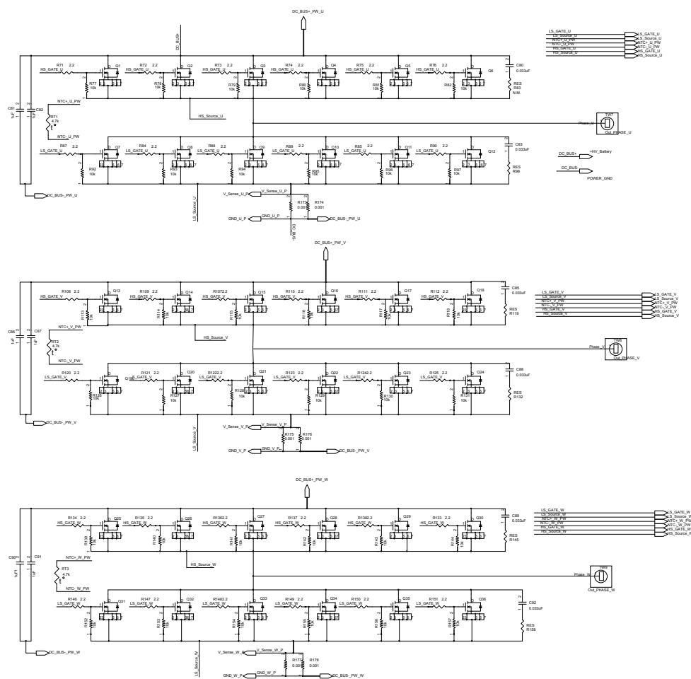
Figure 13. STEVAL-CTM004V1 power board schematic
