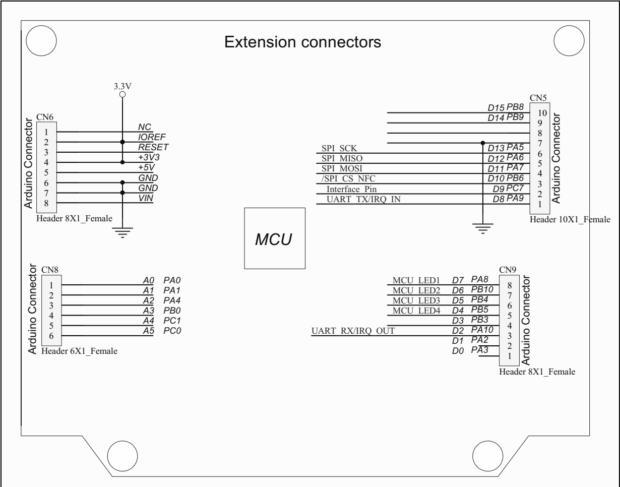
Figure 4. Nucleo connectors
