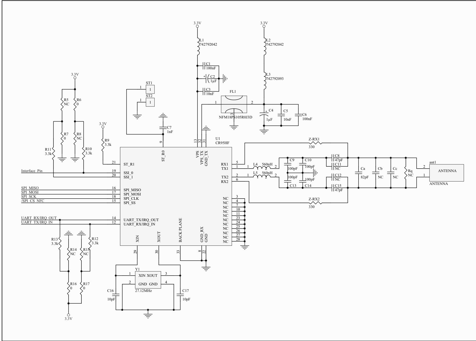
Figure 6. ST25R95HF and matching circuitry
