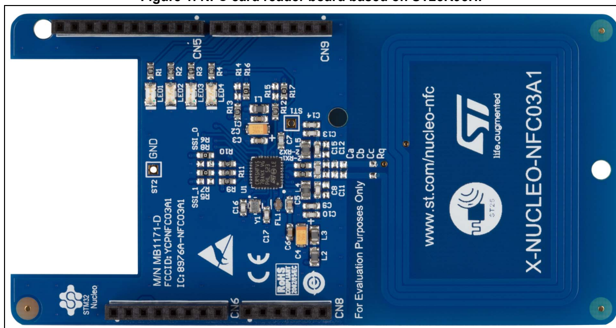
Figure 1. NFC card reader board based on ST25R95HF
