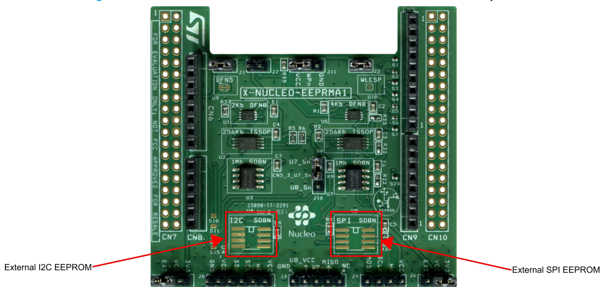
Figure 6. I 2 C and SPI EEPROM soldered on the X-NUCLEO-EEPRMA1 expansion board
