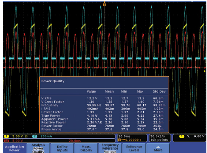
Figure 12. DPOxPWR Power Quality Measurements.
