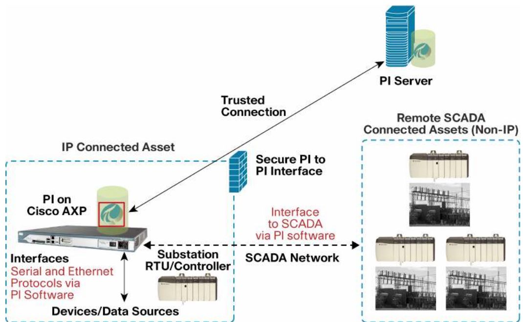
Figure 1. Supervisory Control and Data Acquisition (SCADA) via a Cisco Router with PI Software from OSIsoft
