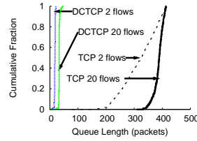
Figure 14: Queue length CDF (1Gbps)
