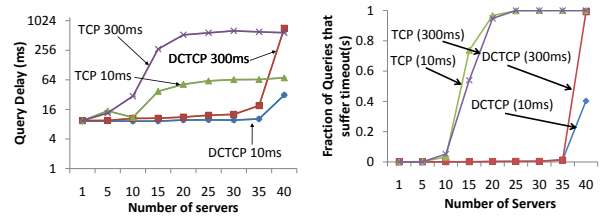
Figure 19: DCTCP performs better than TCP and then converges at 35 senders (log scale on Y axis; 90% confidence intervals for the means are too small to be visible).
