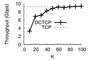
Figure 15: Throughput (10Gbps)
