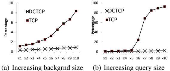
Figure 27: Fraction of queries that suffer at least one timeout
