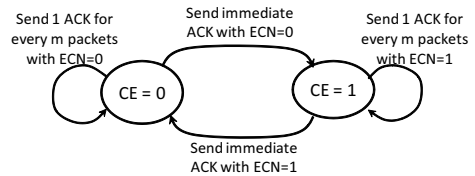
Figure 11: Two state ACK generation state machine.
