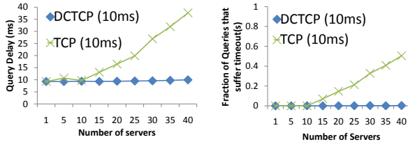
Figure 20: Many-to-one: With dynamic buffering, DCTCP does not suffer problems at even high load.
