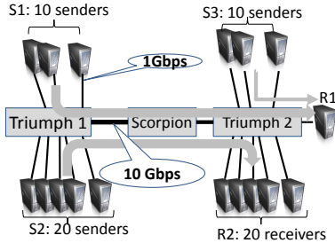
Figure 18: Multi-hop topology
