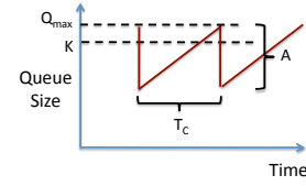
Figure 12: DCTCP queue size sawtooth parameters.
