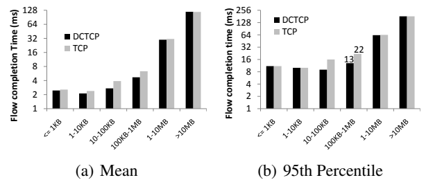
Figure 23: Completion time of background traffic. Note the log scale on the Y axis.
