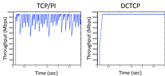
Figure 13: DCTCP and TCP/PI with two long-lived flows.
