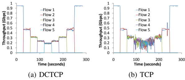
Figure 17: Convergence test
