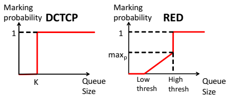
Figure 10: DCTCP’s AQM scheme is a variant of RED: Low and High marking thresholds are equal, and marking is based on the instantaneous queue length.
