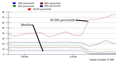
Figure 8: Response time percentiles for a production application having the incast traffic pattern. Forwarded requests were jittered (deliberately delayed) over a 10 ms window until 8:30am, when jittering was switched off. The 95th and lower percentiles drop 10x, while the 99.9th percentile doubles.
