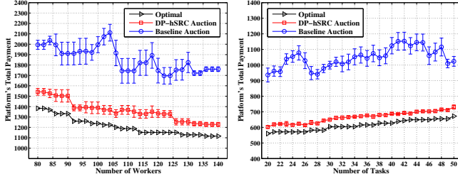
Figure 1. Platform's total payment under setting I
