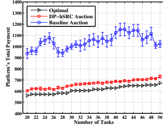
Figure 2. Platform's total payment under setting II
