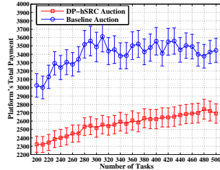
Figure 4. Platform's total payment under setting IV
