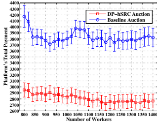
Figure 3. Platform's total payment under setting III
