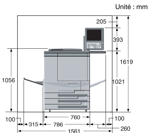
Machine + OC-506 + OT-502
