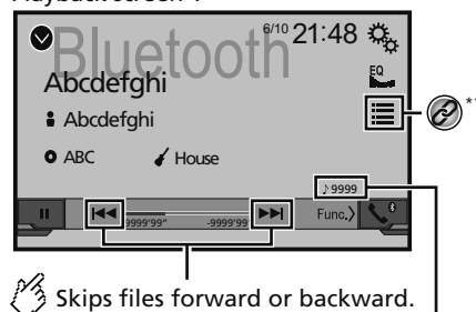
Playback screen 1
