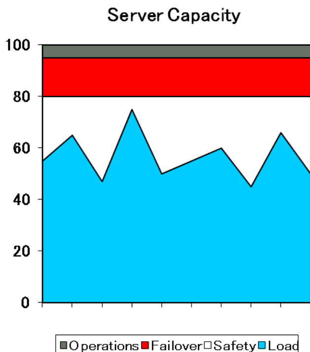
Figure 8. CPU Capacity
