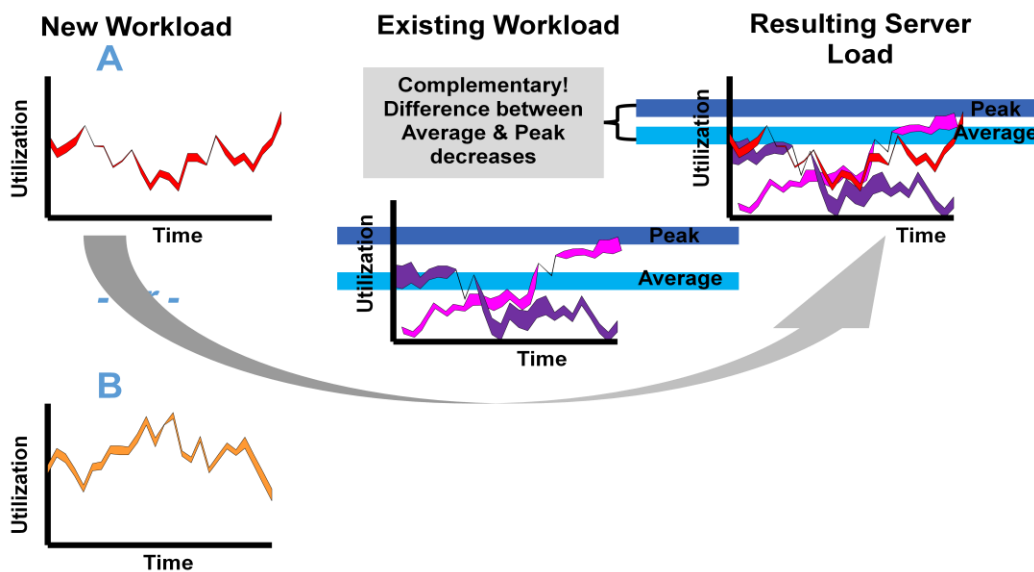
Figure 9. Complementary Workloads
