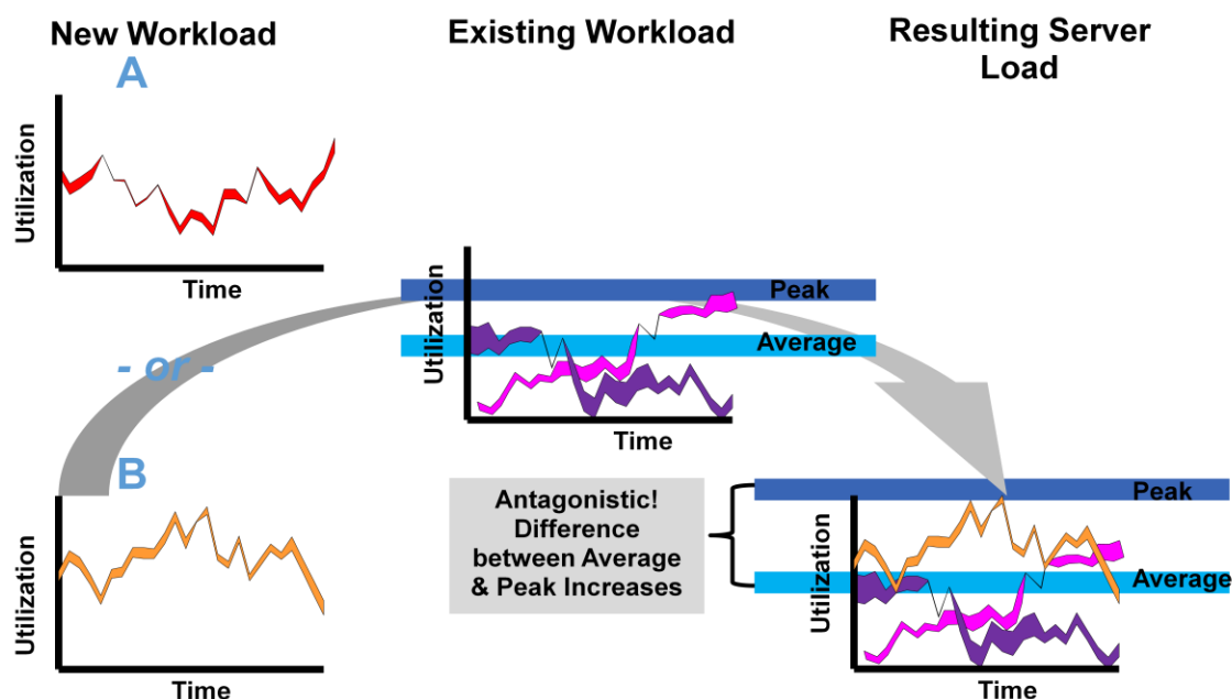
Figure 10. Antagonistic Workloads
