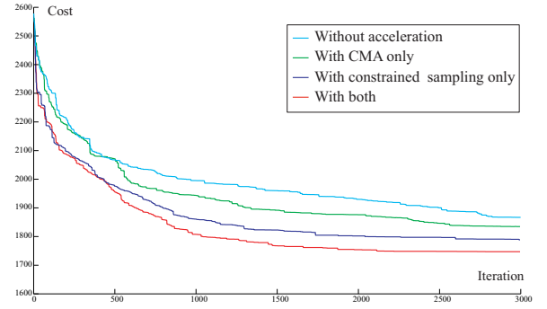
Figure 6: Optimization acceleration.
