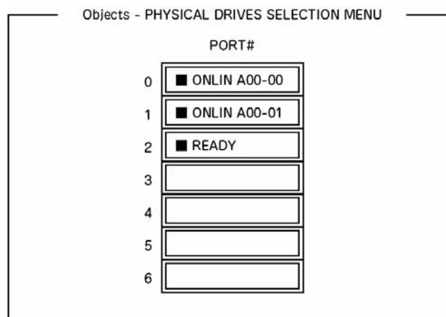
Illustration 43: Écran Objects - Physical Drive Selection Menu
