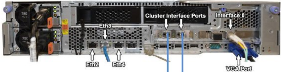
3650M4 Master above and Data Node below
