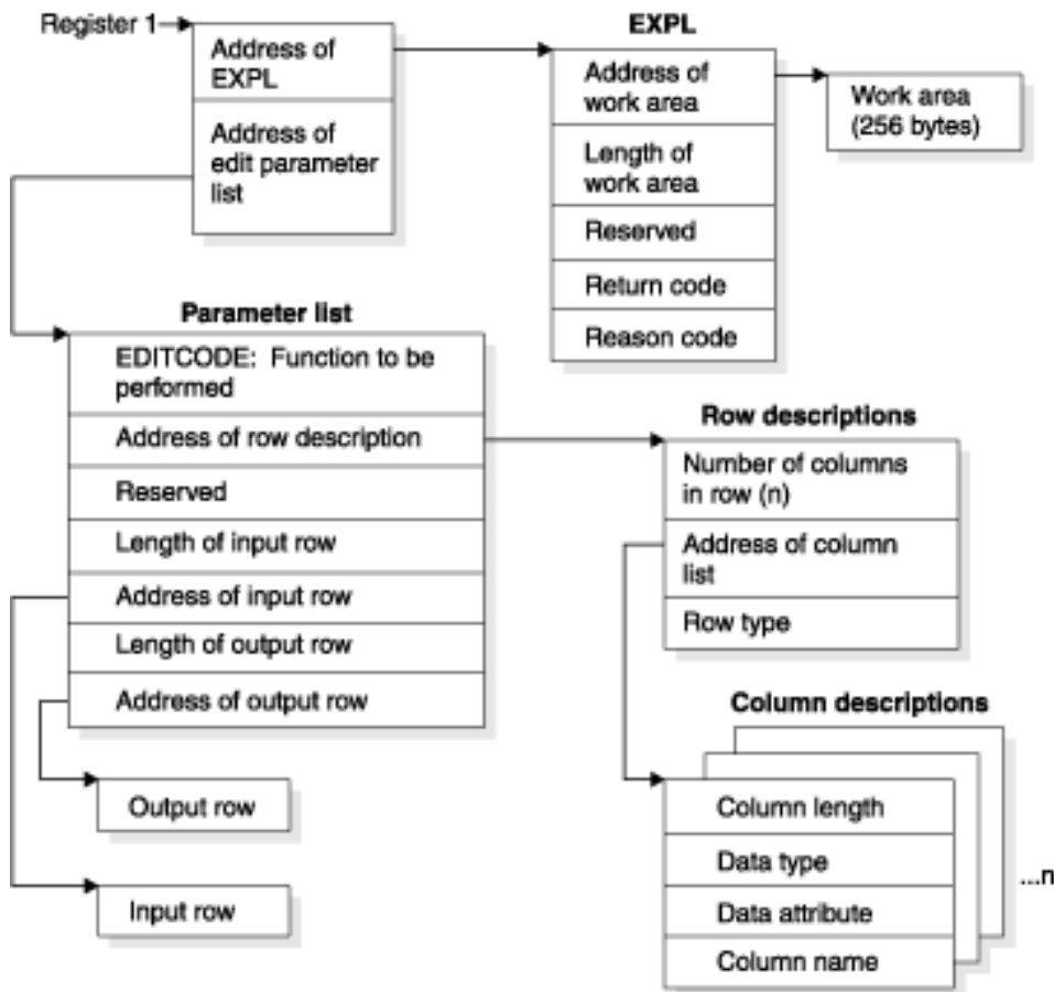
Figure 68. How the edit exit parameter list points to row information
