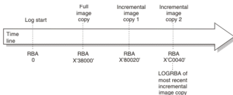
Figure 43. Overview of Db2 recovery from COPY utility
