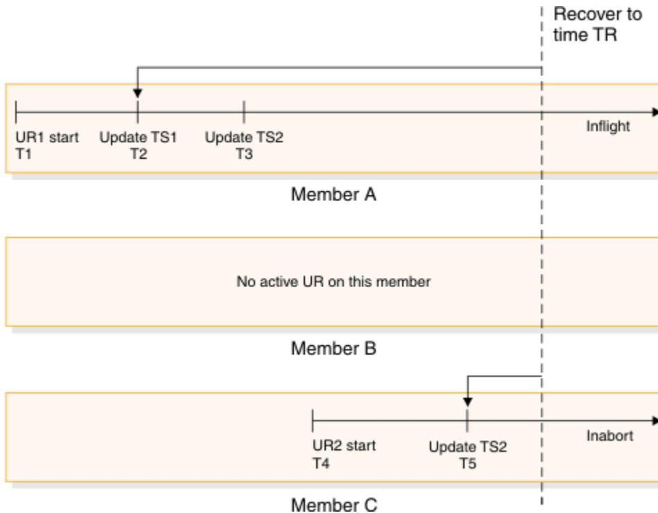
Figure 47. Using the RECOVER TOLOGPOINT option in a data sharing system
