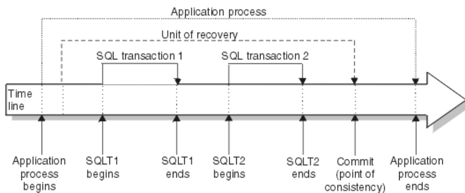
Figure 35. A unit of recovery within an application process
