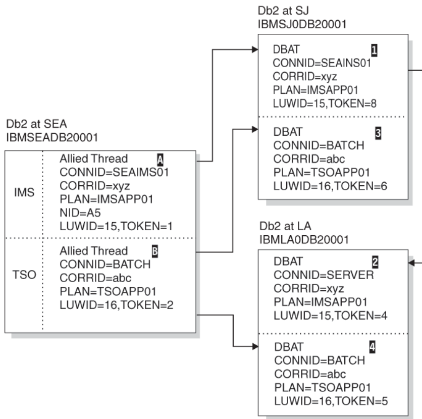
Figure 61. Resolution of indoubt threads
