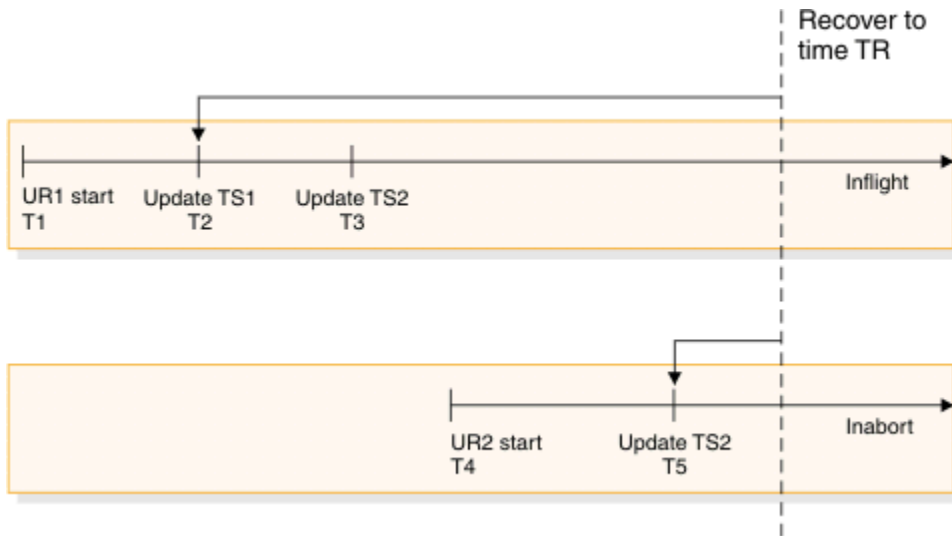
Figure 48. Using the RECOVER TOLOGPOINT option in a non-data sharing system
