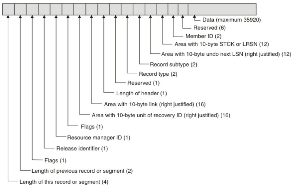
Figure 65. 10-byte format of a Db2 recovery log record
