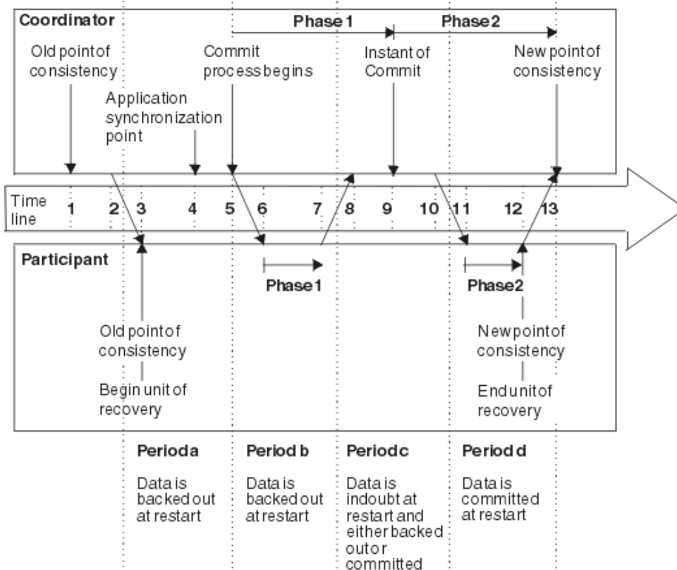
Figure 39. Time line illustrating a commit that is coordinated with another subsystem
