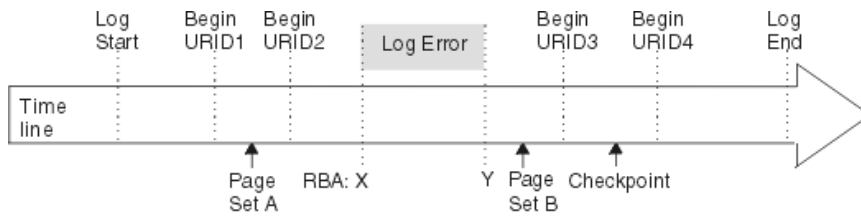
Figure 54. Illustration of failure during forward-log recovery
