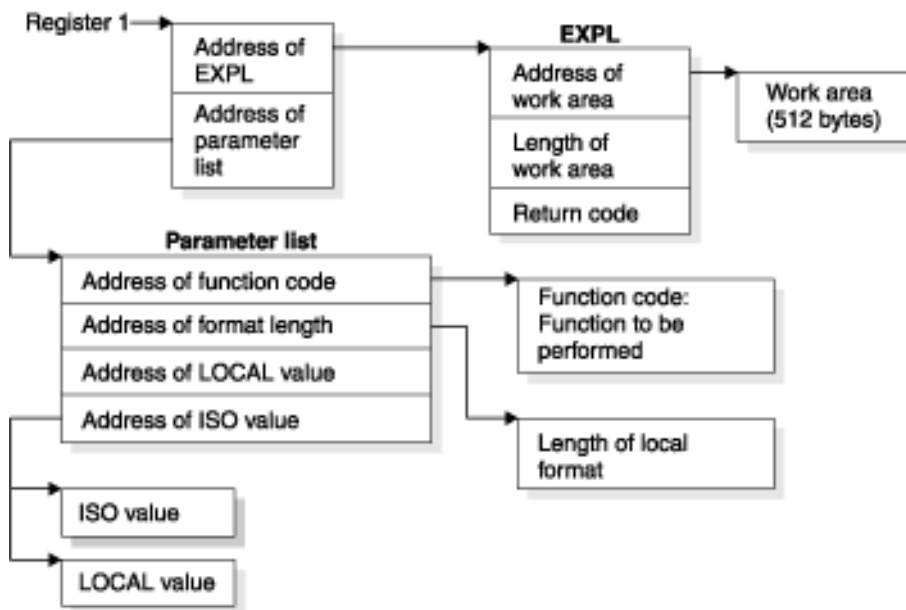
Figure 70. How a date or time parameter list points to other information
