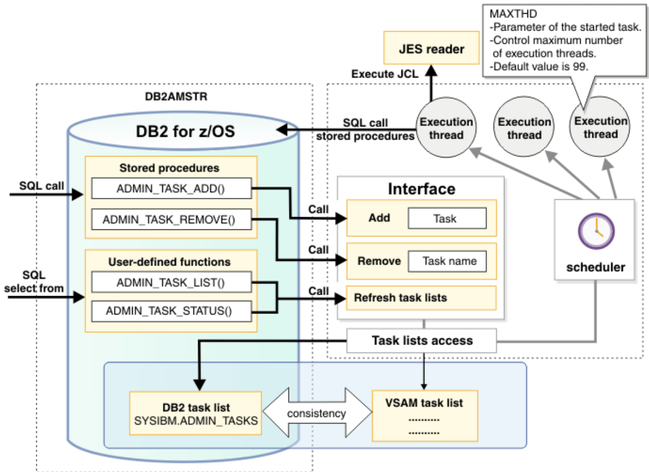
Figure 24. Multi-threading in the administrative task scheduler
