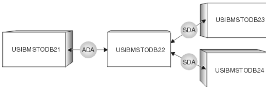
Figure 25. Example of a Db2 transaction that involves four sites
