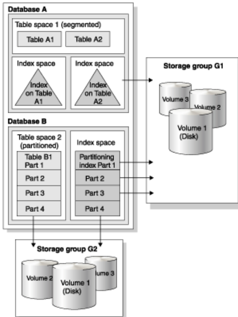
Figure 13. Hierarchy of Db2 structures
