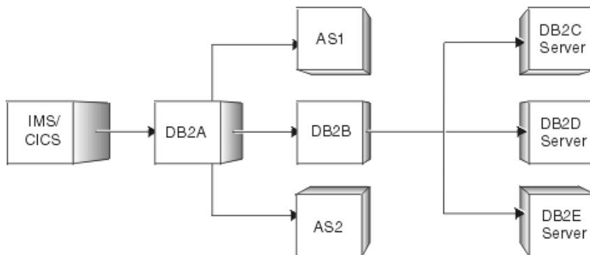
Figure 40. Illustration of multi-site unit of work
