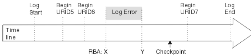
Figure 55. Illustration of failure during backward log recovery
