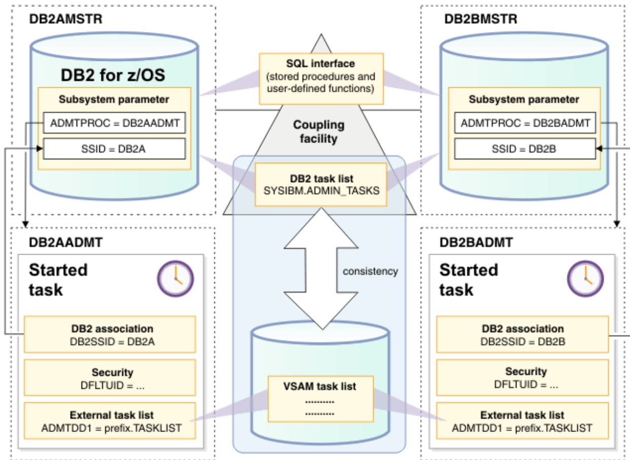
Figure 22. Administrative task schedulers in a data sharing group
