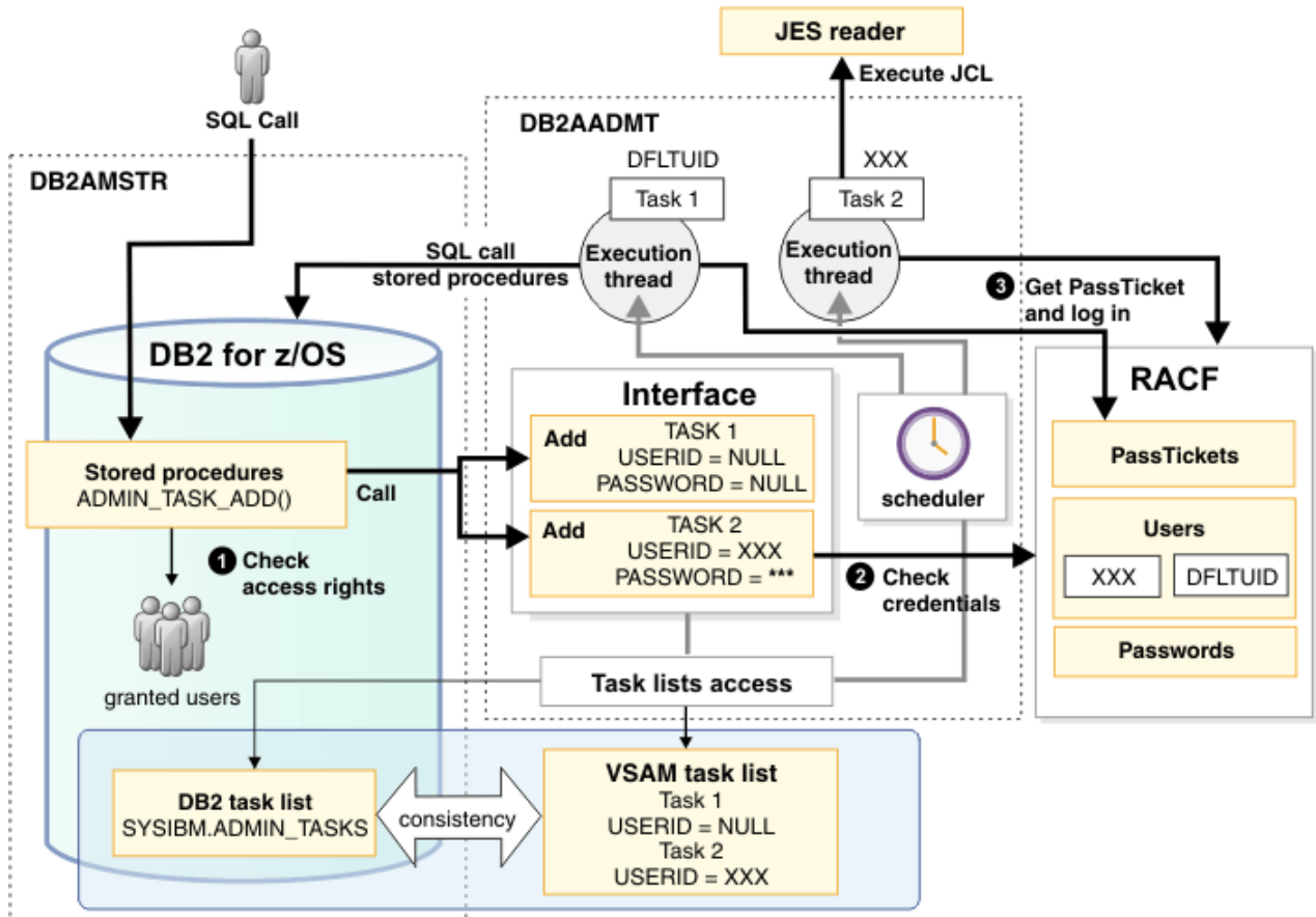
Figure 23. Security checkpoints for the administrative task scheduler
