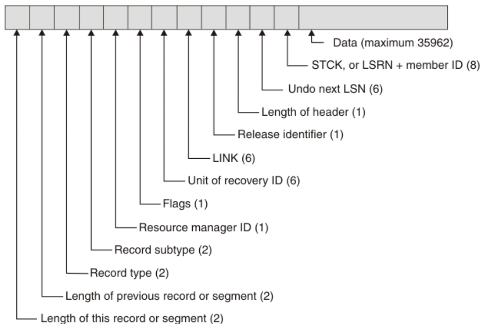
Figure 66. 6-byte format of a Db2 recovery log record
