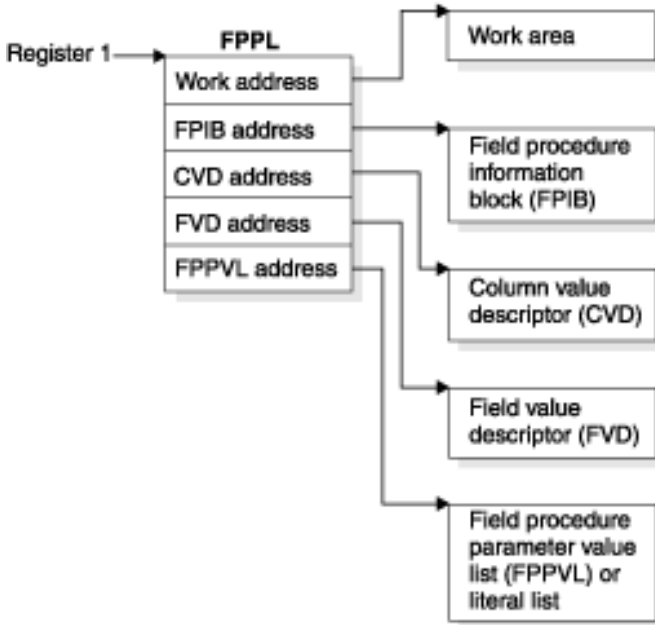
Figure 72. Field procedure parameter list
