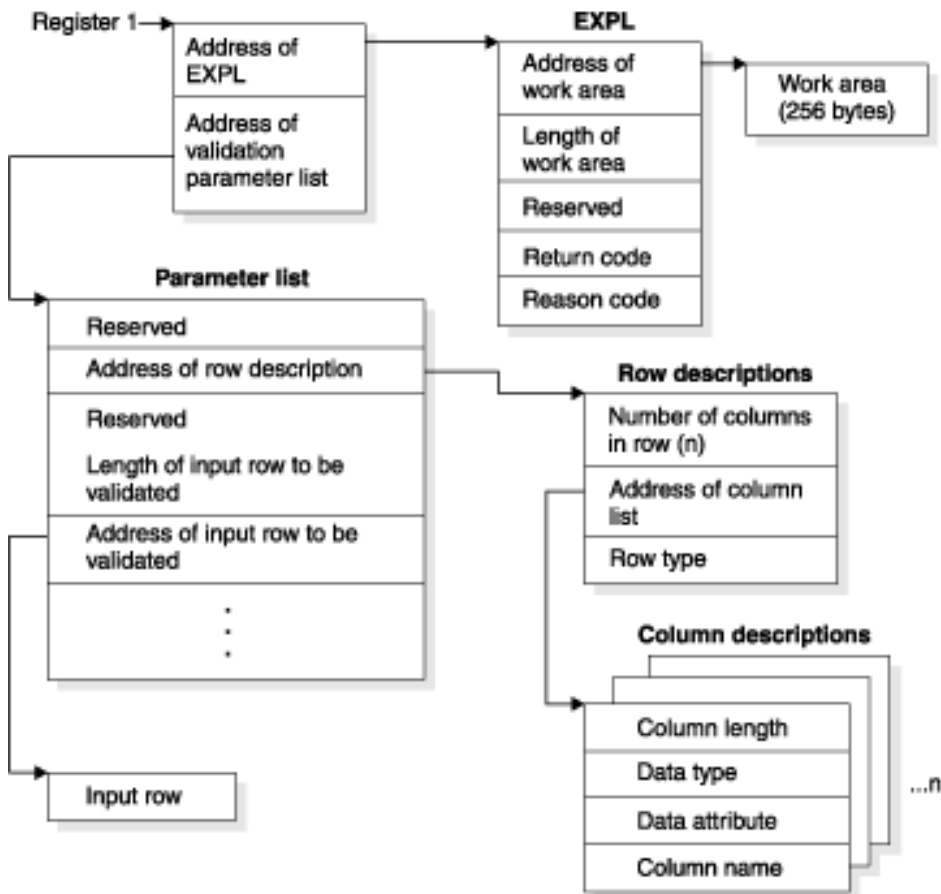
Figure 69. How a validation parameter list points to information
