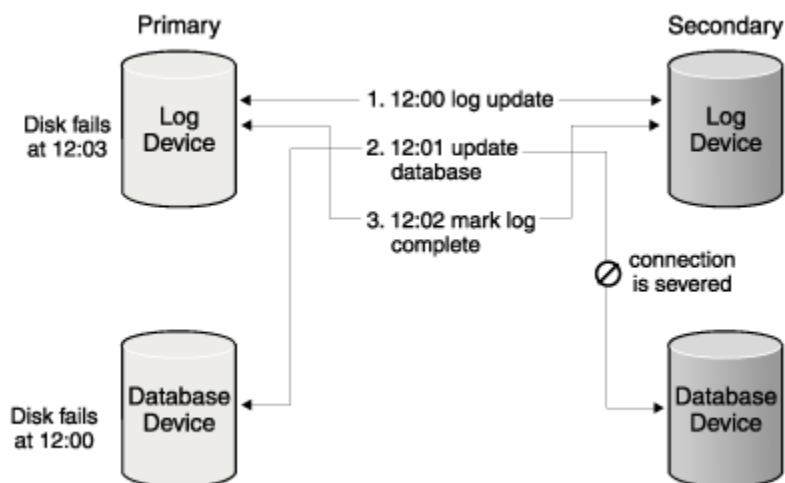
Figure 56. Data inconsistency caused by a rolling disaster
