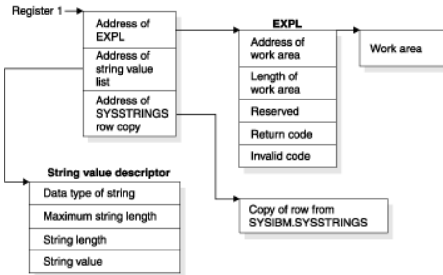
Figure 71. Pointers at entry to a conversion procedure
