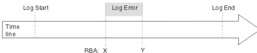
Figure 49. General problem of damaged Db2 log information
