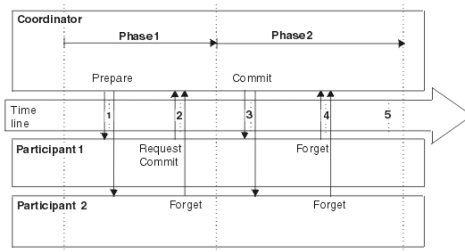
Figure 41. Illustration of multi-site update
