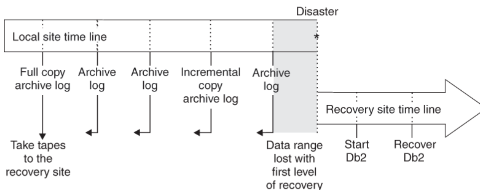
Figure 45. Preparing for disaster recovery
