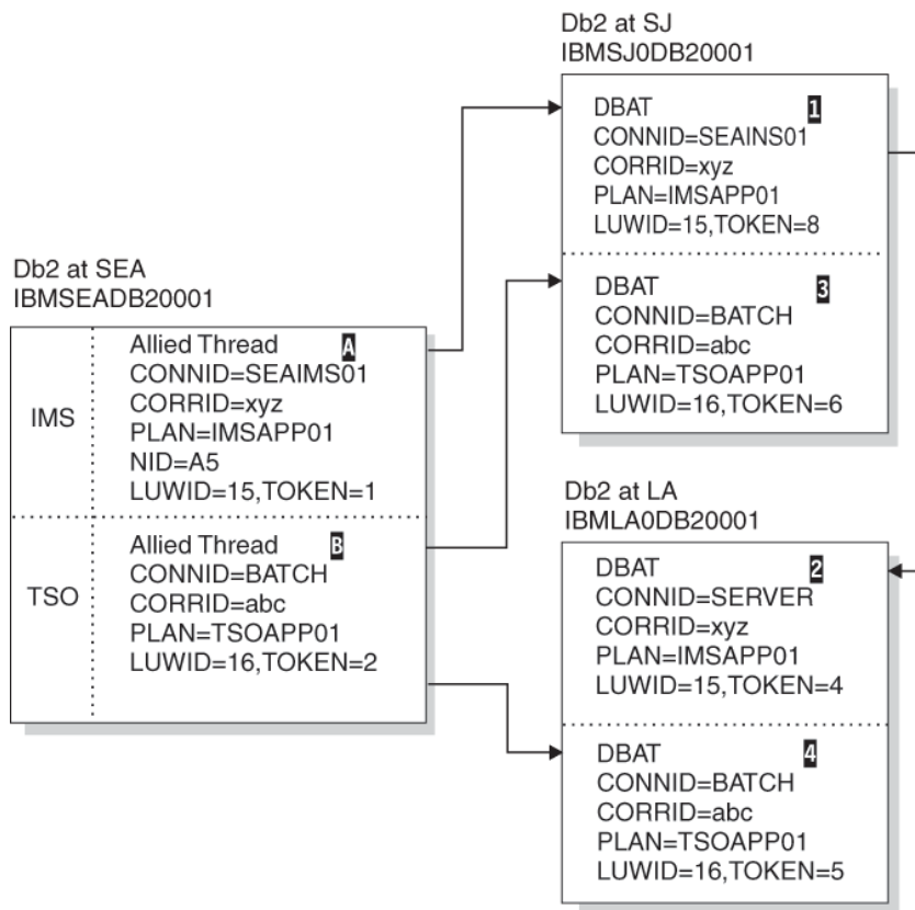
Figure 57. Resolution of indoubt threads
