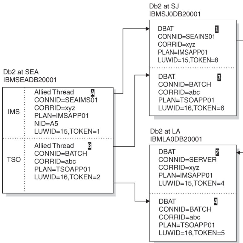
Figure 59. Resolution of indoubt threads
