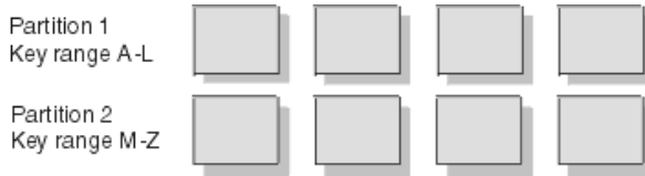
Figure 14. Pages in a range-partitioned table space
