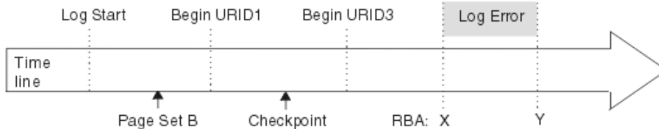
Figure 50. Failure during log initialization
