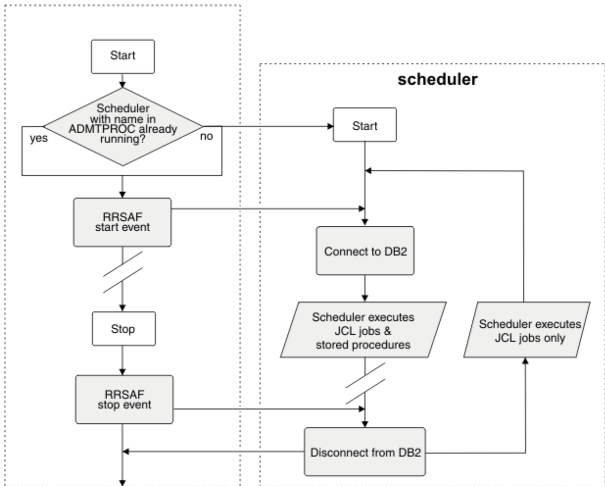
Figure 21. The lifecycle of the administrative task scheduler
