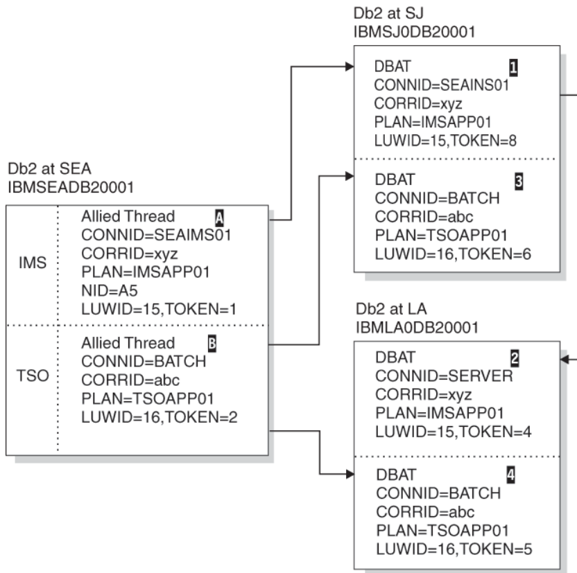
Figure 63. Resolution of indoubt threads
