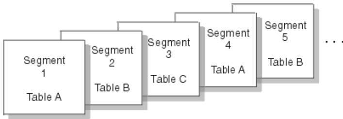
Figure 16. A possible organization of segments in a segmented table space
