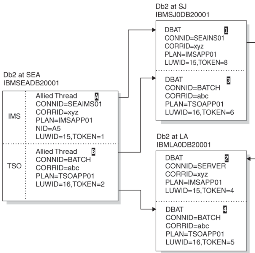
Figure 58. Resolution of indoubt threads
