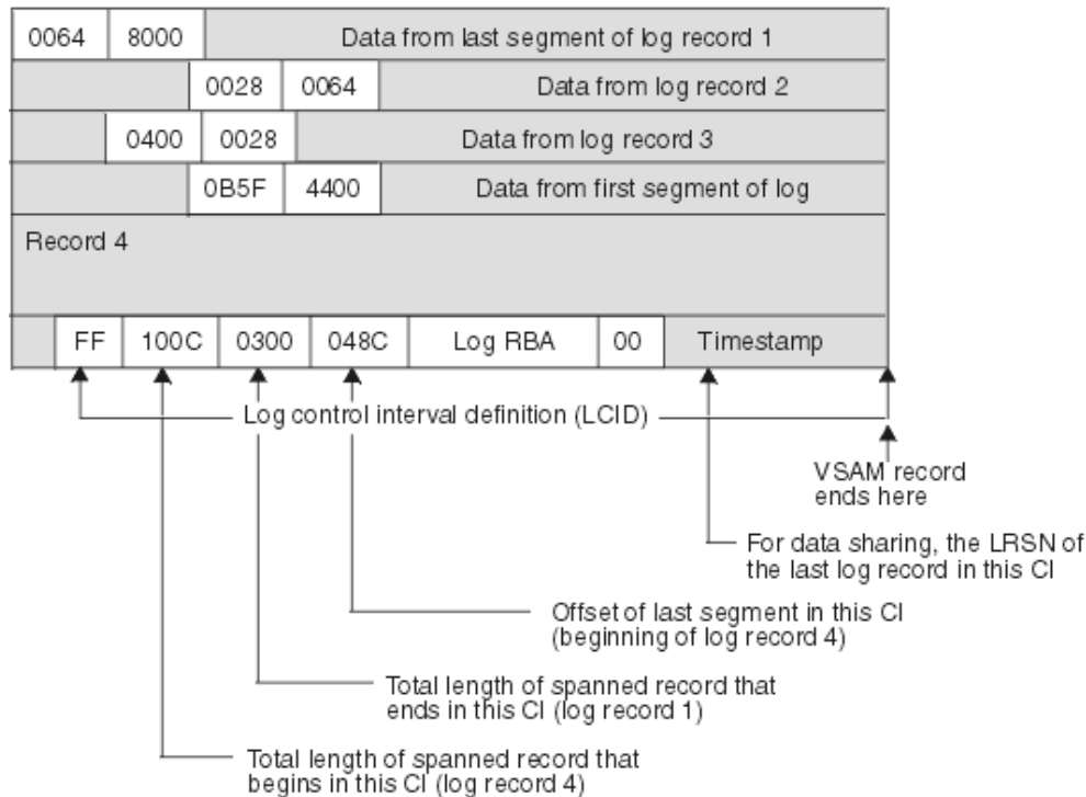
Figure 64. A VSAM CI and its contents
