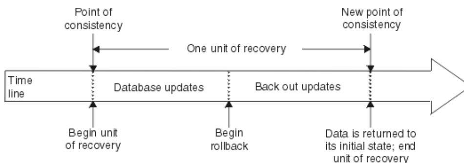
Figure 36. Unit of recovery (rolling back)
