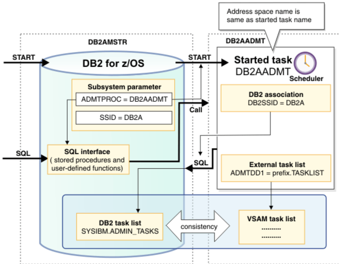
Figure 20. Architecture of the administrative task scheduler
