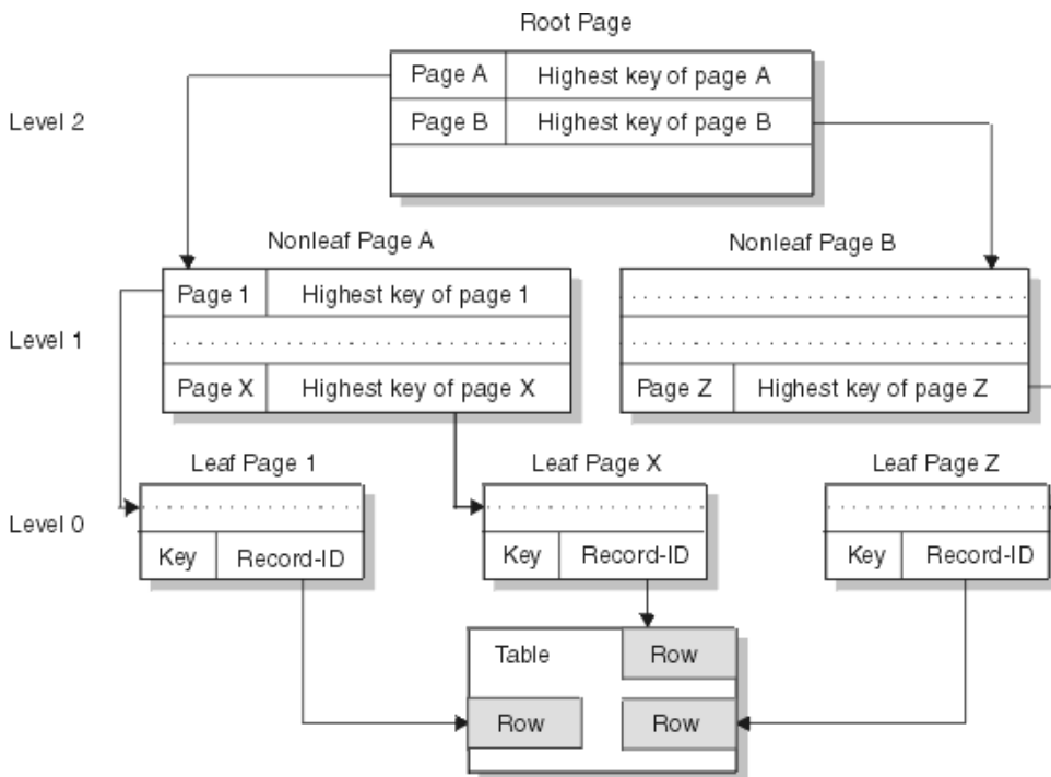
Figure 18. Sample index structure and pointers (three-level index)
