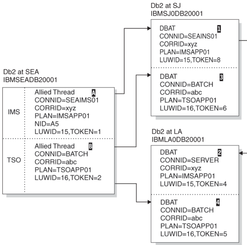
Figure 62. Resolution of indoubt threads
