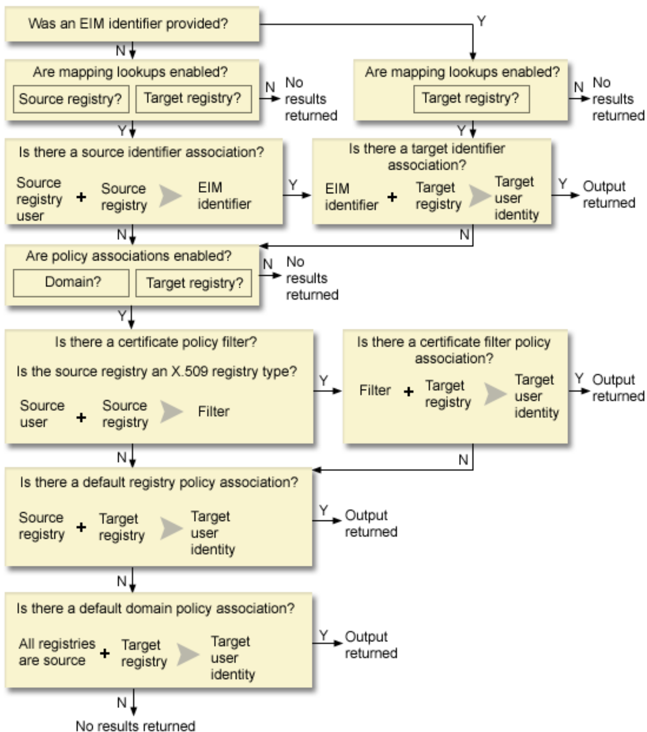
Figure 10: EIM lookup operation general processing flow chart
