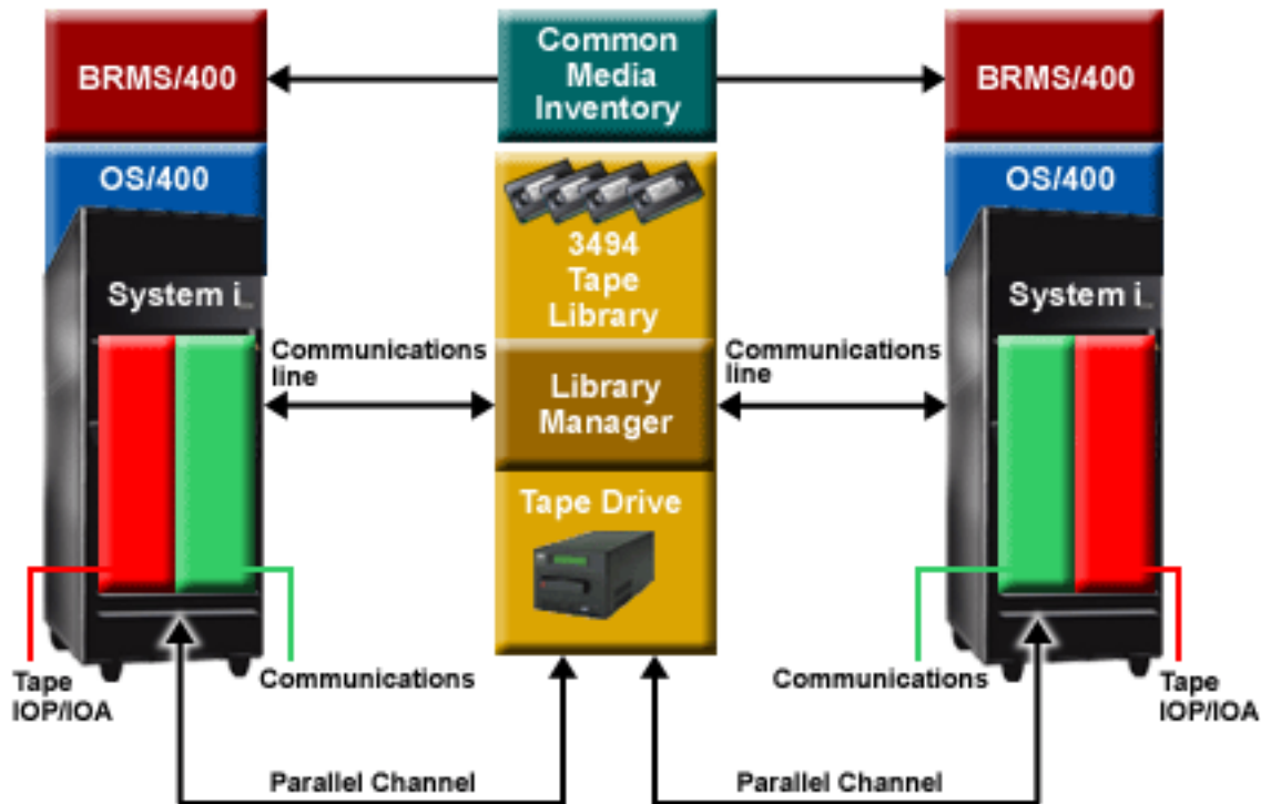
Figure 5. Servers sharing a 3494 tape library
