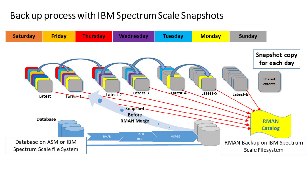
Figure 6-1 Proposed backup architecture
