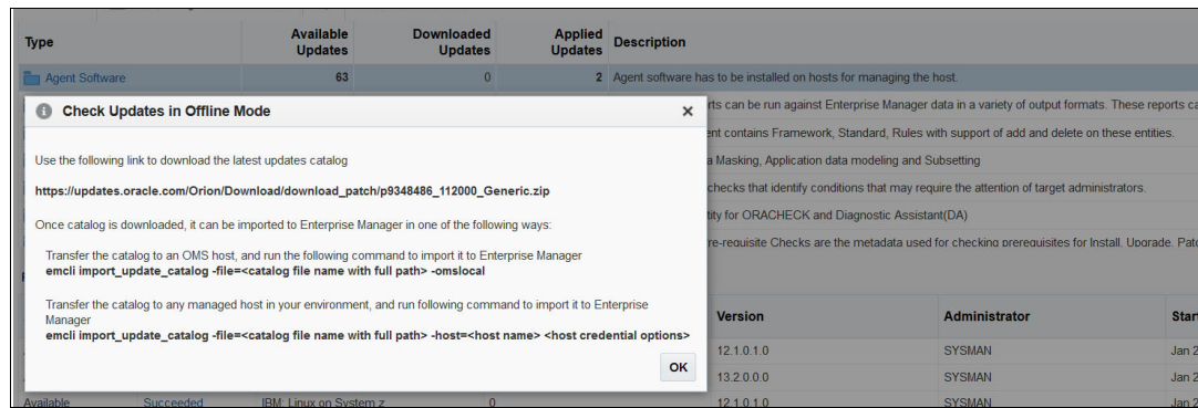
Figure 4-2 Check updates in offline mode
