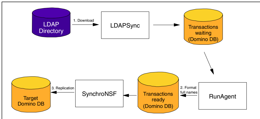
Figure 3-48 LDAPSync processing
