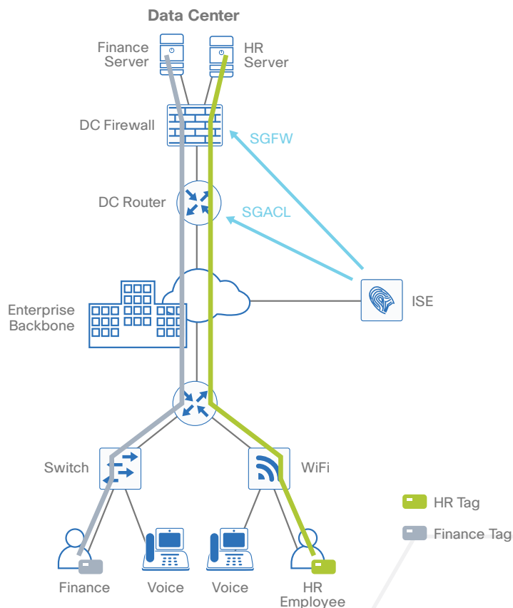
Figure 6 TrustSec for line-of-business access control
