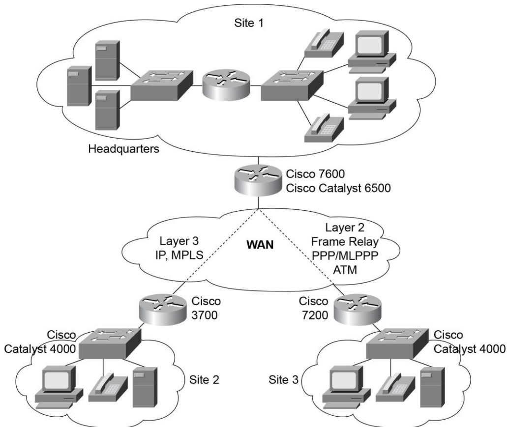
Figure 2. WAN Aggregation
