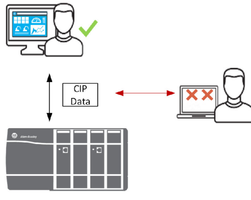
Figure 1 Reconnaissance Attack
