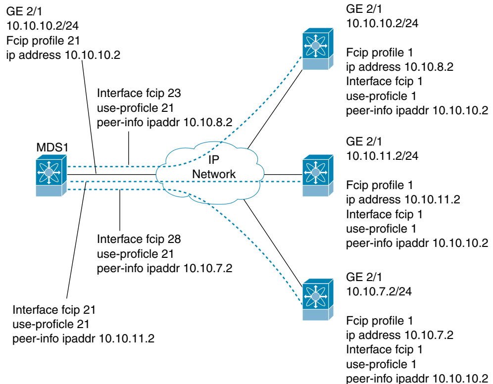
Figure 10-6 MDS1 Configured for Three FCIP Tunnels
