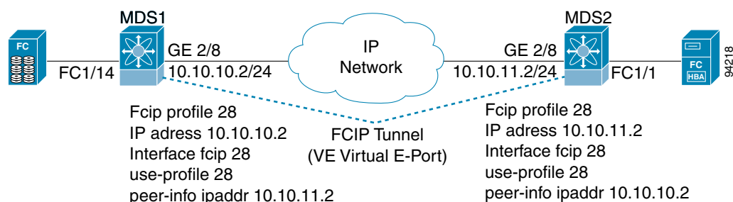
Figure 10-1 Connecting MDS 9000 Family Switches Over IP
