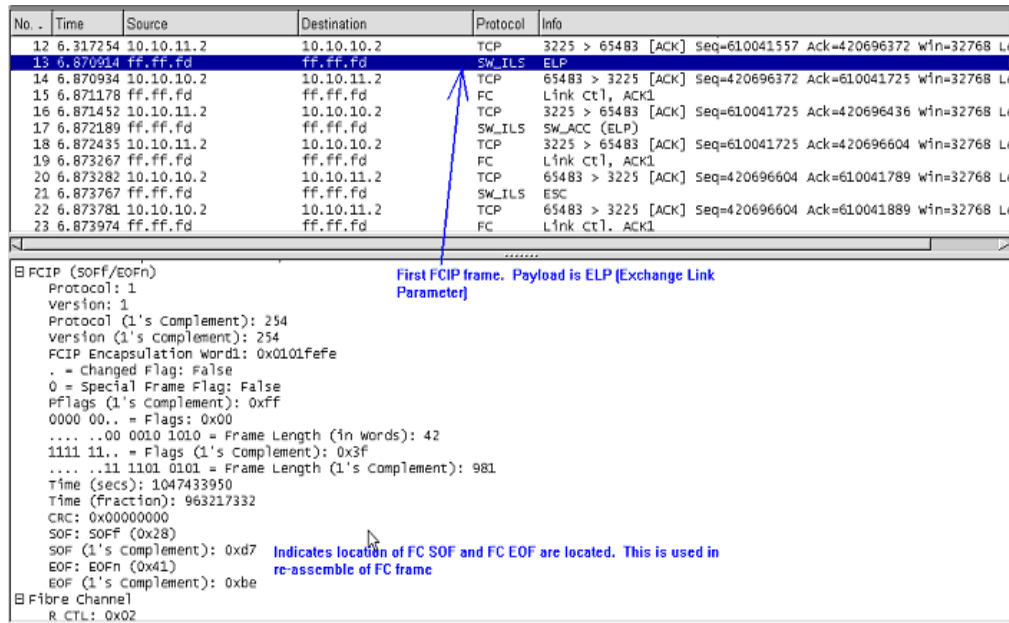
Figure 10-5 shows the FC portion of the EISL initialization over the FCIP tunnel.
