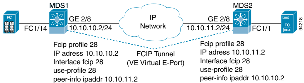
Figure 10-2 One-to-One Topology
