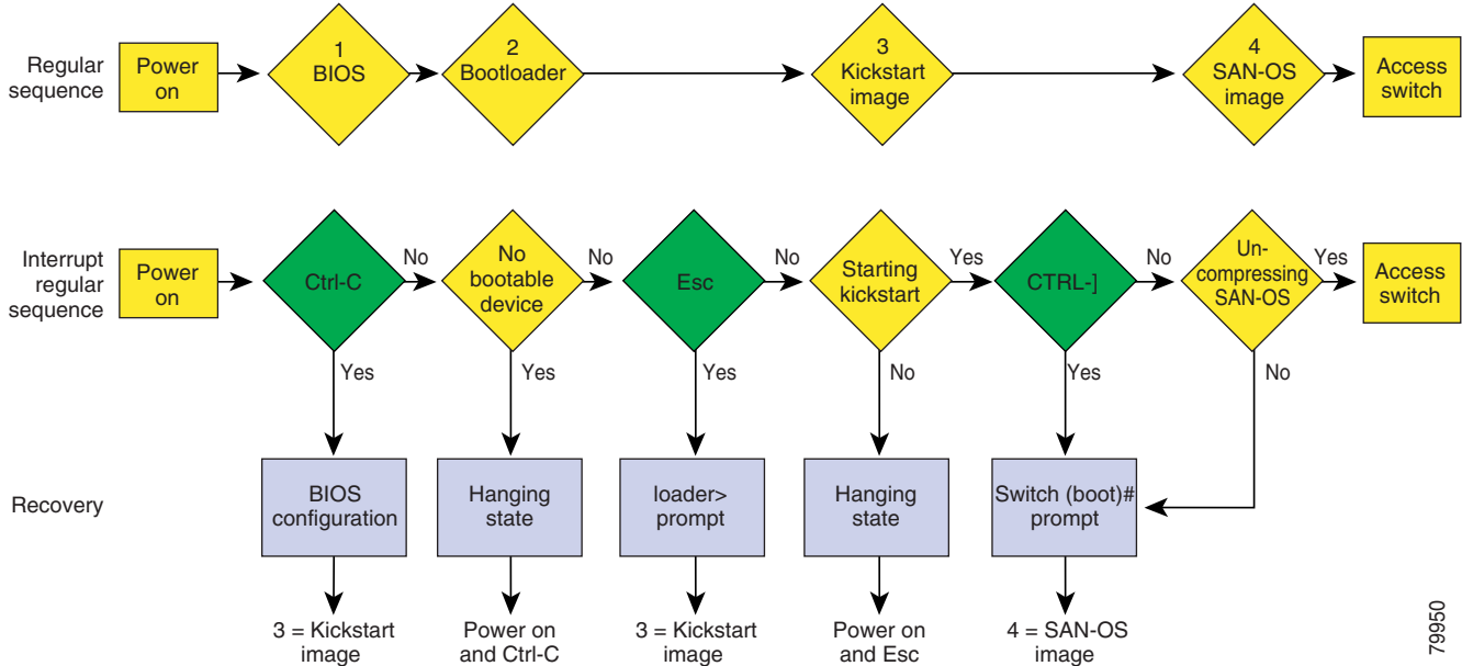
Figure 2-3 Regular and Recovery Sequence
