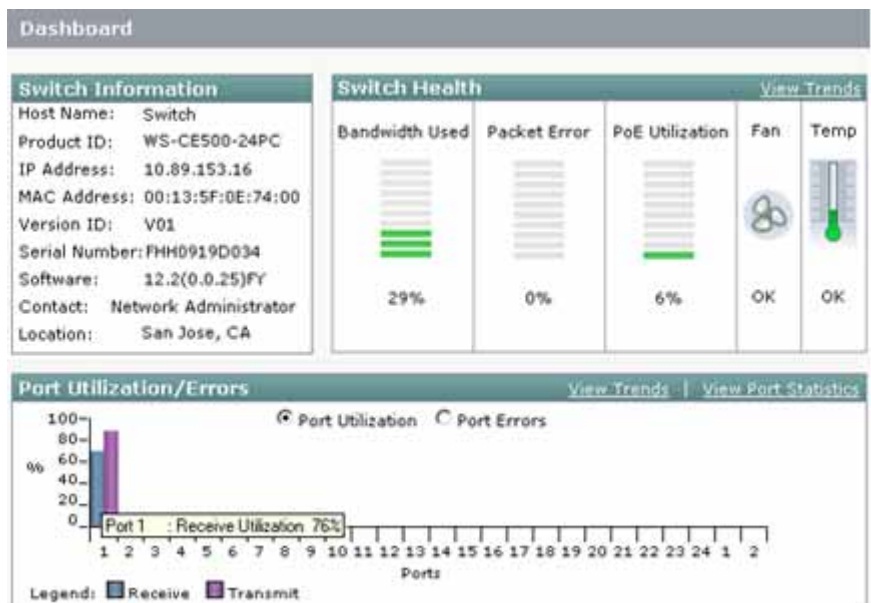
Figure 4-4 Switch Dashboard
