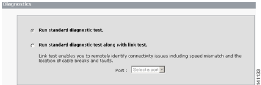
Figure 5-1 Diagnostics Window
