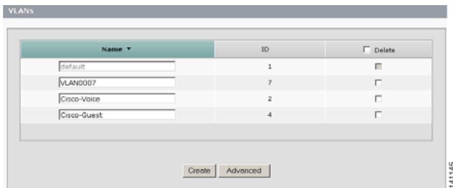
Figure 3-7 VLANs Window
