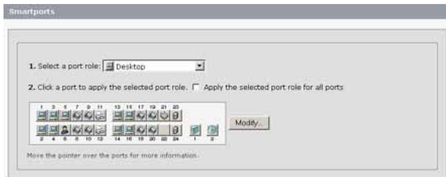
Figure 3-2 Smartports Window
